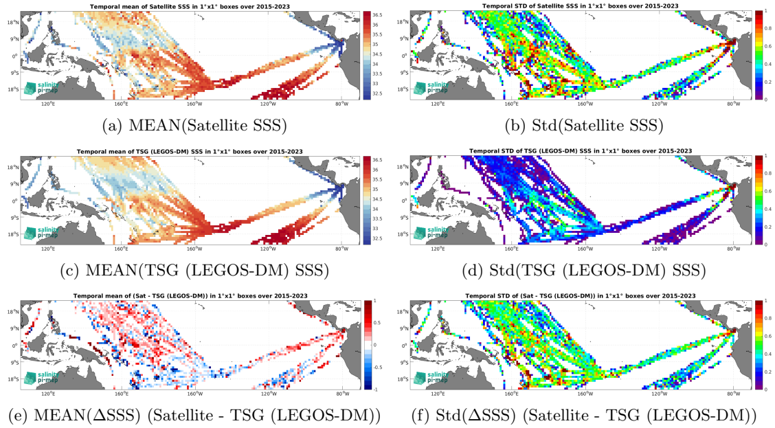
Figure 7: Temporal mean (left) and Std (right) of SSS from SMAP SSS L2 v5.0 (JPL) (top), TSG (LEGOS-DM) (middle), and of \Delta SSS (Satellite - TSG (LEGOS-DM)). Only match-up pairs are used to generate these maps.
