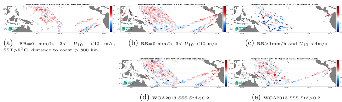
Figure 14: Temporal mean gridded over spatial boxes of size 1^\circ \times 1^\circ of \Delta SSS (SMAP SSS L2 v5.0 (JPL) - TSG (LEGOS-DM)) for 5 different subdatasets corresponding to:RR=0 mm/h, 3 < U_{10} < 12 m/s, SST > 5^\circ\text{C} , distance to coast > 800 km (a), RR=0 mm/h, 3 < U_{10} < 12 m/s (b), RR > 1 mm/h and U_{10} < 4 m/s (c), WOA2013 SSS Std < 0.2 (d), WOA2013 SSS Std > 0.2 (e).
