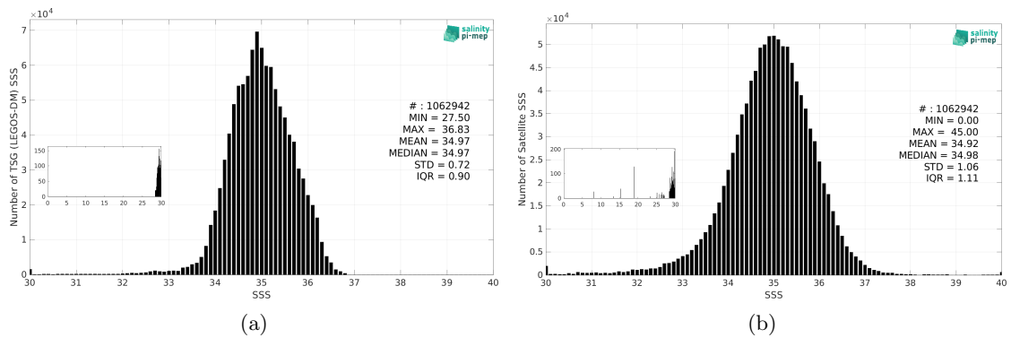
Figure 3: Histograms of SSS from TSG (LEGOS-DM) (a) and SMAP SSS L2 v5.0 (JPL) (b) considering all match-up pairs per bins of 0.1 over the Tropical Pacific Ocean Pi-MEP region and for the full satellite product period.
