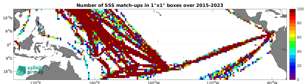
Figure 5: Number of SSS match-ups between TSG (LEGOS-DM) SSS and the SMAP SSS L2 v5.0 (JPL) SSS product for the Tropical Pacific Ocean Pi-MEP region over 1^\circ \times 1^\circ boxes and for the full satellite product period.
