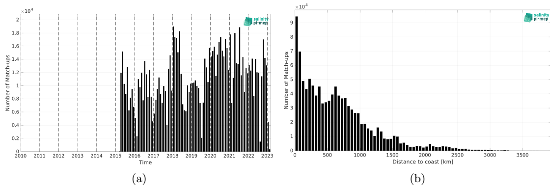
Figure 2: Number of match-ups between TSG (LEGOS-DM) and SMAP SSS L2 v5.0 (JPL) SSS as a function of time (a) and as function of the distance to coast (b) over the Tropical Pacific Ocean Pi-MEP region and for the full satellite product period.
