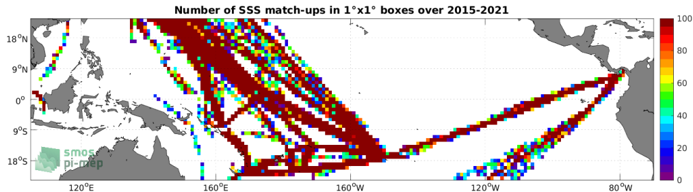
Figure 4: Number of SSS match-ups between TSG (LEGOS-DM) SSS and the SMAP SSS L2 v5.0 (JPL) SSS product for the Tropical Pacific Ocean Pi-MEP region over 1^\circ \times 1^\circ boxes and for the full satellite product period.
