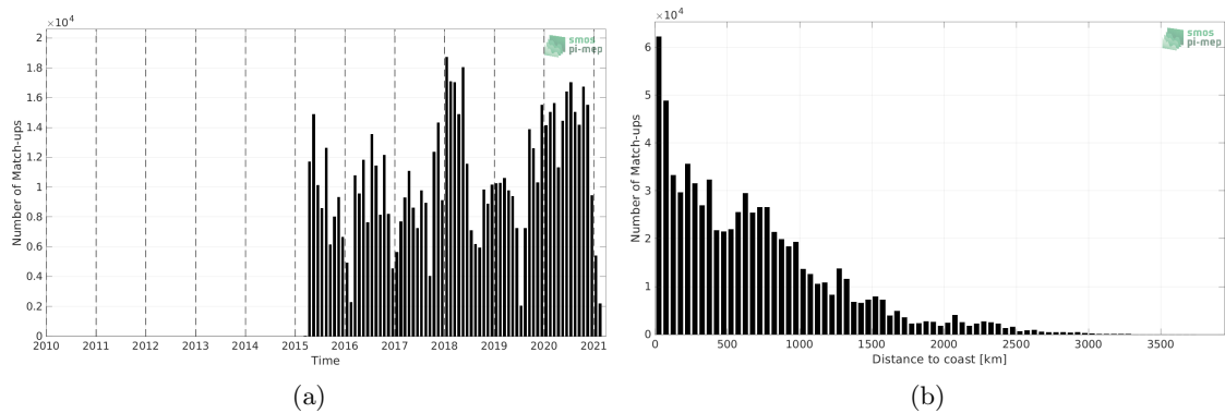
Figure 1: Number of match-ups between TSG (LEGOS-DM) and SMAP SSS L2 v5.0 (JPL) SSS as a function of time (a) and as function of the distance to coast (b) over the Tropical Pacific Ocean Pi-MEP region and for the full satellite product period.
