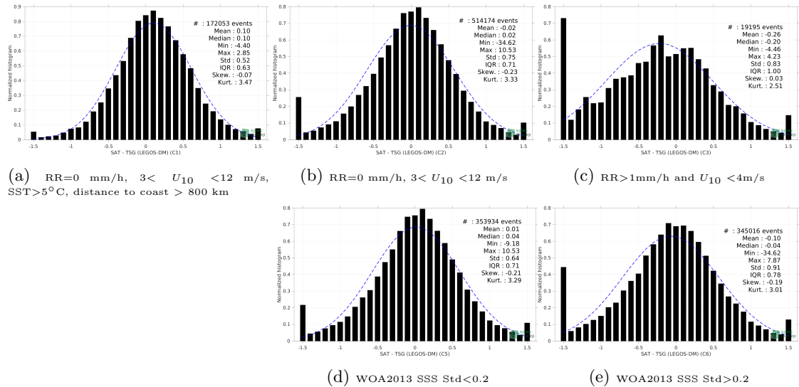
Figure 13: Normalized histogram of \Delta SSS (SMAP SSS L2 v5.0 (JPL) - TSG (LEGOS-DM)) for 5 different subdatasets corresponding to: RR=0 mm/h, 3 < U_{10} < 12 m/s, SST > 5^\circ C , distance to coast > 800 km (a), RR=0 mm/h, 3 < U_{10} < 12 m/s (b), RR>1mm/h and U_{10} < 4 m/s (c), WOA2013 SSS Std<0.2 (d), WOA2013 SSS Std>0.2 (e).
