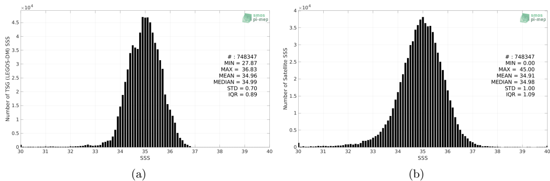
Figure 2: Histograms of SSS from TSG (LEGOS-DM) (a) and SMAP SSS L2 v5.0 (JPL) (b) considering all match-up pairs per bins of 0.1 over the Tropical Pacific Ocean Pi-MEP region and for the full satellite product period.
