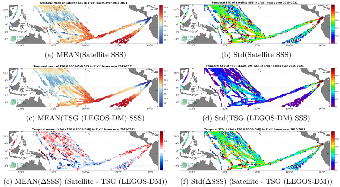
Figure 6: Temporal mean (left) and Std (right) of SSS from SMAP SSS L2 v5.0 (JPL) (top), TSG (LEGOS-DM) (middle), and of \Delta SSS (Satellite - TSG (LEGOS-DM)). Only match-up pairs are used to generate these maps.
