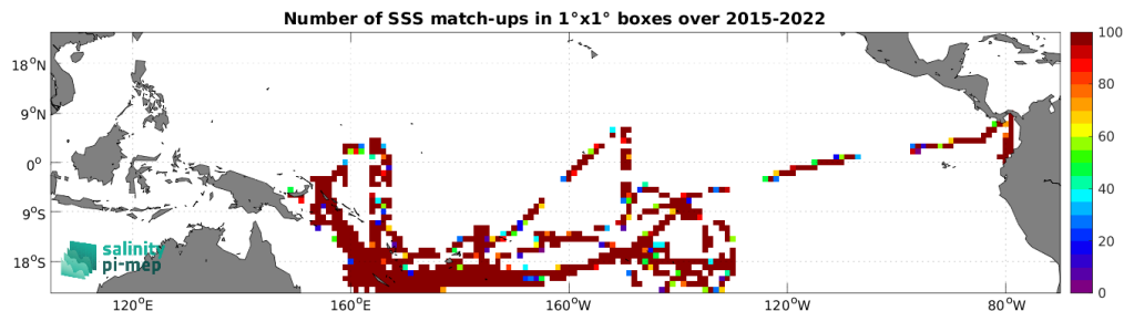
Figure 5: Number of SSS match-ups between TSG (GOSUD-Research-vessel) SSS and the SMAP SSS L2 v5.0 (JPL) SSS product for the Tropical Pacific Ocean Pi-MEP region over 1^\circ \times 1^\circ boxes and for the full satellite product period.
