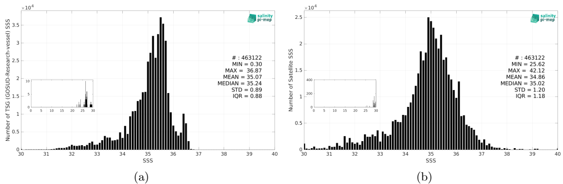
Figure 3: Histograms of SSS from TSG (GOSUD-Research-vessel) (a) and SMAP SSS L2 v5.0 (JPL) (b) considering all match-up pairs per bins of 0.1 over the Tropical Pacific Ocean Pi-MEP region and for the full satellite product period.
