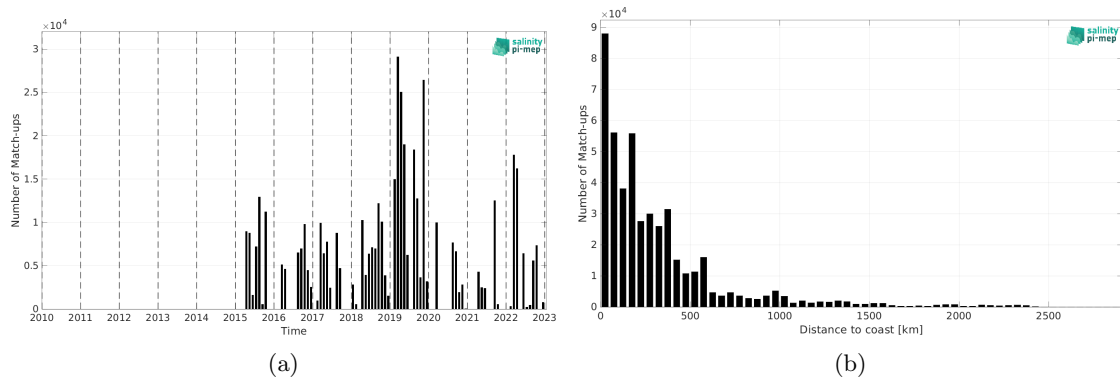
Figure 2: Number of match-ups between TSG (GOSUD-Research-vessel) and SMAP SSS L2 v5.0 (JPL) SSS as a function of time (a) and as function of the distance to coast (b) over the Tropical Pacific Ocean Pi-MEP region and for the full satellite product period.
