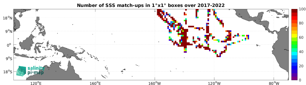
Figure 5: Number of SSS match-ups between Saildrone SSS and the SMAP SSS L2 v5.0 (JPL) SSS product for the Tropical Pacific Ocean Pi-MEP region over 1^\circ \times 1^\circ boxes and for the full satellite product period.
