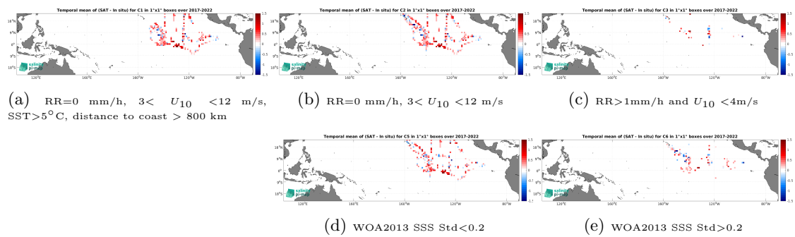
Figure 14: Temporal mean gridded over spatial boxes of size 1^\circ \times 1^\circ of \Delta SSS (SMAP SSS L2 v5.0 (JPL) - Sairdrone) for 5 different subdatasets corresponding to:RR=0 mm/h, 3 < U_{10} < 12 m/s, SST > 5^\circ\text{C} , distance to coast > 800 km (a), RR=0 mm/h, 3 < U_{10} < 12 m/s (b), RR > 1 mm/h and U_{10} < 4 m/s (c), WOA2013 SSS Std < 0.2 (d), WOA2013 SSS Std > 0.2 (e).
