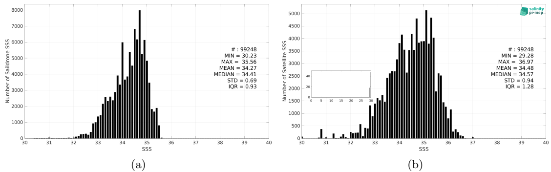
Figure 3: Histograms of SSS from Saildrone (a) and SMAP SSS L2 v5.0 (JPL) (b) considering all match-up pairs per bins of 0.1 over the Tropical Pacific Ocean Pi-MEP region and for the full satellite product period.
