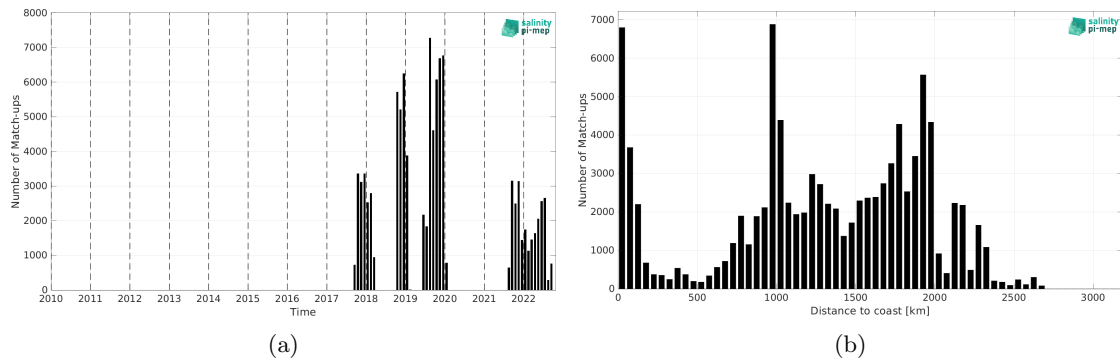
Figure 2: Number of match-ups between Saildrone and SMAP SSS L2 v5.0 (JPL) SSS as a function of time (a) and as function of the distance to coast (b) over the Tropical Pacific Ocean Pi-MEP region and for the full satellite product period.
