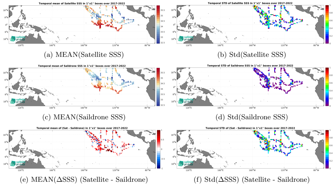
Figure 7: Temporal mean (left) and Std (right) of SSS from SMAP SSS L2 v5.0 (JPL) (top), Saildrone (middle), and of \Delta SSS (Satellite - Saildrone). Only match-up pairs are used to generate these maps.
