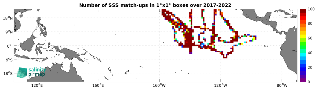
Figure 4: Number of SSS match-ups between Saildrone SSS and the SMAP SSS L2 v5.0 (JPL) SSS product for the Tropical Pacific Ocean Pi-MEP region over 1^\circ \times 1^\circ boxes and for the full satellite product period.
