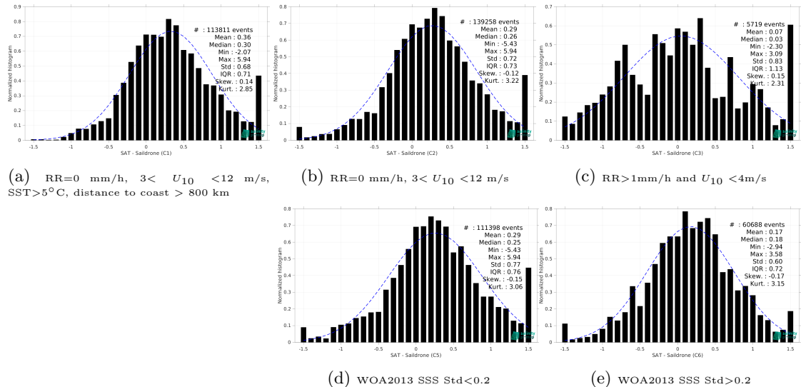
Figure 13: Normalized histogram of \Delta SSS (SMAP SSS L2 v5.0 (JPL) - Saildrone) for 5 different subdatasets corresponding to: RR=0 mm/h, 3 < U_{10} < 12 m/s, SST >5^\circ C, distance to coast > 800 km (a), RR=0 mm/h, 3 < U_{10} < 12 m/s (b), RR >1 mm/h and U_{10} < 4 m/s (c), WOA2013 SSS Std <0.2 (d), WOA2013 SSS Std >0.2 (e).
