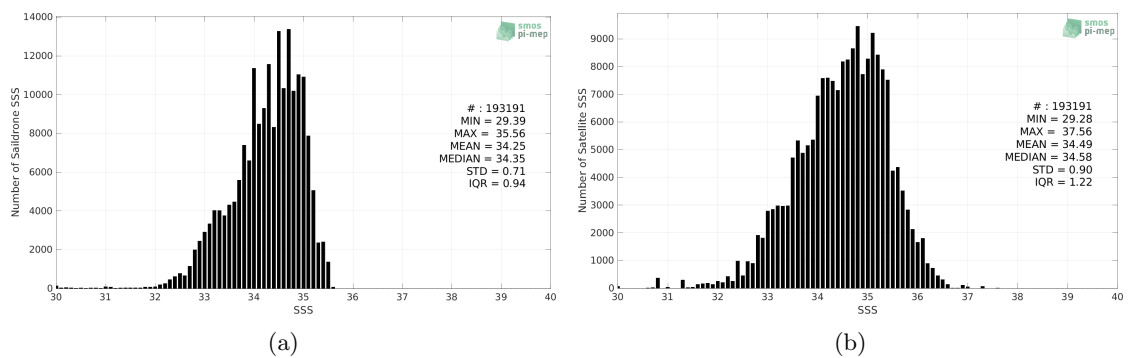
Figure 2: Histograms of SSS from Saildrone (a) and SMAP SSS L2 v5.0 (JPL) (b) considering all match-up pairs per bins of 0.1 over the Tropical Pacific Ocean Pi-MEP region and for the full satellite product period.
