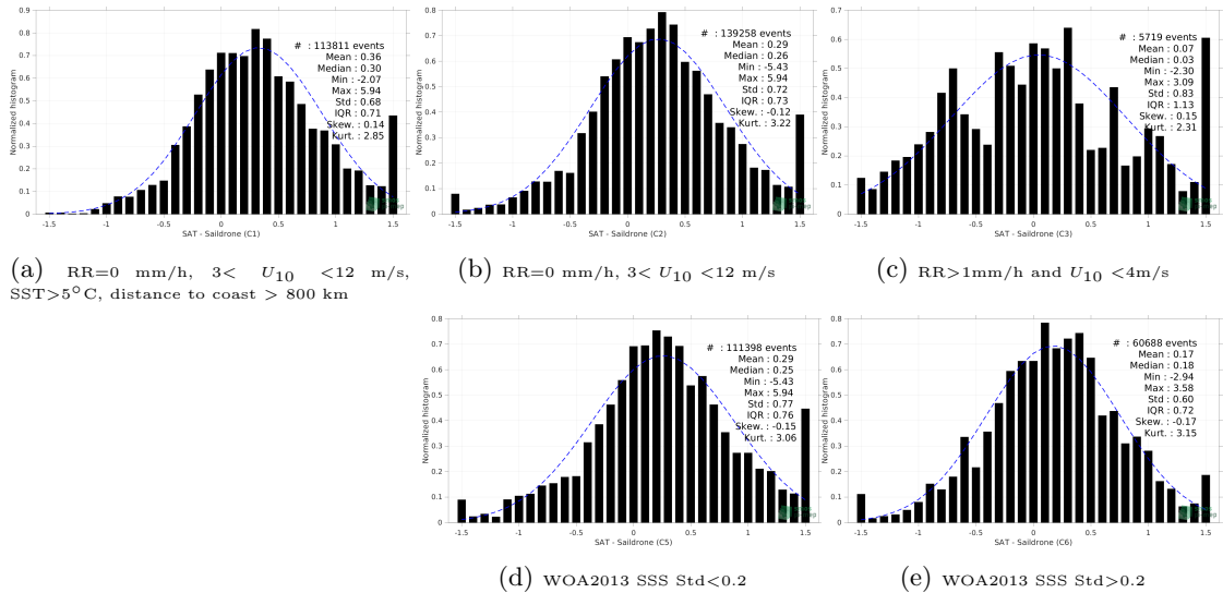
Figure 13: Normalized histogram of \Delta SSS (SMAP SSS L2 v5.0 (JPL) - Saildrone) for 5 different subdatasets corresponding to: RR=0 mm/h, 3 < U_{10} < 12 m/s, SST>5°C, distance to coast > 800 km (a), RR=0 mm/h, 3 < U_{10} < 12 m/s (b), RR>1mm/h and U_{10} < 4 m/s (c), WOA2013 SSS Std<0.2 (d), WOA2013 SSS Std>0.2 (e).
