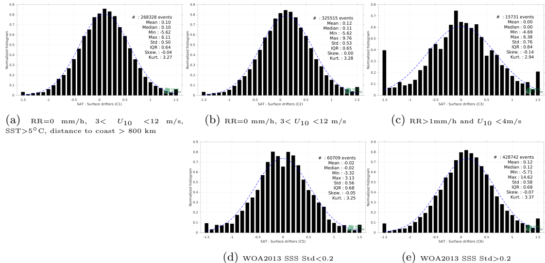
Figure 12: Normalized histogram of \Delta SSS (SMAP SSS L2 v5.0 (JPL) - Surface drifters) for 5 different subdatasets corresponding to: RR=0 mm/h, 3 < U_{10} < 12 m/s, SST >5^\circ C, distance to coast > 800 km (a), RR=0 mm/h, 3 < U_{10} < 12 m/s (b), RR >1 mm/h and U_{10} < 4 m/s (c), WOA2013 SSS Std <0.2 (d), WOA2013 SSS Std >0.2 (e).
