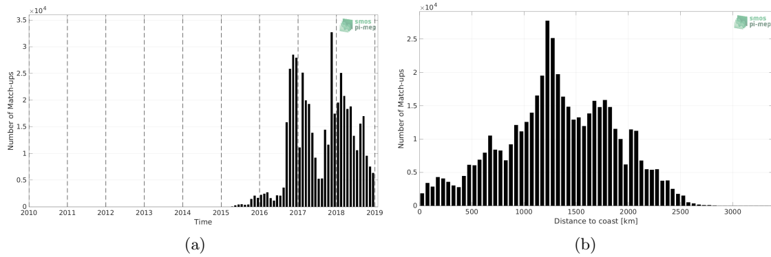
Figure 1: Number of match-ups between Surface drifters and SMAP SSS L2 v5.0 (JPL) SSS as a function of time (a) and as function of the distance to coast (b) over the Tropical Pacific Ocean Pi-MEP region and for the full satellite product period.
