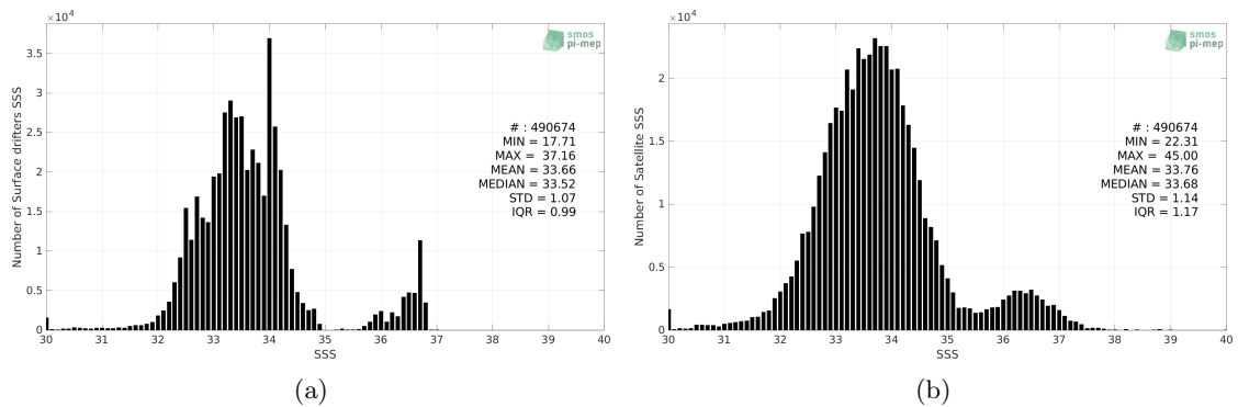
Figure 2: Histograms of SSS from Surface drifters (a) and SMAP SSS L2 v5.0 (JPL) (b) considering all match-up pairs per bins of 0.1 over the Tropical Pacific Ocean Pi-MEP region and for the full satellite product period.
