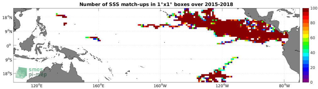
Figure 3: Number of SSS match-ups between Surface drifters SSS and the SMAP SSS L2 v5.0 (JPL) SSS product for the Tropical Pacific Ocean Pi-MEP region over 1^\circ \times 1^\circ boxes and for the full satellite product period.
