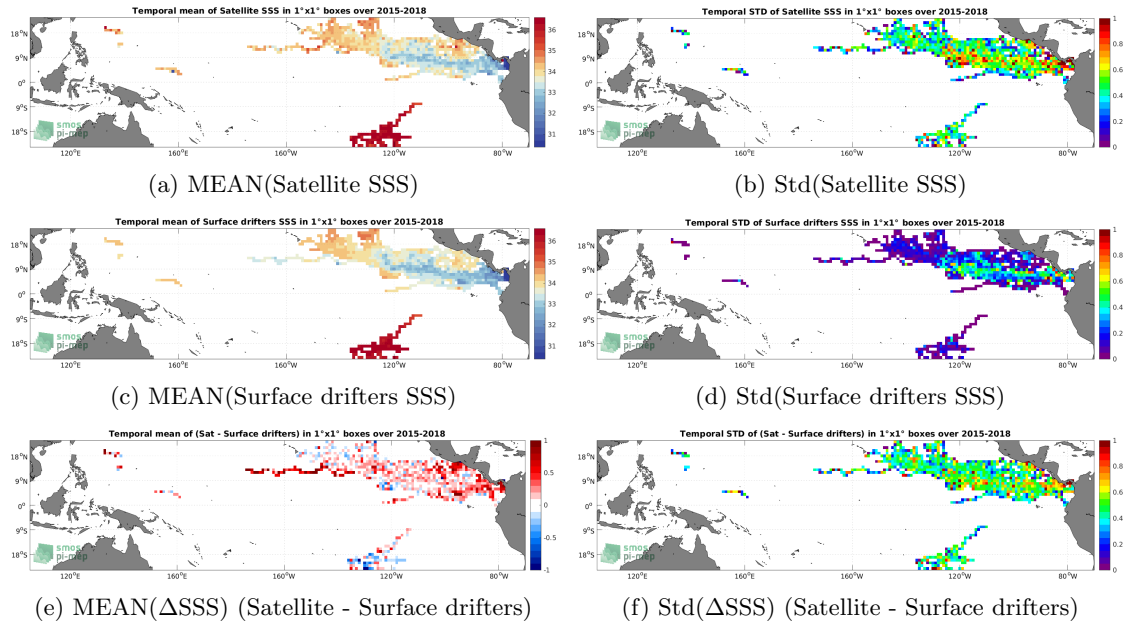
Figure 5: Temporal mean (left) and Std (right) of SSS from SMAP SSS L2 v5.0 (JPL) (top), Surface drifters (middle), and of \Delta SSS (Satellite - Surface drifters). Only match-up pairs are used to generate these maps.
