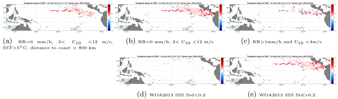
Figure 11: Temporal mean gridded over spatial boxes of size 1°x1° of ΔSSS (SMAP SSS L2 v5.0 (JPL) - Surface drifters) for 5 different subdatasets corresponding to:RR=0 mm/h, 3 < U 10 < 12 m/s, SST>5°C, distance to coast > 800 km (a), RR=0 mm/h, 3 < U 10 < 12 m/s (b), RR>1mm/h and U 10 <4m/s (c), WOA2013 SSS Std<0.2 (d), WOA2013 SSS Std>0.2 (e).
