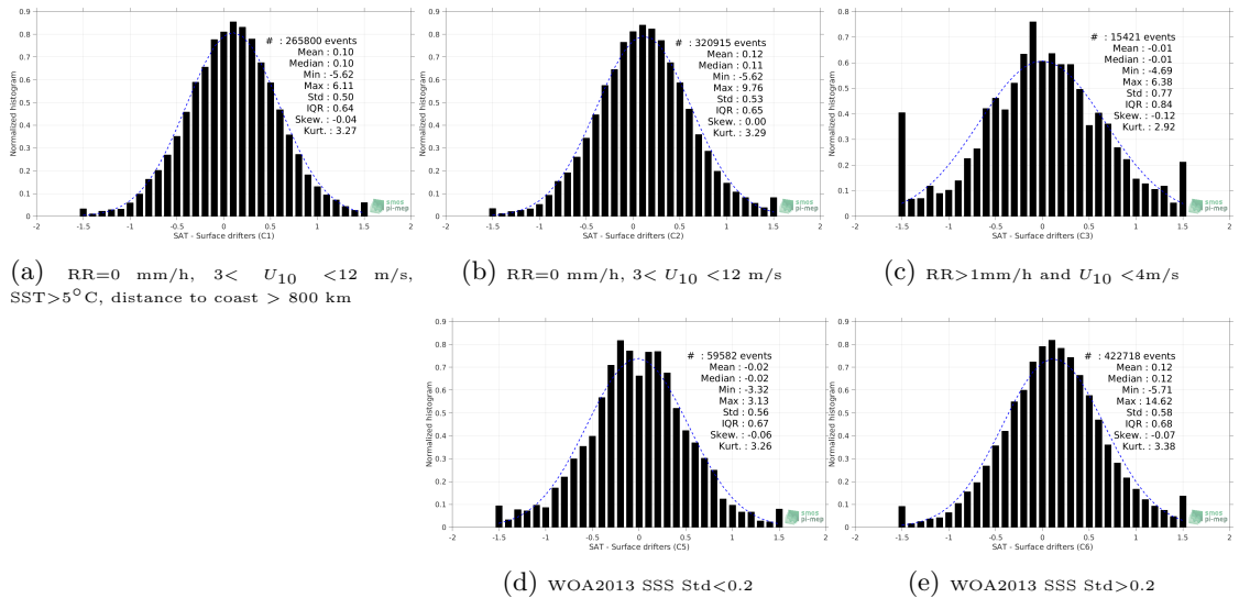
Figure 12: Normalized histogram of ΔSSS (SMAP SSS L2 v5.0 (JPL) - Surface drifters) for 5 different subdatasets corresponding to: RR=0 mm/h, 3 < U 10 < 12 m/s, SST>5°C, distance to coast > 800 km (a), RR=0 mm/h, 3 < U 10 < 12 m/s (b), RR>1mm/h and U 10 <4m/s (c), WOA2013 SSS Std<0.2 (d), WOA2013 SSS Std>0.2 (e).
