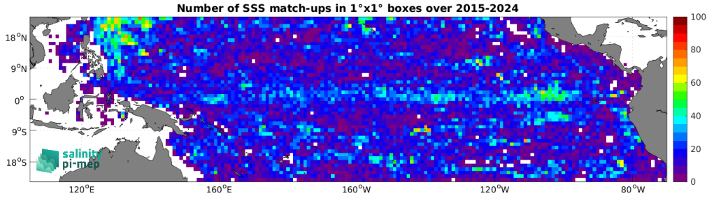
Figure 5: Number of SSS match-ups between Argo SSS and the SMAP SSS L2 v5.0 (JPL) SSS product for the Tropical Pacific Ocean Pi-MEP region over 1^\circ \times 1^\circ boxes and for the full satellite product period.
