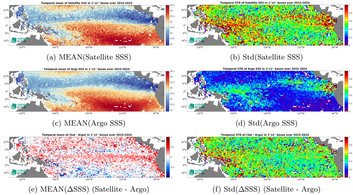
Figure 7: Temporal mean (left) and Std (right) of SSS from SMAP SSS L2 v5.0 (JPL) (top), Argo (middle), and of \Delta SSS (Satellite - Argo). Only match-up pairs are used to generate these maps.
