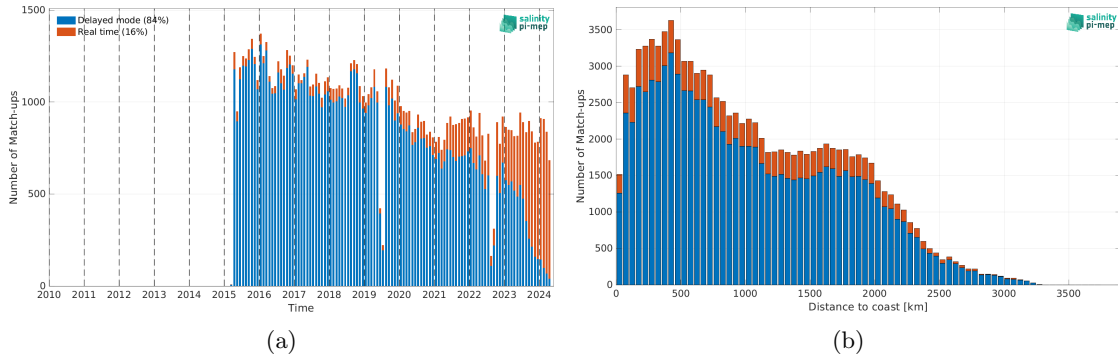
Figure 2: Number of match-ups between Argo and SMAP SSS L2 v5.0 (JPL) SSS as a function of time (a) and as function of the distance to coast (b) over the Tropical Pacific Ocean Pi-MEP region and for the full satellite product period.
