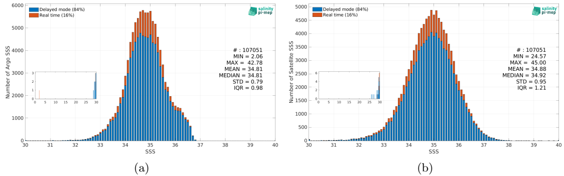
Figure 3: Histograms of SSS from Argo (a) and SMAP SSS L2 v5.0 (JPL) (b) considering all match-up pairs per bins of 0.1 over the Tropical Pacific Ocean Pi-MEP region and for the full satellite product period.
