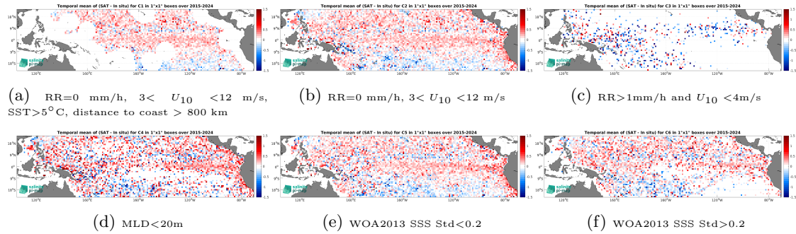
Figure 14: Temporal mean gridded over spatial boxes of size 1^\circ \times 1^\circ of \Delta SSS (SMAP SSS L2 v5.0 (JPL) - Argo) for 6 different subdatasets corresponding to:RR=0 mm/h, 3 < U_{10} < 12 m/s, SST>5°C, distance to coast > 800 km (a), RR=0 mm/h, 3 < U_{10} < 12 m/s (b), RR>1mm/h and U_{10} < 4 m/s (c),MLD<20m (d),WOA2013 SSS Std<0.2 (e),WOA2013 SSS Std>0.2 (f).
