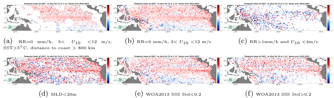
Figure 12: Temporal mean gridded over spatial boxes of size 1^\circ \times 1^\circ of \Delta SSS (SMAP SSS L2 v5.0 (JPL) - Argo) for 6 different subdatasets corresponding to:RR=0 mm/h, 3 < U_{10} < 12 m/s, SST >5^\circ C, distance to coast > 800 km (a), RR=0 mm/h, 3 < U_{10} < 12 m/s (b), RR >1 mm/h and U_{10} < 4 m/s (c),MLD <20 m (d),WOA2013 SSS Std <0.2 (e),WOA2013 SSS Std >0.2 (f).
