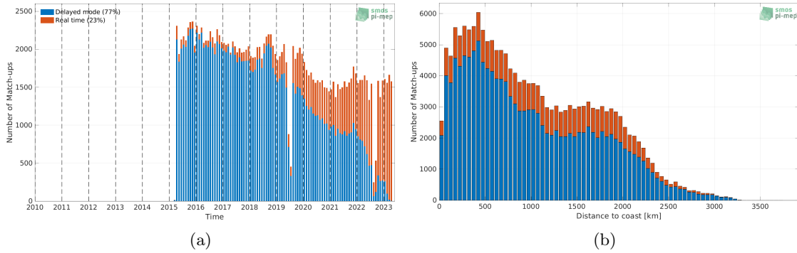
Figure 1: Number of match-ups between Argo and SMAP SSS L2 v5.0 (JPL) SSS as a function of time (a) and as function of the distance to coast (b) over the Tropical Pacific Ocean Pi-MEP region and for the full satellite product period.
