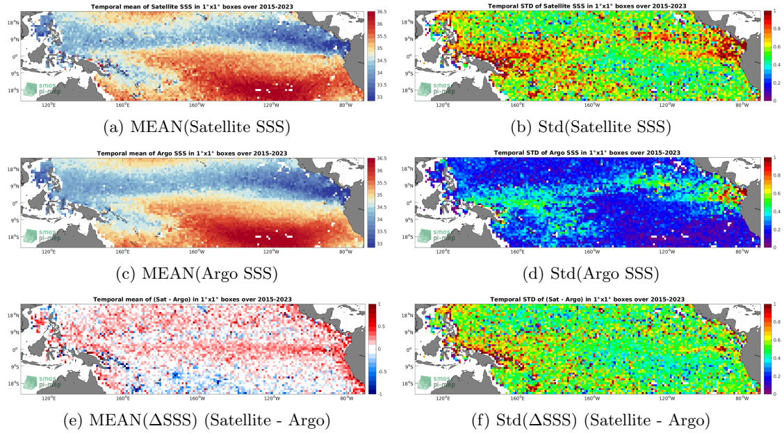
Figure 6: Temporal mean (left) and Std (right) of SSS from SMAP SSS L2 v5.0 (JPL) (top), Argo (middle), and of \Delta SSS (Satellite - Argo). Only match-up pairs are used to generate these maps.
