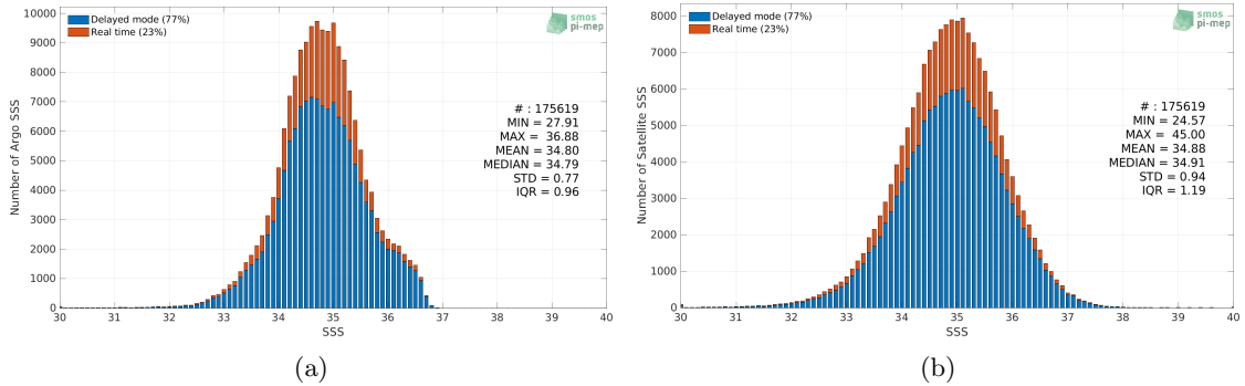
Figure 2: Histograms of SSS from Argo (a) and SMAP SSS L2 v5.0 (JPL) (b) considering all match-up pairs per bins of 0.1 over the Tropical Pacific Ocean Pi-MEP region and for the full satellite product period.
