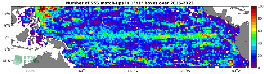
Figure 4: Number of SSS match-ups between Argo SSS and the SMAP SSS L2 v5.0 (JPL) SSS product for the Tropical Pacific Ocean Pi-MEP region over 1^\circ \times 1^\circ boxes and for the full satellite product period.
