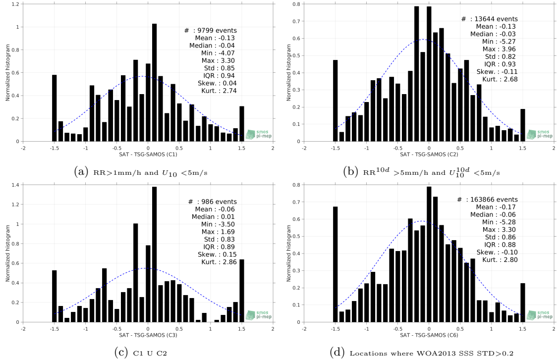
Figure 13: Normalized histogram of \Delta\text{SSS} (SMAP-L2-JPL-V4 - TSG-SAMOS) for 6 different subdatasets corresponding to: RR > 1\text{mm/h} and U_{10} < 5\text{m/s} (a), RR^{10d} > 5\text{mm/h} and U_{10}^{10d} < 5\text{m/s} (b), C1 U C2 (c), Locations where WOA2013 SSS STD > 0.2 (d).
