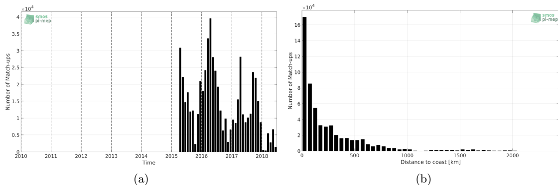
Figure 1: Number of match-ups between TSG-SAMOS and SMAP-L2-JPL-V4 SSS as a function of time (a) and as function of the distance to coast (b) over the Tropical Pacific Ocean Pi-MEP region and for the full satellite product period.
