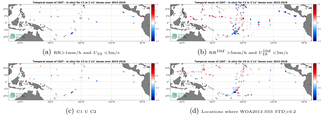
Figure 12: Temporal mean gridded over spatial boxes of size 1^\circ \times 1^\circ of \Delta SSS (SMAP-L2-JPL-V4 - TSG-SAMOS) for 4 different subdatasets corresponding to: RR > 1\text{mm/h} and U_{10} < 5\text{m/s} (a), RR^{10d} > 5\text{mm/h} and U_{10}^{10d} < 5\text{m/s} (b), C1 U C2 (c), Locations where WOA2013 SSS STD > 0.2 (d).
