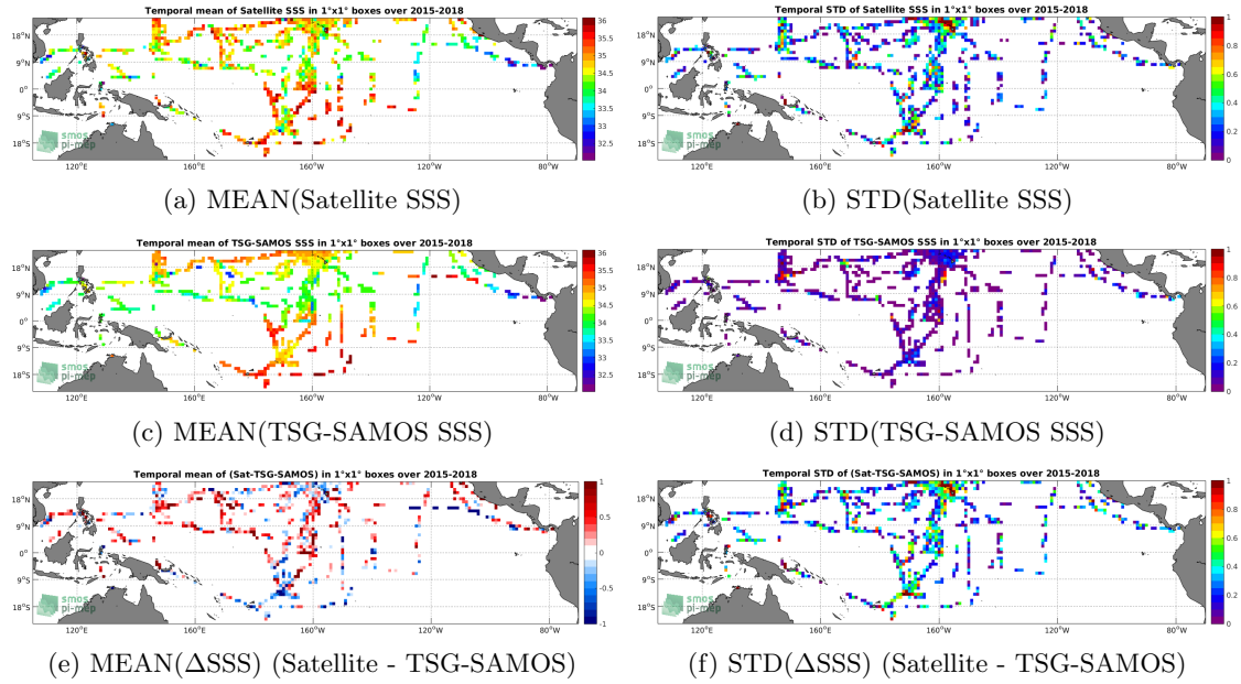
Figure 6: Temporal mean (left) and STD (right) of SSS from SMAP-L2-JPL-V4 (top), TSG-SAMOS (middle), and of \Delta SSS (Satellite - TSG-SAMOS). Only match-up pairs are used to generate these maps.
