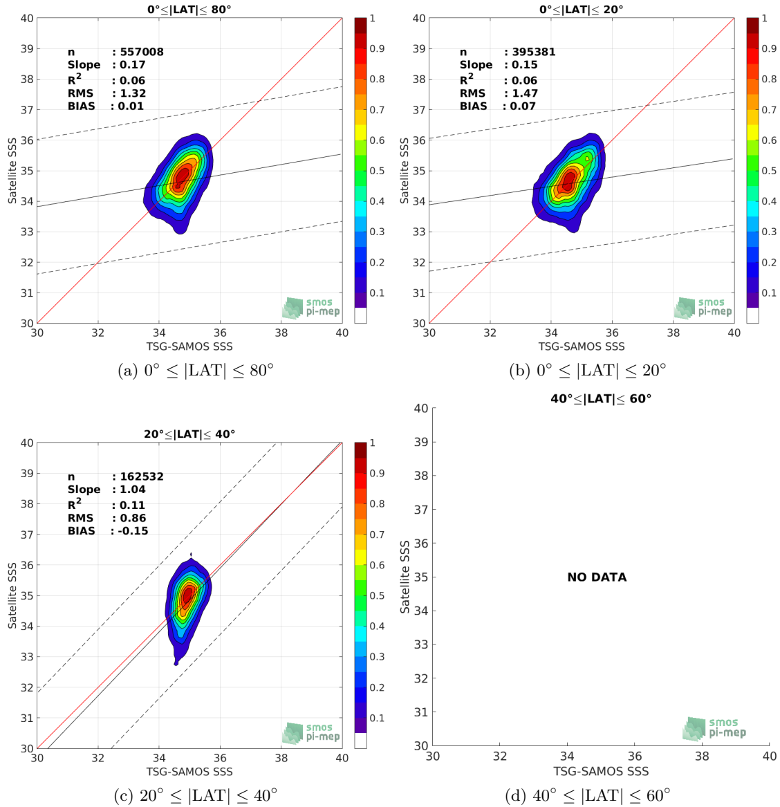
Figure 9: Contour maps of the concentration of SMAP-L2-JPL-V4 SSS (y-axis) versus TSG-SAMOS SSS (x-axis) at match-up pairs for different latitude bands. For each plot, the red line shows x=y . The black thin and dashed lines indicate a linear fit through the data cloud and the \pm 95\% confidence levels, respectively. The number match-up pairs n , the slope and R^2 coefficient of the linear fit, the root mean square (RMS) and the mean bias between satellite and in situ data are indicated for each latitude band in each plots.
