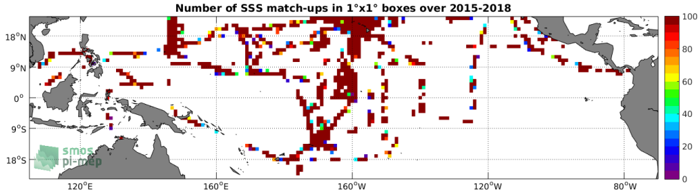
Figure 4: Number of SSS match-ups between TSG-SAMOS SSS and the SMAP-L2-JPL-V4 SSS product for the Tropical Pacific Ocean Pi-MEP region over 1^\circ \times 1^\circ boxes and for the full satellite product period.
