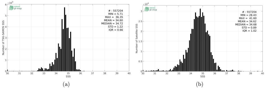
Figure 2: Histograms of SSS from TSG-SAMOS (a) and SMAP-L2-JPL-V4 (b) considering all match-up pairs per bins of 0.1 over the Tropical Pacific Ocean Pi-MEP region and for the full satellite product period.
