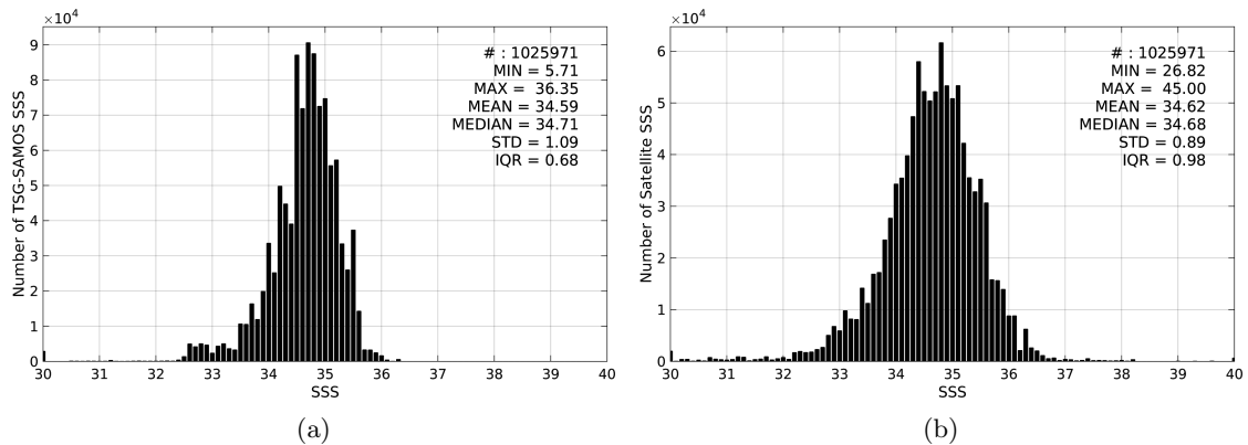
Figure 2: Histograms of SSS from TSG-SAMOS (a) and SMAP-L2-JPL-V4 (b) considering all match-up pairs per bins of 0.1 over the Tropical Pacific Ocean Pi-MEP region and for the full satellite product period.
