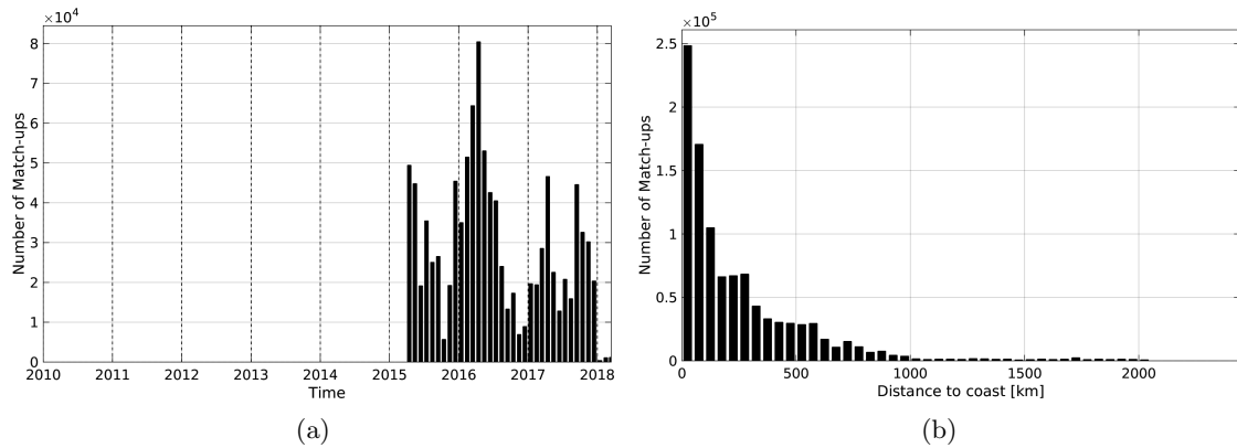
Figure 1: Number of match-ups between TSG-SAMOS and SMAP-L2-JPL-V4 SSS as a function of time (a) and as function of the distance to coast (b) over the Tropical Pacific Ocean Pi-MEP region and for the full satellite product period.
