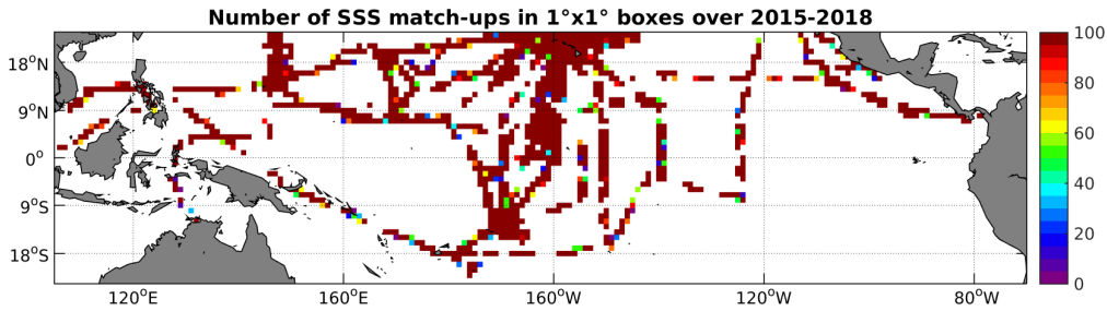
Figure 4: Number of SSS match-ups between TSG-SAMOS SSS and the SMAP-L2-JPL-V4 SSS product for the Tropical Pacific Ocean Pi-MEP region over 1^\circ \times 1^\circ boxes and for the full satellite product period.
