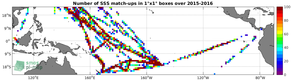
Figure 4: Number of SSS match-ups between TSG-LEGOS-DM SSS and the SMAP-L2-JPL-V4 SSS product for the Tropical Pacific Ocean Pi-MEP region over 1^\circ \times 1^\circ boxes and for the full satellite product period.
