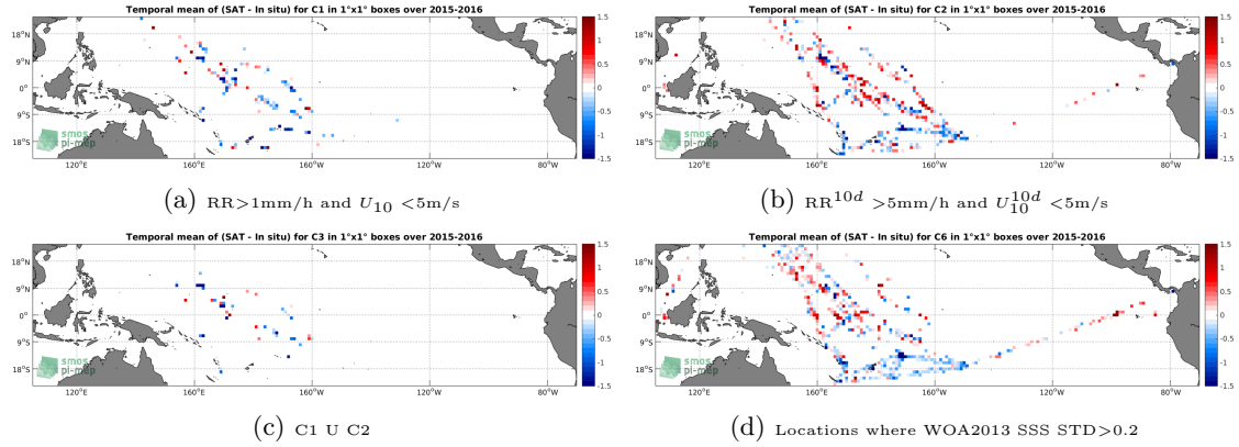
Figure 12: Temporal mean gridded over spatial boxes of size 1^\circ \times 1^\circ of \Delta SSS (SMAP-L2-JPL-V4 - TSG-LEGOS-DM) for 4 different subdatasets corresponding to: RR > 1\text{mm/h} and U_{10} < 5\text{m/s} (a), RR^{10d} > 5\text{mm/h} and U_{10}^{10d} < 5\text{m/s} (b), C1 U C2 (c), Locations where WOA2013 SSS STD > 0.2 (d).
