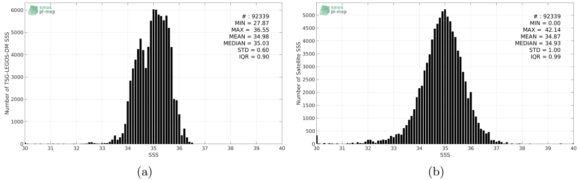
Figure 2: Histograms of SSS from TSG-LEGOS-DM (a) and SMAP-L2-JPL-V4 (b) considering all match-up pairs per bins of 0.1 over the Tropical Pacific Ocean Pi-MEP region and for the full satellite product period.
