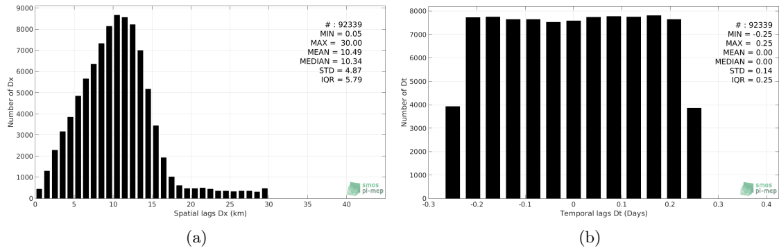
Figure 5: Histograms of the spatial (a) and temporal (b) lags between the time of the TSG-LEGOS-DM measurements and the date of the corresponding SMAP-L2-JPL-V4 SSS product.
