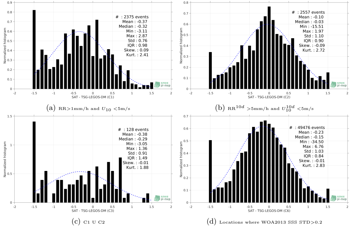
Figure 13: Normalized histogram of \Delta\text{SSS} (SMAP-L2-JPL-V4 - TSG-LEGOS-DM) for 6 different subdatasets corresponding to: \text{RR} > 1\text{mm/h} and U_{10} < 5\text{m/s} (a), \text{RR}^{10d} > 5\text{mm/h} and U_{10}^{10d} < 5\text{m/s} (b), C1 U C2 (c), Locations where WOA2013 SSS STD > 0.2 (d).
