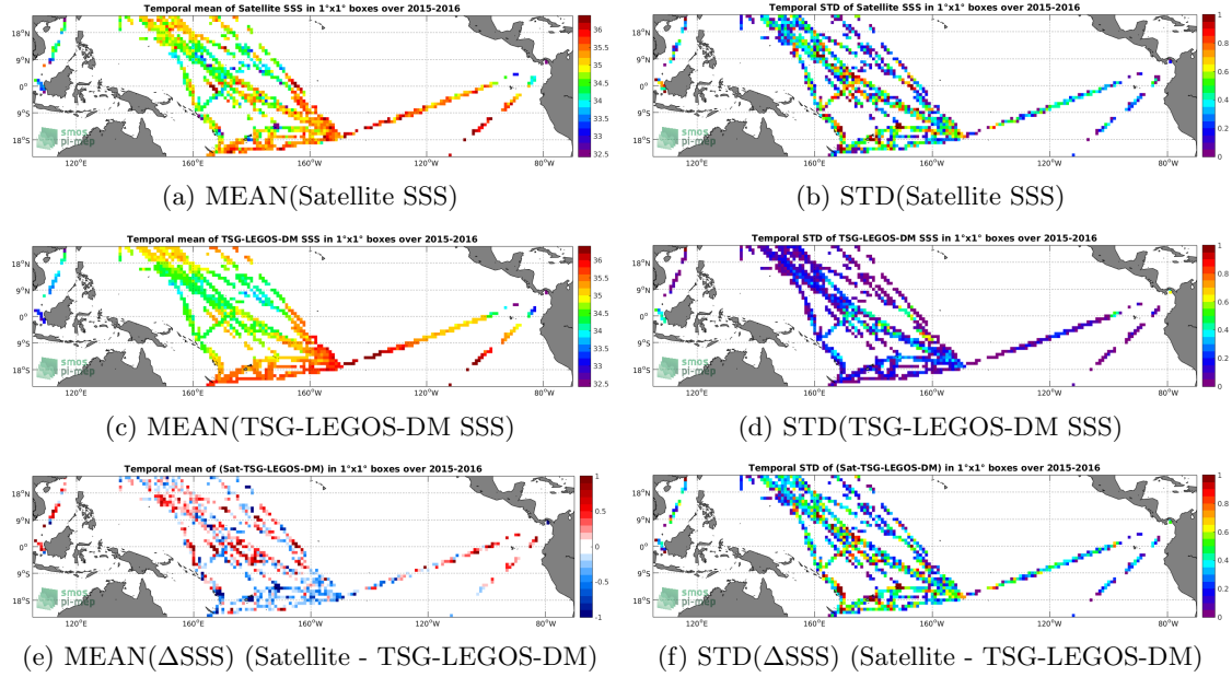
Figure 6: Temporal mean (left) and STD (right) of SSS from SMAP-L2-JPL-V4 (top), TSG-LEGOS-DM (middle), and of \Delta SSS (Satellite - TSG-LEGOS-DM). Only match-up pairs are used to generate these maps.
