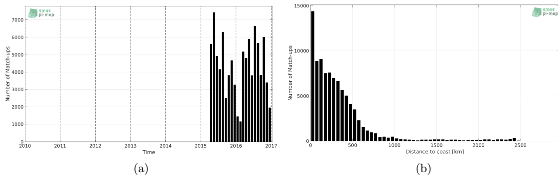
Figure 1: Number of match-ups between TSG-LEGOS-DM and SMAP-L2-JPL-V4 SSS as a function of time (a) and as function of the distance to coast (b) over the Tropical Pacific Ocean Pi-MEP region and for the full satellite product period.
