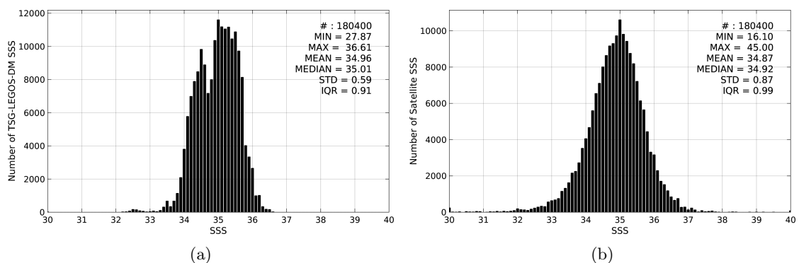
Figure 2: Histograms of SSS from TSG-LEGOS-DM (a) and SMAP-L2-JPL-V4 (b) considering all match-up pairs per bins of 0.1 over the Tropical Pacific Ocean Pi-MEP region and for the full satellite product period.
