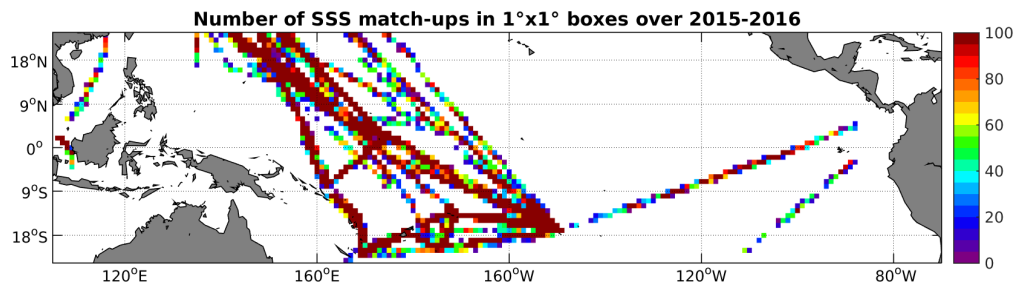
Figure 4: Number of SSS match-ups between TSG-LEGOS-DM SSS and the SMAP-L2-JPL-V4 SSS product for the Tropical Pacific Ocean Pi-MEP region over 1^\circ \times 1^\circ boxes and for the full satellite product period.
