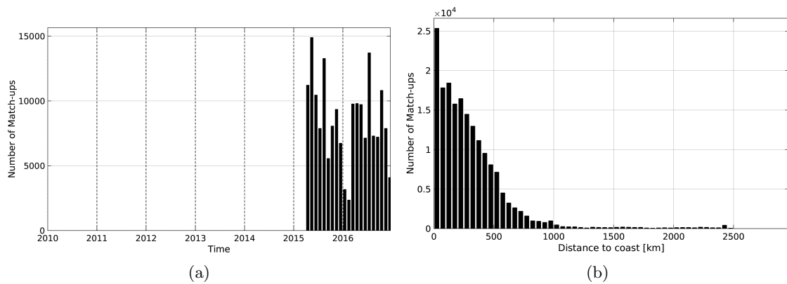
Figure 1: Number of match-ups between TSG-LEGOS-DM and SMAP-L2-JPL-V4 SSS as a function of time (a) and as function of the distance to coast (b) over the Tropical Pacific Ocean Pi-MEP region and for the full satellite product period.
