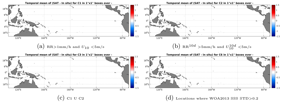
Figure 12: Temporal mean gridded over spatial boxes of size 1^\circ \times 1^\circ of \Delta SSS (SMAP-L2-JPL-V4 - TSG-GOSUD-Sailing-ship) for 4 different subdatasets corresponding to:RR >1 mm/h and U_{10} < 5 m/s (a), RR 10d > 5 mm/h and U_{10}^{10d} < 5 m/s (b), C1 U C2 (c),Locations where WOA2013 SSS STD >0.2 (d).
