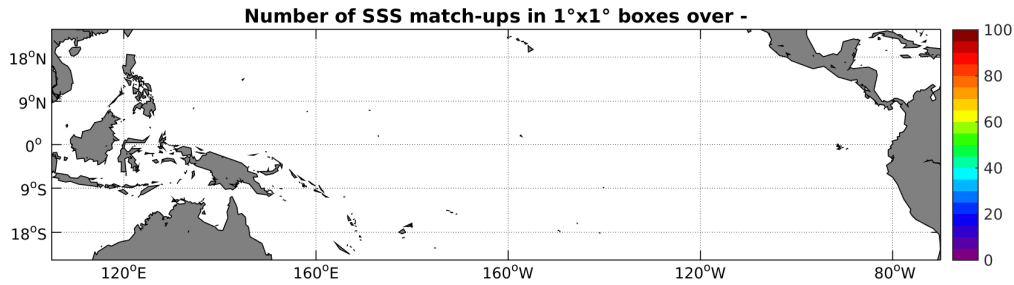
Figure 4: Number of SSS match-ups between TSG-GOSUD-Sailing-ship SSS and the SMAP-L2-JPL-V4 SSS product for the Tropical Pacific Ocean Pi-MEP region over 1^\circ \times 1^\circ boxes and for the full satellite product period.
