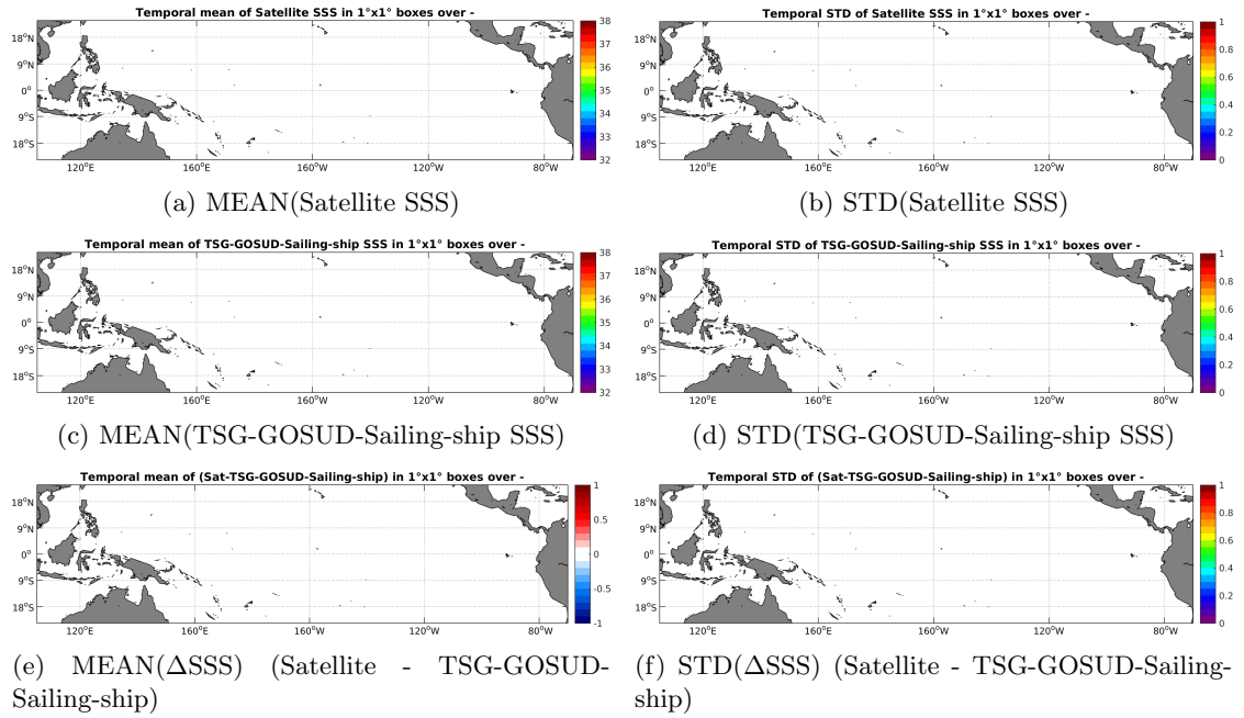
Figure 6: Temporal mean (left) and STD (right) of SSS from SMAP-L2-JPL-V4 (top), TSG-GOSUD-Sailing-ship (middle), and of \Delta SSS (Satellite - TSG-GOSUD-Sailing-ship). Only match-up pairs are used to generate these maps.
