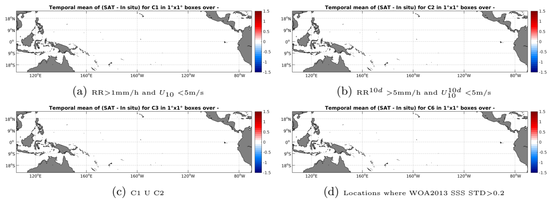
Figure 12: Temporal mean gridded over spatial boxes of size 1^\circ \times 1^\circ of \Delta SSS (SMAP-L2-JPL-V4 - TSG-GOSUD-Sailing-ship) for 4 different subdatasets corresponding to: RR > 1 mm/h and U_{10} < 5 m/s (a), RR ^{10d} > 5 mm/h and U_{10}^{10d} < 5 m/s (b), C1 U C2 (c), Locations where WOA2013 SSS STD > 0.2 (d).
