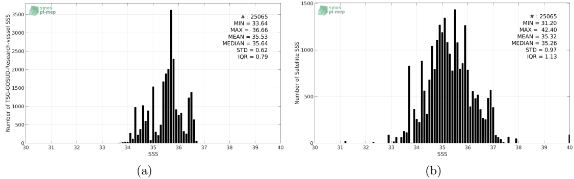
Figure 2: Histograms of SSS from TSG-GOSUD-Research-vessel (a) and SMAP-L2-JPL-V4 (b) considering all match-up pairs per bins of 0.1 over the Tropical Pacific Ocean Pi-MEP region and for the full satellite product period.
