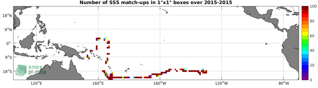
Figure 4: Number of SSS match-ups between TSG-GOSUD-Research-vessel SSS and the SMAP-L2-JPL-V4 SSS product for the Tropical Pacific Ocean Pi-MEP region over 1^\circ \times 1^\circ boxes and for the full satellite product period.
