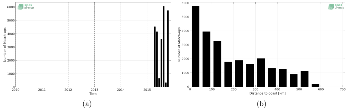
Figure 1: Number of match-ups between TSG-GOSUD-Research-vessel and SMAP-L2-JPL-V4 SSS as a function of time (a) and as function of the distance to coast (b) over the Tropical Pacific Ocean Pi-MEP region and for the full satellite product period.
