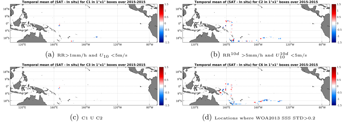
Figure 12: Temporal mean gridded over spatial boxes of size 1^\circ \times 1^\circ of \Delta SSS (SMAP-L2-JPL-V4 - TSG-GOSUD-Research-vessel) for 4 different subdatasets corresponding to: RR > 1mm/h and U_{10} < 5 m/s (a), RR 10d > 5mm/h and U_{10}^{10d} < 5 m/s (b), C1 U C2 (c), Locations where WOA2013 SSS STD > 0.2 (d).
