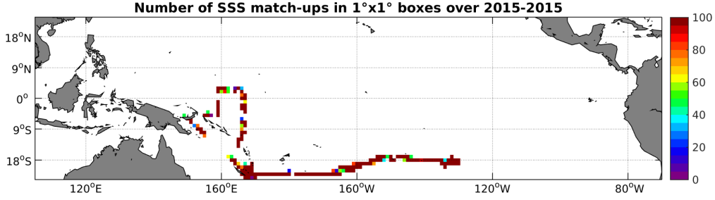
Figure 4: Number of SSS match-ups between TSG-GOSUD-Research-vessel SSS and the SMAP-L2-JPL-V4 SSS product for the Tropical Pacific Ocean Pi-MEP region over 1^\circ \times 1^\circ boxes and for the full satellite product period.
