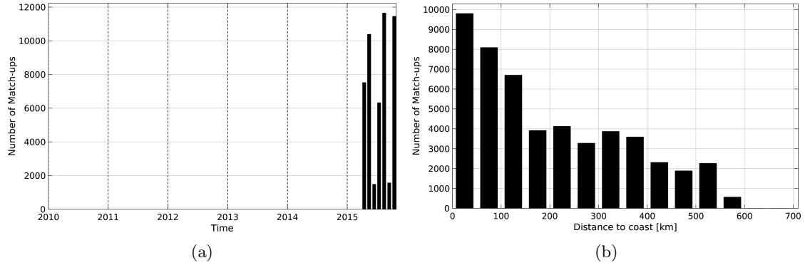
Figure 1: Number of match-ups between TSG-GOSUD-Research-vessel and SMAP-L2-JPL-V4 SSS as a function of time (a) and as function of the distance to coast (b) over the Tropical Pacific Ocean Pi-MEP region and for the full satellite product period.
