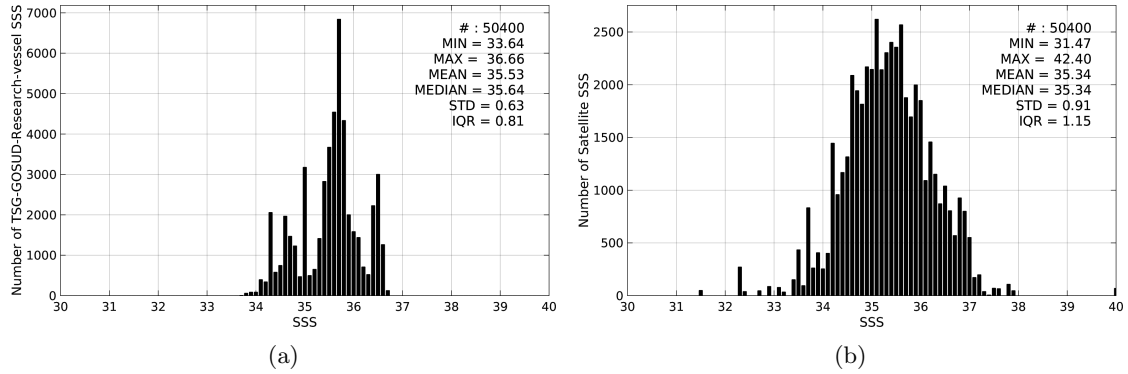
Figure 2: Histograms of SSS from TSG-GOSUD-Research-vessel (a) and SMAP-L2-JPL-V4 (b) considering all match-up pairs per bins of 0.1 over the Tropical Pacific Ocean Pi-MEP region and for the full satellite product period.
