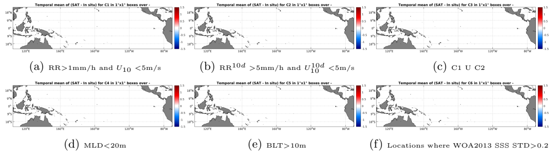
Figure 12: Temporal mean gridded over spatial boxes of size 1^\circ \times 1^\circ of \Delta SSS (SMAP-L2-JPL-V4 - Sea mammals) for 6 different subdatasets corresponding to: RR > 1\text{mm/h} and U_{10} < 5\text{m/s} (a), RR^{10d} > 5\text{mm/h} and U_{10}^{10d} < 5\text{m/s} (b), C1 U C2 (c), MLD < 20\text{m} (d), BLT > 10\text{m} (e), Locations where WOA2013 SSS STD > 0.2 (f).
