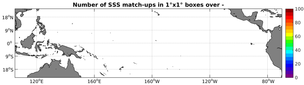
Figure 4: Number of SSS match-ups between Sea mammals SSS and the SMAP-L2-JPL-V4 SSS product for the Tropical Pacific Ocean Pi-MEP region over 1^\circ \times 1^\circ boxes and for the full satellite product period.
