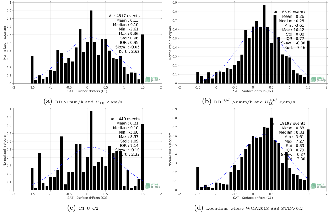
Figure 12: Normalized histogram of \Delta SSS (SMAP-L2-JPL-V4 - Surface drifters) for 6 different subdatasets corresponding to: RR > 1mm/h and U_{10} < 5 m/s (a), RR^{10d} > 5 mm/h and U_{10}^{10d} < 5 m/s (b), C1 U C2 (c), Locations where WOA2013 SSS STD > 0.2 (d).
