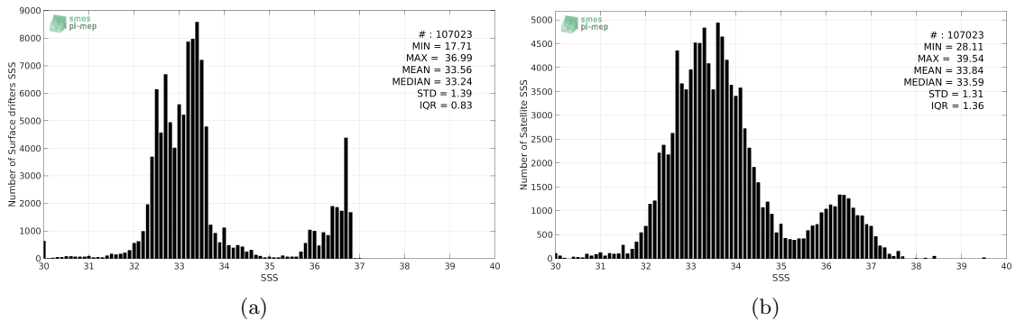
Figure 2: Histograms of SSS from Surface drifters (a) and SMAP-L2-JPL-V4 (b) considering all match-up pairs per bins of 0.1 over the Tropical Pacific Ocean Pi-MEP region and for the full satellite product period.
