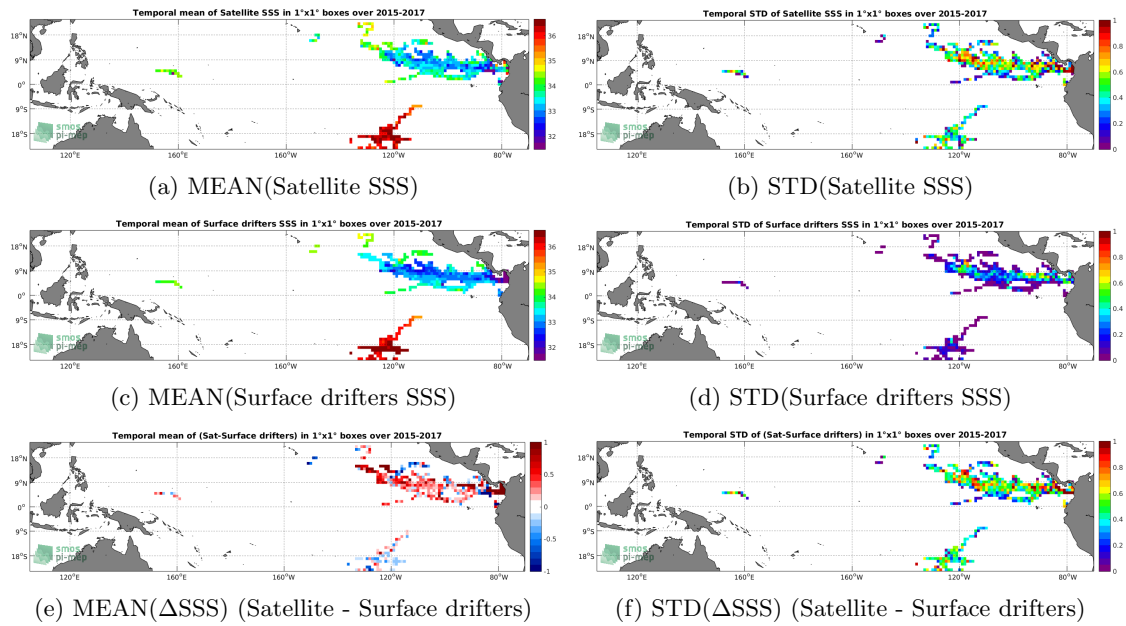
Figure 5: Temporal mean (left) and STD (right) of SSS from SMAP-L2-JPL-V4 (top), Surface drifters (middle), and of \Delta SSS (Satellite - Surface drifters). Only match-up pairs are used to generate these maps.
