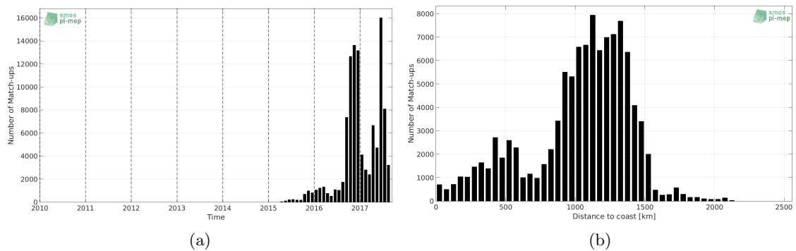
Figure 1: Number of match-ups between Surface drifters and SMAP-L2-JPL-V4 SSS as a function of time (a) and as function of the distance to coast (b) over the Tropical Pacific Ocean Pi-MEP region and for the full satellite product period.
