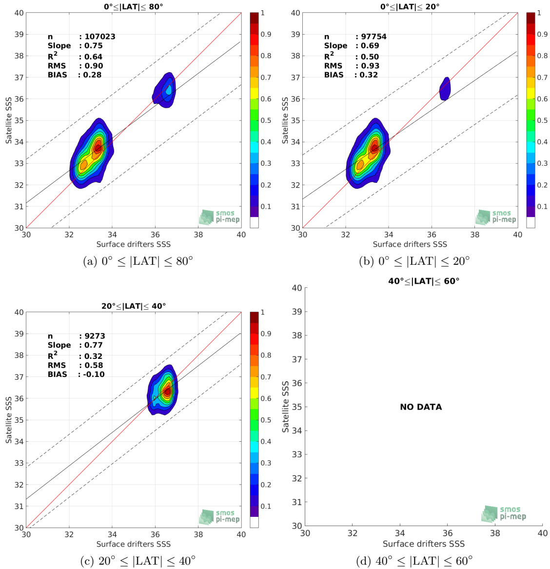
Figure 8: Contour maps of the concentration of SMAP-L2-JPL-V4 SSS (y-axis) versus Surface drifters SSS (x-axis) at match-up pairs for different latitude bands. For each plot, the red line shows x=y . The black thin and dashed lines indicate a linear fit through the data cloud and the \pm 95\% confidence levels, respectively. The number match-up pairs n , the slope and R^2 coefficient of the linear fit, the root mean square (RMS) and the mean bias between satellite and in situ data are indicated for each latitude band in each plots.
