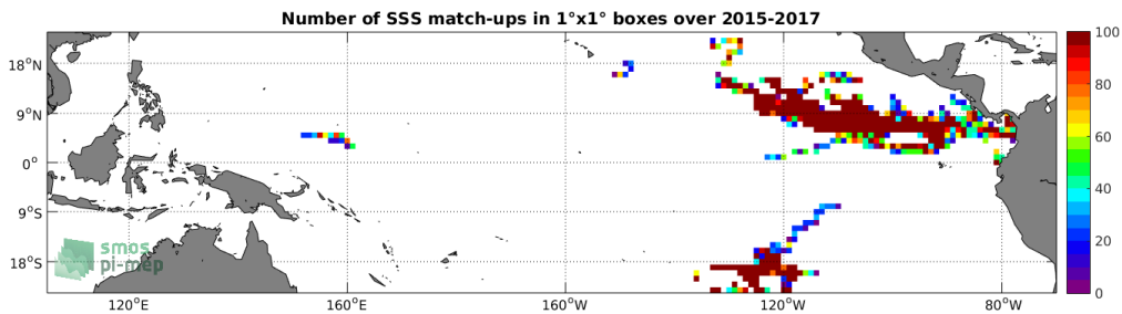
Figure 3: Number of SSS match-ups between Surface drifters SSS and the SMAP-L2-JPL-V4 SSS product for the Tropical Pacific Ocean Pi-MEP region over 1°x1° boxes and for the full satellite product period.
