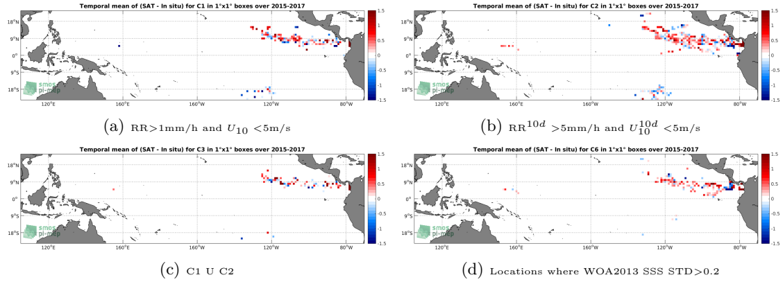
Figure 11: Temporal mean gridded over spatial boxes of size 1^\circ \times 1^\circ of \Delta SSS (SMAP-L2-JPL-V4 - Surface drifters) for 4 different subdatasets corresponding to: RR > 1\text{mm/h} and U_{10} < 5\text{m/s} (a), RR^{10d} > 5\text{mm/h} and U_{10}^{10d} < 5\text{m/s} (b), C1 U C2 (c), Locations where WOA2013 SSS STD > 0.2 (d).
