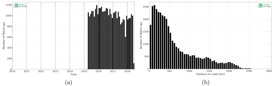
Figure 1: Number of match-ups between Argo and SMAP-L2-JPL-V4 SSS as a function of time (a) and as function of the distance to coast (b) over the Tropical Pacific Ocean Pi-MEP region and for the full satellite product period.
