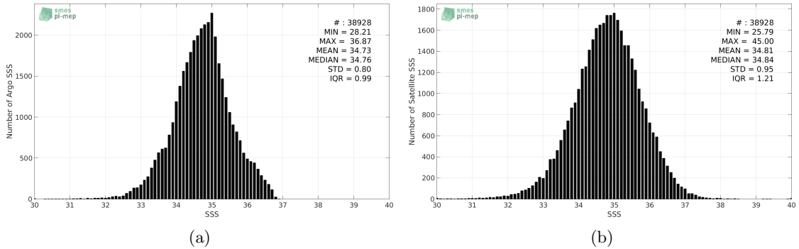
Figure 2: Histograms of SSS from Argo (a) and SMAP-L2-JPL-V4 (b) considering all match-up pairs per bins of 0.1 over the Tropical Pacific Ocean Pi-MEP region and for the full satellite product period.
