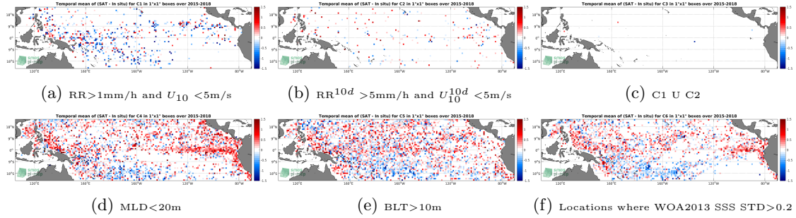
Figure 12: Temporal mean gridded over spatial boxes of size 1^\circ \times 1^\circ of \Delta SSS (SMAP-L2-JPL-V4 - Argo) for 6 different subdatasets corresponding to: RR > 1\text{mm/h} and U_{10} < 5\text{m/s} (a), RR^{10d} > 5\text{mm/h} and U_{10}^{10d} < 5\text{m/s} (b), C1 U C2 (c), MLD < 20\text{m} (d), BLT > 10\text{m} (e), Locations where WOA2013 SSS STD > 0.2 (f).
