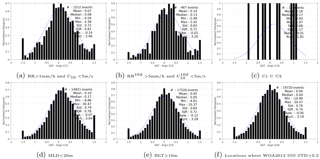
Figure 13: Normalized histogram of ΔSSS (SMAP-L2-JPL-V4 - Argo) for 6 different subdatasets corresponding to: RR>1mm/h and U_{10} < 5\text{m/s} (a), RR^{10d} > 5\text{mm/h} and U_{10}^{10d} < 5\text{m/s} (b), C1 U C2 (c),MLD<20m (d),BLT>10m (e),Locations where WOA2013 SSS STD>0.2 (f).
