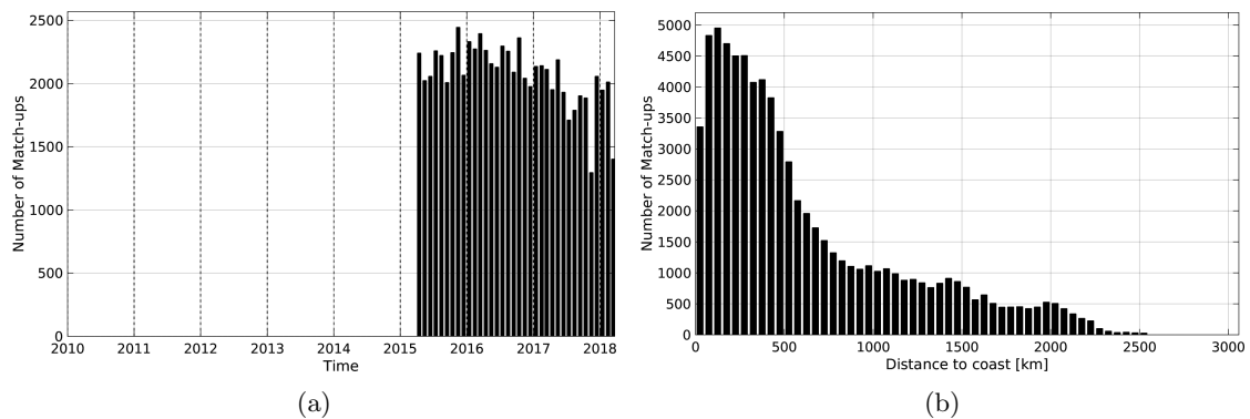
Figure 1: Number of match-ups between Argo and SMAP-L2-JPL-V4 SSS as a function of time (a) and as function of the distance to coast (b) over the Tropical Pacific Ocean Pi-MEP region and for the full satellite product period.
