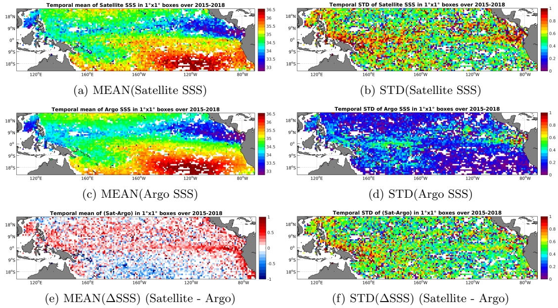
Figure 6: Temporal mean (left) and STD (right) of SSS from SMAP-L2-JPL-V4 (top), Argo (middle), and of \Delta SSS (Satellite - Argo). Only match-up pairs are used to generate these maps.
