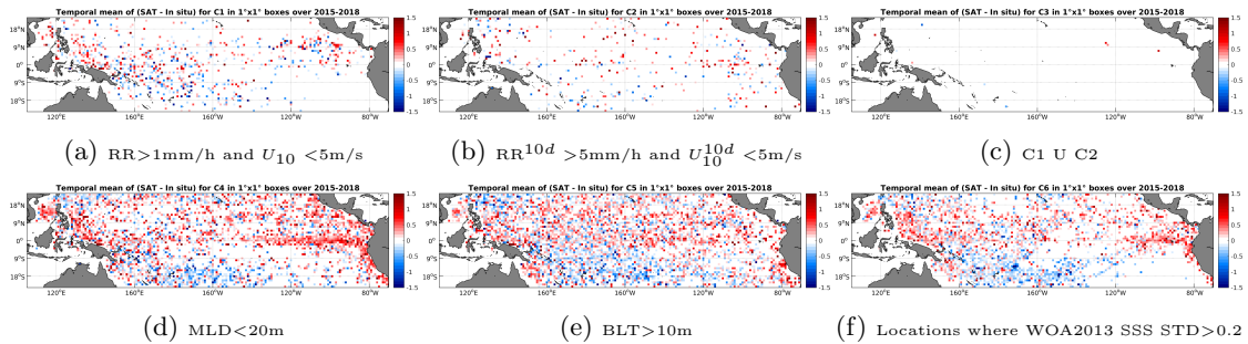
Figure 12: Temporal mean gridded over spatial boxes of size 1°x1° of ΔSSS (SMAP-L2-JPL-V4 - Argo) for 6 different subdatasets corresponding to:RR>1mm/h and U_{10} < 5\text{m/s} (a), RR^{10d} > 5\text{mm/h} and U_{10}^{10d} < 5\text{m/s} (b), C1 U C2 (c),MLD<20m (d),BLT>10m (e),Locations where WOA2013 SSS STD>0.2 (f).
