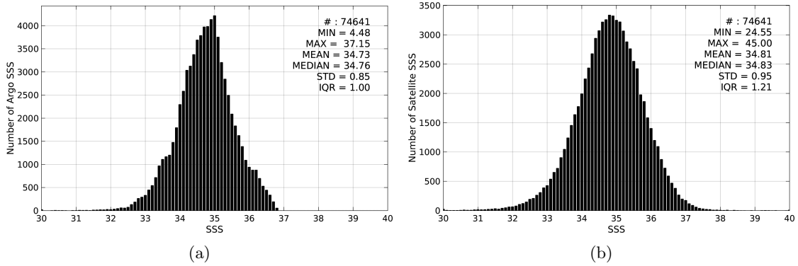
Figure 2: Histograms of SSS from Argo (a) and SMAP-L2-JPL-V4 (b) considering all match-up pairs per bins of 0.1 over the Tropical Pacific Ocean Pi-MEP region and for the full satellite product period.
