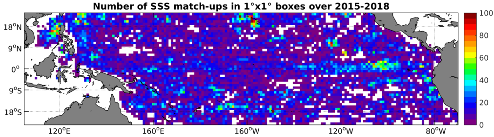
Figure 4: Number of SSS match-ups between Argo SSS and the SMAP-L2-JPL-V4 SSS product for the Tropical Pacific Ocean Pi-MEP region over 1^\circ \times 1^\circ boxes and for the full satellite product period.
