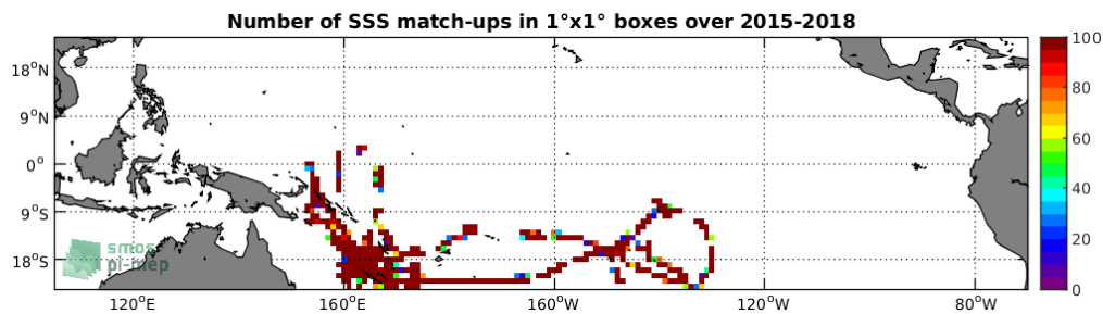
Figure 4: Number of SSS match-ups between TSG-GOSUD-Research-vessel SSS and the SMAP-L2-JPL-V4.2 SSS product for the Tropical Pacific Ocean Pi-MEP region over 1^\circ \times 1^\circ boxes and for the full satellite product period.
