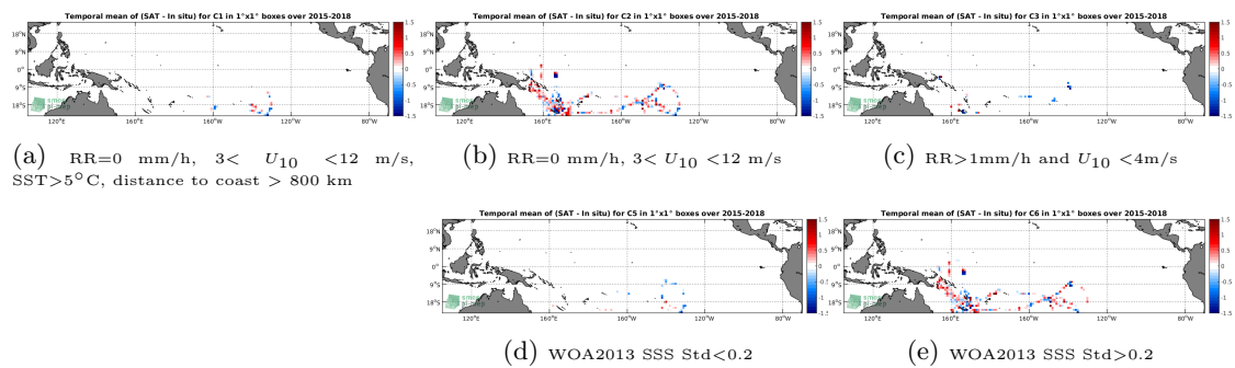
Figure 12: Temporal mean gridded over spatial boxes of size 1^\circ \times 1^\circ of \Delta SSS (SMAP-L2-JPL-V4.2 - TSG-GOSUD-Research-vessel) for 5 different subdatasets corresponding to:RR=0 mm/h, 3 < U_{10} < 12 m/s, SST >5^\circ C, distance to coast > 800 km (a), RR=0 mm/h, 3 < U_{10} < 12 m/s (b), RR >1 mm/h and U_{10} < 4 m/s (c), WOA2013 SSS Std <0.2 (d), WOA2013 SSS Std >0.2 (e).
