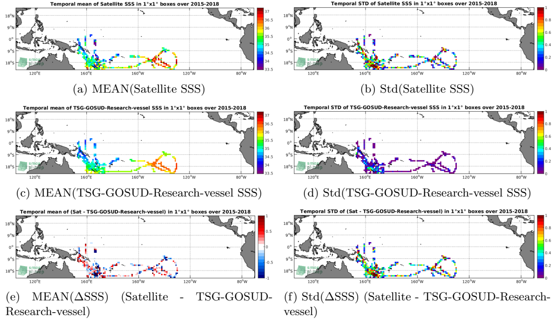
Figure 6: Temporal mean (left) and Std (right) of SSS from SMAP-L2-JPL-V4.2 (top), TSG-GOSUD-Research-vessel (middle), and of \Delta SSS (Satellite - TSG-GOSUD-Research-vessel). Only match-up pairs are used to generate these maps.
