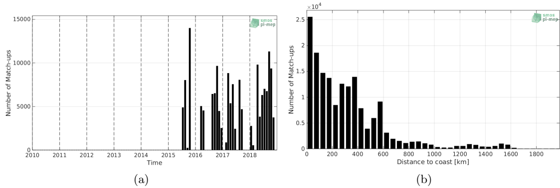
Figure 1: Number of match-ups between TSG-GOSUD-Research-vessel and SMAP-L2-JPL-V4.2 SSS as a function of time (a) and as function of the distance to coast (b) over the Tropical Pacific Ocean Pi-MEP region and for the full satellite product period.
