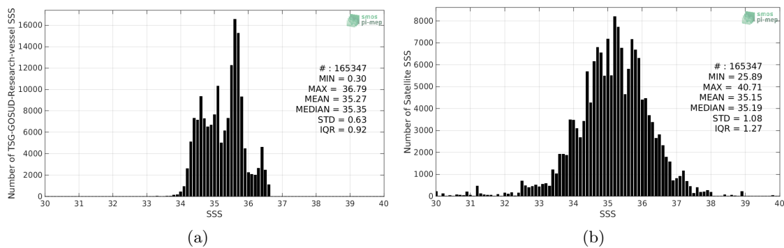
Figure 2: Histograms of SSS from TSG-GOSUD-Research-vessel (a) and SMAP-L2-JPL-V4.2 (b) considering all match-up pairs per bins of 0.1 over the Tropical Pacific Ocean Pi-MEP region and for the full satellite product period.
