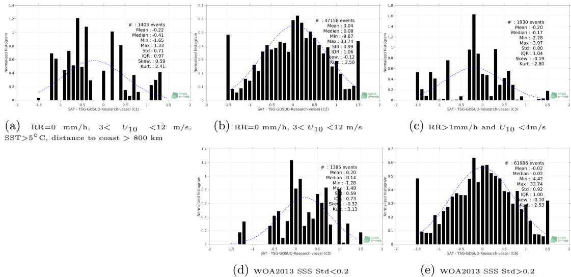
Figure 13: Normalized histogram of \Delta SSS (SMAP-L2-JPL-V4.2 - TSG-GOSUD-Research-vessel) for 5 different subdatasets corresponding to: RR=0 mm/h, 3 < U_{10} < 12 m/s, SST >5^\circ C, distance to coast > 800 km (a), RR=0 mm/h, 3 < U_{10} < 12 m/s (b), RR >1 mm/h and U_{10} < 4 m/s (c), WOA2013 SSS Std <0.2 (d), WOA2013 SSS Std >0.2 (e).
