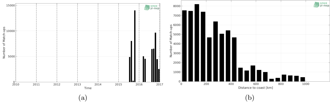
Figure 1: Number of match-ups between TSG-GOSUD-Research-vessel and SMAP-L2-JPL-V4.2 SSS as a function of time (a) and as function of the distance to coast (b) over the Tropical Pacific Ocean Pi-MEP region and for the full satellite product period.
