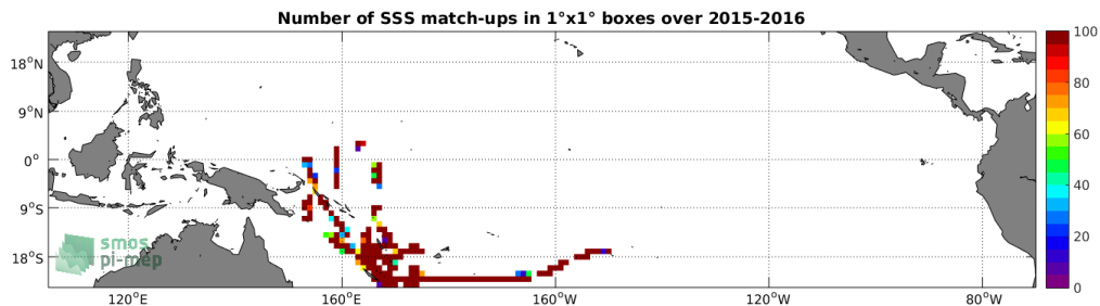
Figure 4: Number of SSS match-ups between TSG-GOSUD-Research-vessel SSS and the SMAP-L2-JPL-V4.2 SSS product for the Tropical Pacific Ocean Pi-MEP region over 1^\circ \times 1^\circ boxes and for the full satellite product period.
