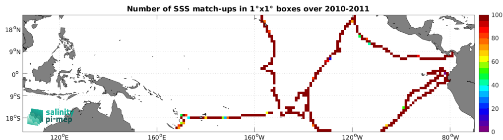
Figure 5: Number of SSS match-ups between TSG (GOSUD-Sailing-ship) SSS and the ISAS v7 - Monthly (Ifremer-LOPS-CMEMS) SSS product for the Tropical Pacific Ocean Pi-MEP region over 1^\circ \times 1^\circ boxes and for the full satellite product period.
