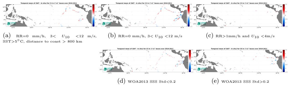
Figure 14: Temporal mean gridded over spatial boxes of size 1^\circ \times 1^\circ of \Delta\text{SSS} (ISAS v7 - Monthly (Ifremer-LOPS-CMEMS) - TSG (GOSUD-Sailing-ship)) for 5 different subdatasets corresponding to:RR=0 mm/h, 3 < U_{10} < 12 m/s, SST > 5^\circ\text{C} , distance to coast > 800 km (a), RR=0 mm/h, 3 < U_{10} < 12 m/s (b), RR > 1 mm/h and U_{10} < 4 m/s (c), WOA2013 SSS Std < 0.2 (d), WOA2013 SSS Std > 0.2 (e).
