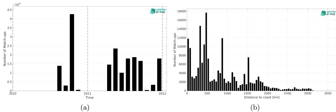
Figure 2: Number of match-ups between TSG (GOSUD-Sailing-ship) and ISAS v7 - Monthly (Ifremer-LOPS-CMEMS) SSS as a function of time (a) and as function of the distance to coast (b) over the Tropical Pacific Ocean Pi-MEP region and for the full satellite product period.
