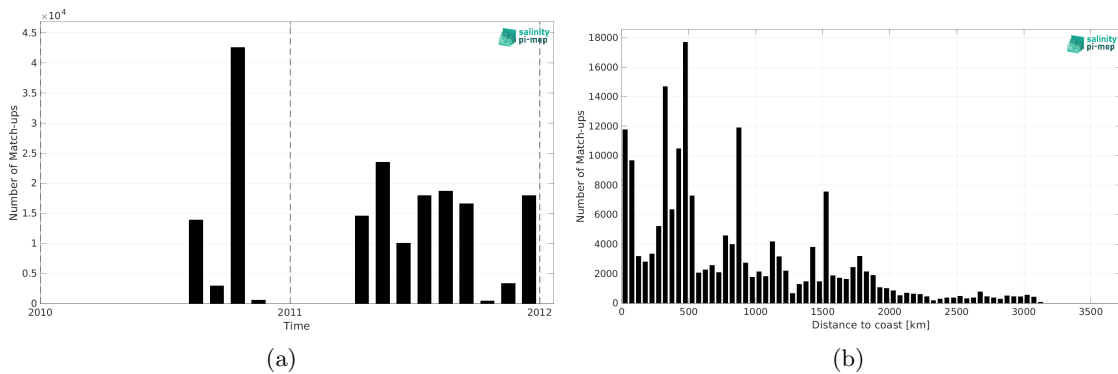
Figure 2: Number of match-ups between TSG (GOSUD-Sailing-ship) and ISAS SSS as a function of time (a) and as function of the distance to coast (b) over the Tropical Pacific Ocean Pi-MEP region and for the full satellite product period.
