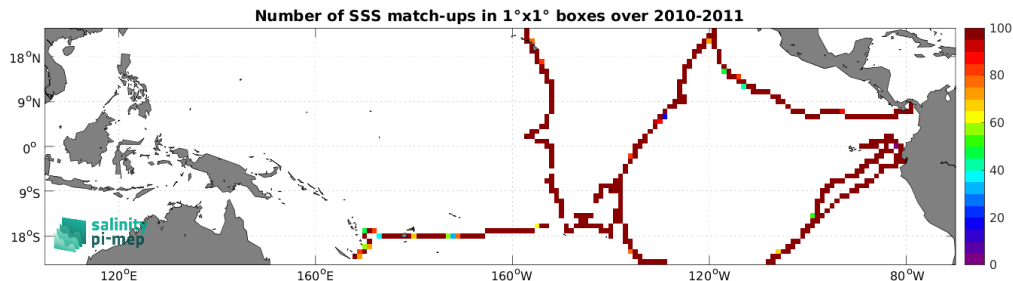
Figure 5: Number of SSS match-ups between TSG (GOSUD-Sailing-ship) SSS and the ISAS SSS product for the Tropical Pacific Ocean Pi-MEP region over 1^\circ \times 1^\circ boxes and for the full satellite product period.
