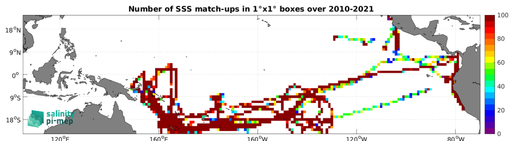
Figure 5: Number of SSS match-ups between TSG (GOSUD-Research-vessel) SSS and the ISAS SSS product for the Tropical Pacific Ocean Pi-MEP region over 1^\circ \times 1^\circ boxes and for the full satellite product period.
