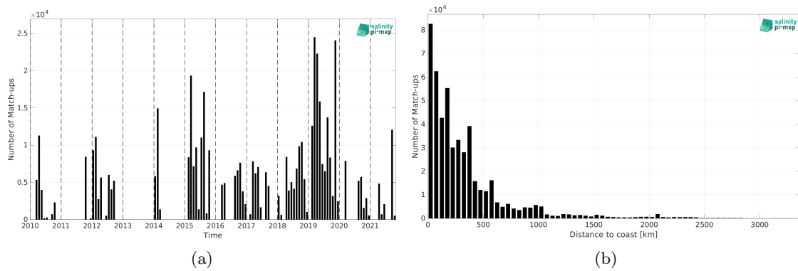
Figure 2: Number of match-ups between TSG (GOSUD-Research-vessel) and ISAS SSS as a function of time (a) and as function of the distance to coast (b) over the Tropical Pacific Ocean Pi-MEP region and for the full satellite product period.
