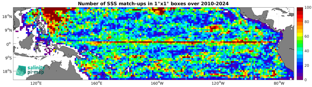
Figure 5: Number of SSS match-ups between Argo SSS and the ISAS v7 - Monthly (Ifremer-LOPS-CMEMS) SSS product for the Tropical Pacific Ocean Pi-MEP region over 1^\circ \times 1^\circ boxes and for the full satellite product period.
