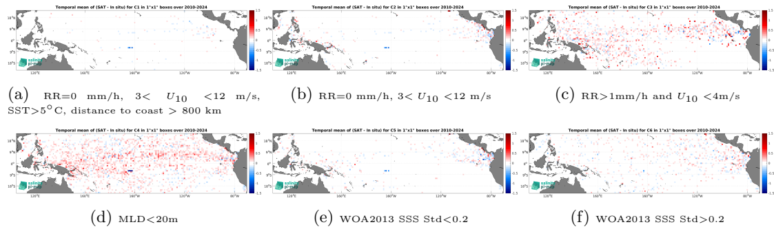
Figure 14: Temporal mean gridded over spatial boxes of size 1^\circ \times 1^\circ of \Delta SSS (ISAS v7 - Monthly (Ifremer-LOPS-CMEMS) - Argo) for 6 different subdatasets corresponding to:RR=0 mm/h, 3 < U_{10} < 12 m/s, SST>5°C, distance to coast > 800 km (a), RR=0 mm/h, 3 < U_{10} < 12 m/s (b), RR>1mm/h and U_{10} < 4 m/s (c),MLD<20m (d),WOA2013 SSS Std<0.2 (e),WOA2013 SSS Std>0.2 (f).
