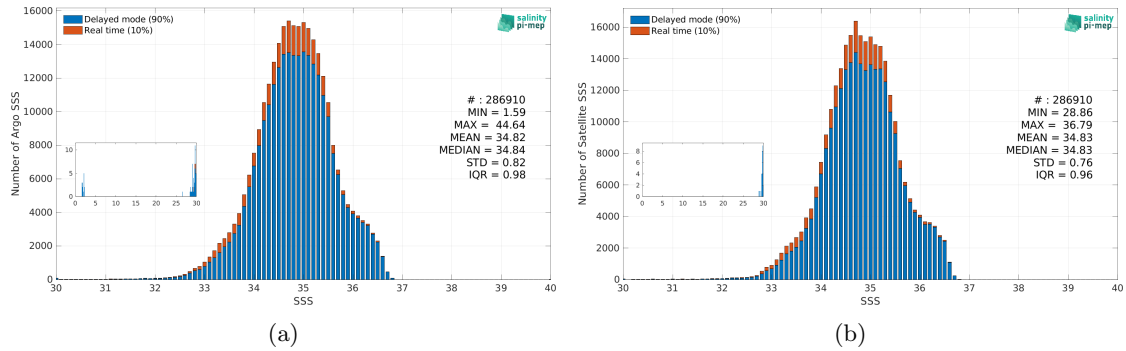
Figure 3: Histograms of SSS from Argo (a) and ISAS v7 - Monthly (Ifremer-LOPS-CMEMS) (b) considering all match-up pairs per bins of 0.1 over the Tropical Pacific Ocean Pi-MEP region and for the full satellite product period.
