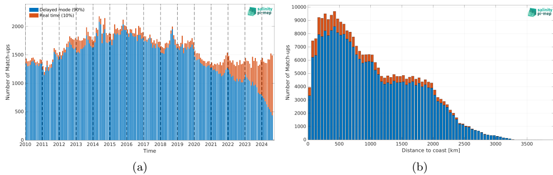
Figure 2: Number of match-ups between Argo and ISAS v7 - Monthly (Ifremer-LOPS-CMEMS) SSS as a function of time (a) and as function of the distance to coast (b) over the Tropical Pacific Ocean Pi-MEP region and for the full satellite product period.
