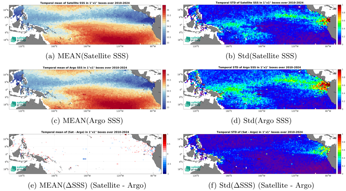
Figure 7: Temporal mean (left) and Std (right) of SSS from ISAS v7 - Monthly (Ifremer-LOPS-CMEMS) (top), Argo (middle), and of \Delta SSS (Satellite - Argo). Only match-up pairs are used to generate these maps.
