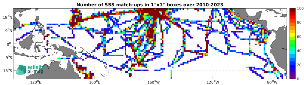
Figure 5: Number of SSS match-ups between TSG (SAMOS) SSS and the CCI SSS L4 Merged-OI v5.5 - 7-day running (ESA) SSS product for the Tropical Pacific Ocean Pi-MEP region over 1^\circ \times 1^\circ boxes and for the full satellite product period.
