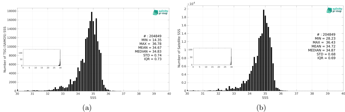
Figure 3: Histograms of SSS from TSG (SAMOS) (a) and CCI SSS L4 Merged-OI v5.5 - 7-day running (ESA) (b) considering all match-up pairs per bins of 0.1 over the Tropical Pacific Ocean Pi-MEP region and for the full satellite product period.
