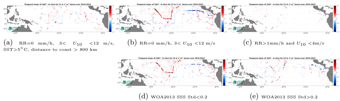
Figure 14: Temporal mean gridded over spatial boxes of size 1^\circ \times 1^\circ of \Delta\text{SSS} (CCI SSS L4 Merged-OI v5.5 - 7-day running (ESA) - TSG (SAMOS)) for 5 different subdatasets corresponding to:RR=0 mm/h, 3 < U_{10} < 12 m/s, SST > 5^\circ\text{C} , distance to coast > 800 km (a), RR=0 mm/h, 3 < U_{10} < 12 m/s (b), RR > 1 mm/h and U_{10} < 4 m/s (c), WOA2013 SSS Std < 0.2 (d), WOA2013 SSS Std > 0.2 (e).
