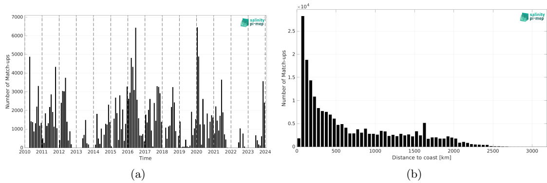
Figure 2: Number of match-ups between TSG (SAMOS) and CCI SSS L4 Merged-OI v5.5 - 7-day running (ESA) SSS as a function of time (a) and as function of the distance to coast (b) over the Tropical Pacific Ocean Pi-MEP region and for the full satellite product period.
