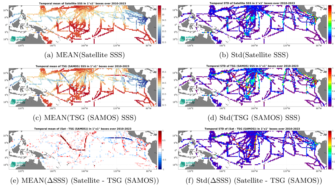
Figure 7: Temporal mean (left) and Std (right) of SSS from CCI SSS L4 Merged-OI v5.5 - 7-day running (ESA) (top), TSG (SAMOS) (middle), and of \Delta SSS (Satellite - TSG (SAMOS)). Only match-up pairs are used to generate these maps.
