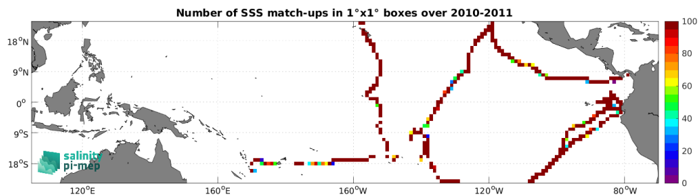
Figure 5: Number of SSS match-ups between TSG (GOSUD-Sailing-ship) SSS and the CCI SSS L4 Merged-OI v5.5 - 7-day running (ESA) SSS product for the Tropical Pacific Ocean Pi-MEP region over 1^\circ \times 1^\circ boxes and for the full satellite product period.
