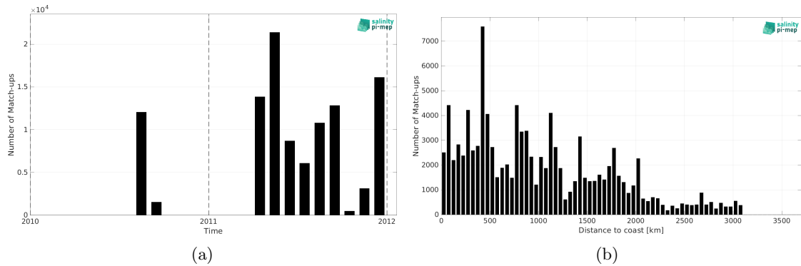
Figure 2: Number of match-ups between TSG (GOSUD-Sailing-ship) and CCI SSS L4 Merged-OI v5.5 - 7-day running (ESA) SSS as a function of time (a) and as function of the distance to coast (b) over the Tropical Pacific Ocean Pi-MEP region and for the full satellite product period.
