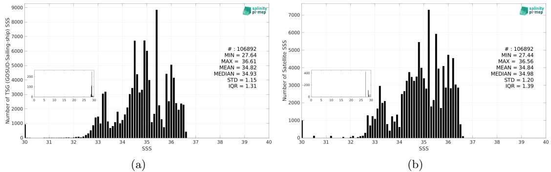
Figure 3: Histograms of SSS from TSG (GOSUD-Sailing-ship) (a) and CCI SSS L4 Merged-OI v5.5 - 7-day running (ESA) (b) considering all match-up pairs per bins of 0.1 over the Tropical Pacific Ocean Pi-MEP region and for the full satellite product period.
