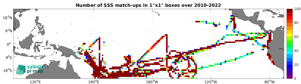
Figure 5: Number of SSS match-ups between TSG (GOSUD-Research-vessel) SSS and the CCI SSS L4 Merged-OI v5.5 - 7-day running (ESA) SSS product for the Tropical Pacific Ocean Pi-MEP region over 1^\circ \times 1^\circ boxes and for the full satellite product period.
