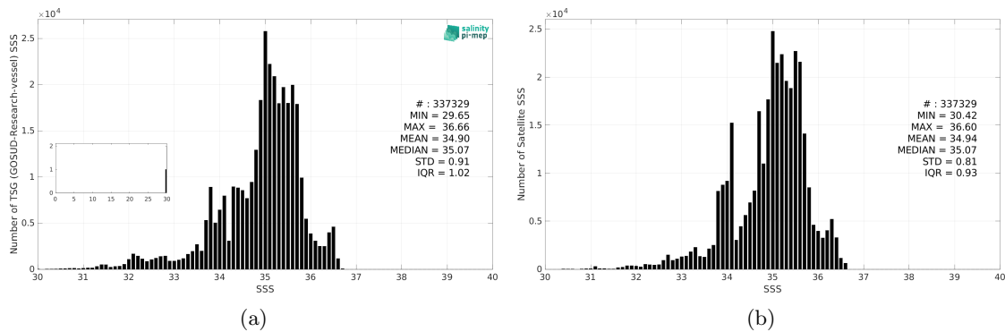
Figure 3: Histograms of SSS from TSG (GOSUD-Research-vessel) (a) and CCI SSS L4 Merged-OI v5.5 - 7-day running (ESA) (b) considering all match-up pairs per bins of 0.1 over the Tropical Pacific Ocean Pi-MEP region and for the full satellite product period.
