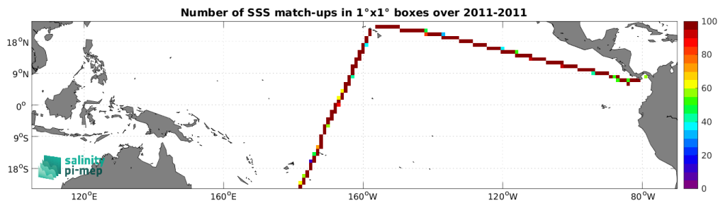
Figure 5: Number of SSS match-ups between TSG (CSIC-UTM) SSS and the CCI SSS L4 Merged-OI v5.5 - 7-day running (ESA) SSS product for the Tropical Pacific Ocean Pi-MEP region over 1^\circ \times 1^\circ boxes and for the full satellite product period.
