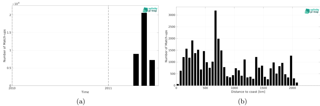
Figure 2: Number of match-ups between TSG (CSIC-UTM) and CCI SSS L4 Merged-OI v5.5 - 7-day running (ESA) SSS as a function of time (a) and as function of the distance to coast (b) over the Tropical Pacific Ocean Pi-MEP region and for the full satellite product period.
