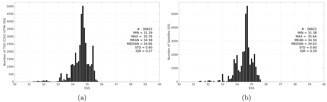
Figure 3: Histograms of SSS from TSG (CSIC-UTM) (a) and CCI SSS L4 Merged-OI v5.5 - 7-day running (ESA) (b) considering all match-up pairs per bins of 0.1 over the Tropical Pacific Ocean Pi-MEP region and for the full satellite product period.
