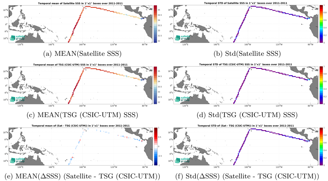
Figure 7: Temporal mean (left) and Std (right) of SSS from CCI SSS L4 Merged-OI v5.5 - 7-day running (ESA) (top), TSG (CSIC-UTM) (middle), and of \Delta SSS (Satellite - TSG (CSIC-UTM)). Only match-up pairs are used to generate these maps.
