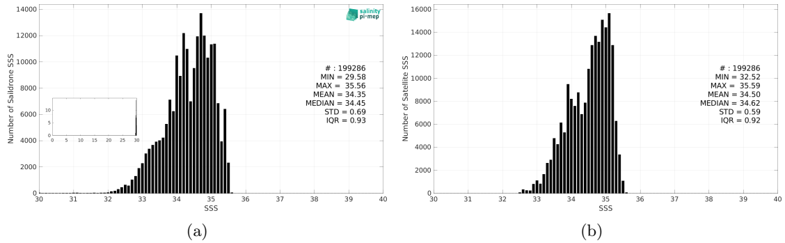
Figure 3: Histograms of SSS from Saildrone (a) and CCI SSS L4 Merged-OI v5.5 - 7-day running (ESA) (b) considering all match-up pairs per bins of 0.1 over the Tropical Pacific Ocean Pi-MEP region and for the full satellite product period.
