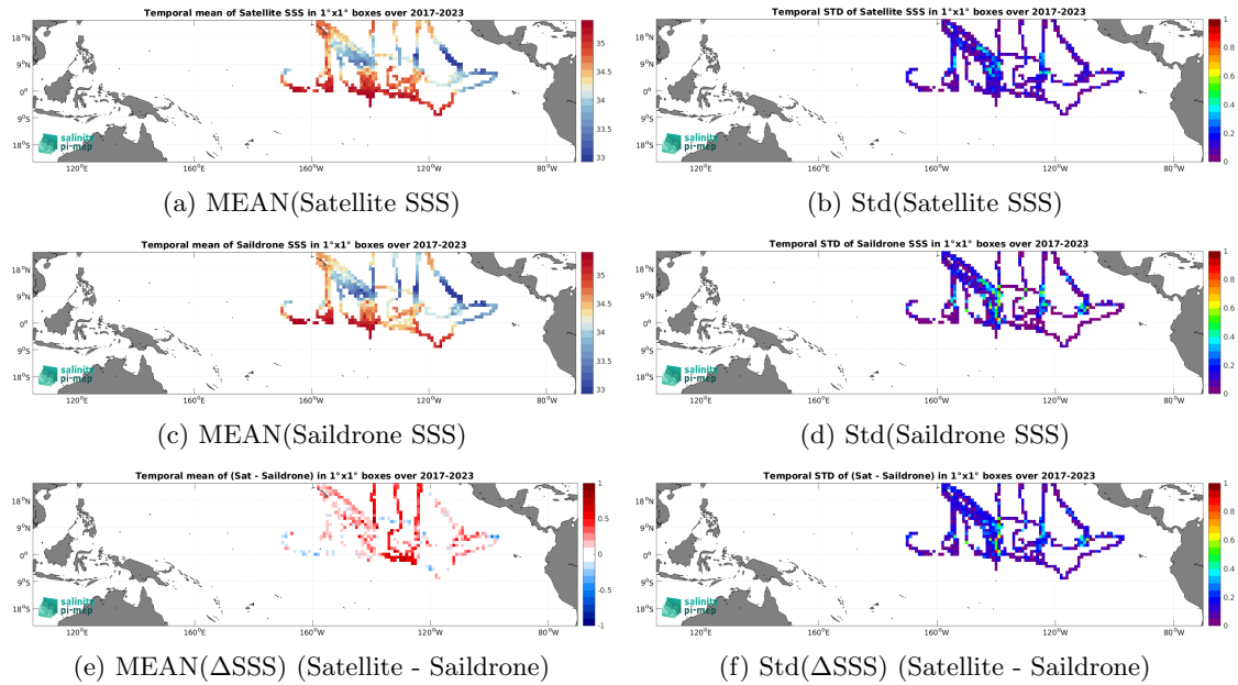
Figure 7: Temporal mean (left) and Std (right) of SSS from CCI SSS L4 Merged-OI v5.5 - 7-day running (ESA) (top), Saildrone (middle), and of \Delta SSS (Satellite - Saildrone). Only match-up pairs are used to generate these maps.
