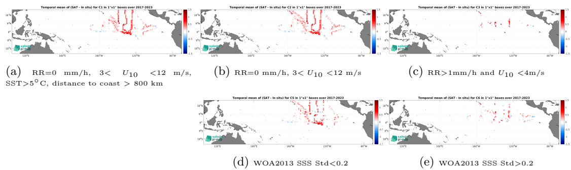
Figure 14: Temporal mean gridded over spatial boxes of size 1^\circ \times 1^\circ of \Delta\text{SSS} (CCI SSS L4 Merged-OI v5.5 - 7-day running (ESA) - Saildrone) for 5 different subdatasets corresponding to: RR=0 mm/h, 3 < U_{10} < 12 m/s, SST > 5°C, distance to coast > 800 km (a), RR=0 mm/h, 3 < U_{10} < 12 m/s (b), RR > 1mm/h and U_{10} < 4 m/s (c), WOA2013 SSS Std < 0.2 (d), WOA2013 SSS Std > 0.2 (e).
