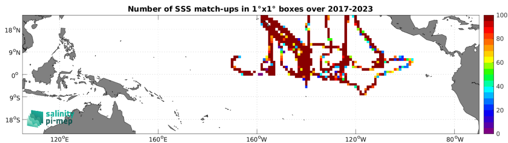
Figure 5: Number of SSS match-ups between Saildrone SSS and the CCI SSS L4 Merged-OI v5.5 - 7-day running (ESA) SSS product for the Tropical Pacific Ocean Pi-MEP region over 1^\circ \times 1^\circ boxes and for the full satellite product period.
