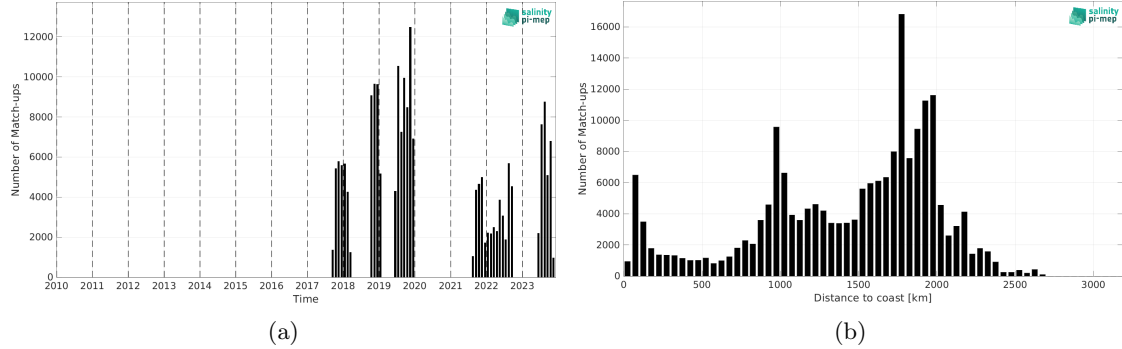
Figure 2: Number of match-ups between Saildrone and CCI SSS L4 Merged-OI v5.5 - 7-day running (ESA) SSS as a function of time (a) and as function of the distance to coast (b) over the Tropical Pacific Ocean Pi-MEP region and for the full satellite product period.
