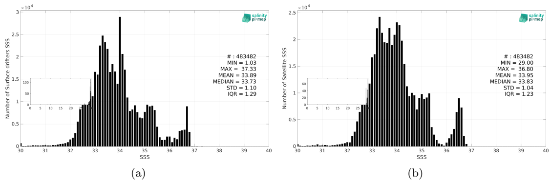
Figure 3: Histograms of SSS from Surface drifters (a) and CCI SSS L4 Merged-OI v5.5 - 7-day running (ESA) (b) considering all match-up pairs per bins of 0.1 over the Tropical Pacific Ocean Pi-MEP region and for the full satellite product period.
