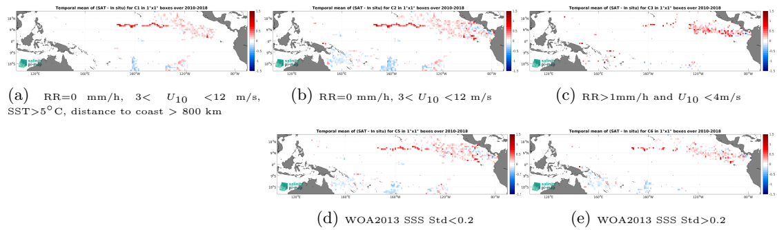
Figure 13: Temporal mean gridded over spatial boxes of size 1^\circ \times 1^\circ of \Delta SSS (CCI SSS L4 Merged-OI v5.5 - 7-day running (ESA) - Surface drifters) for 5 different subdatasets corresponding to:RR=0 mm/h, 3 < U_{10} < 12 m/s, SST > 5^\circ\text{C} , distance to coast > 800 km (a), RR=0 mm/h, 3 < U_{10} < 12 m/s (b), RR > 1 mm/h and U_{10} < 4 m/s (c), WOA2013 SSS Std < 0.2 (d), WOA2013 SSS Std > 0.2 (e).
