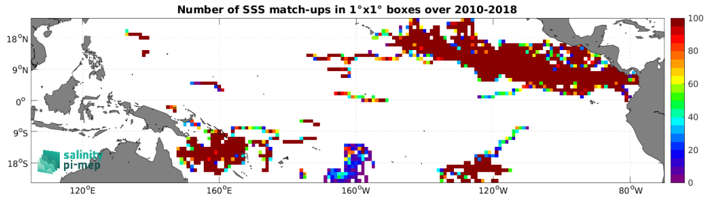
Figure 4: Number of SSS match-ups between Surface drifters SSS and the CCI SSS L4 Merged-OI v5.5 - 7-day running (ESA) SSS product for the Tropical Pacific Ocean Pi-MEP region over 1^\circ \times 1^\circ boxes and for the full satellite product period.
