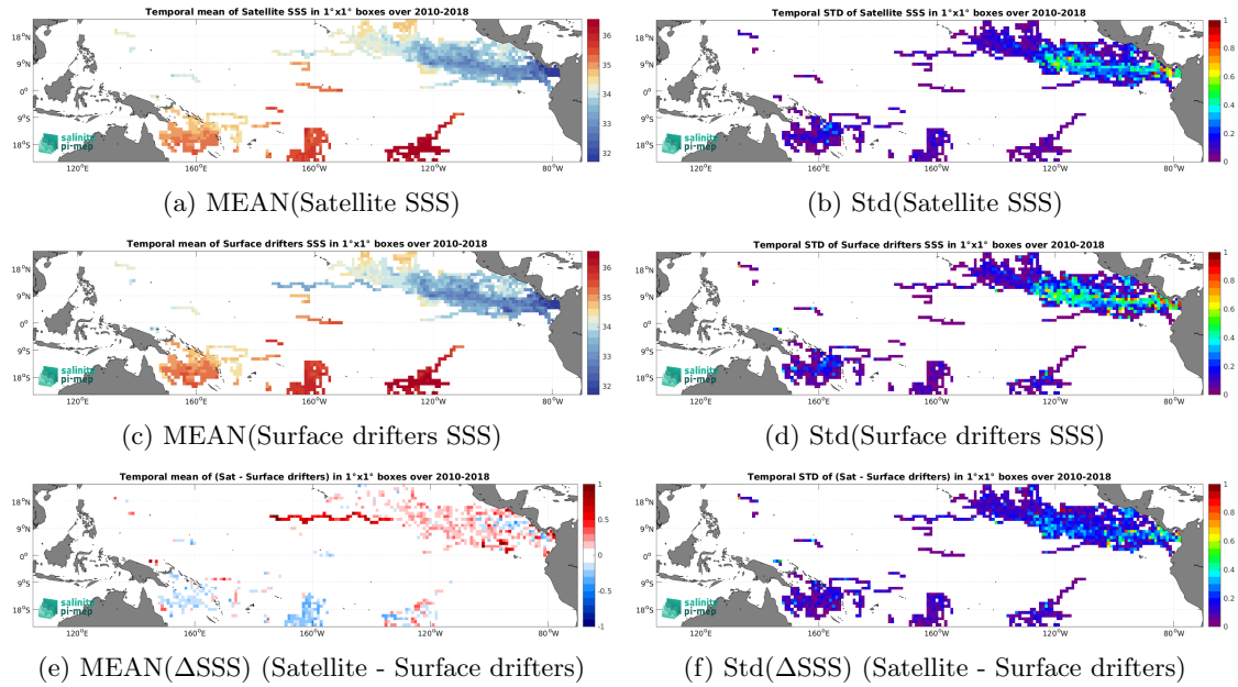
Figure 6: Temporal mean (left) and Std (right) of SSS from CCI SSS L4 Merged-OI v5.5 - 7-day running (ESA) (top), Surface drifters (middle), and of \Delta SSS (Satellite - Surface drifters). Only match-up pairs are used to generate these maps.
