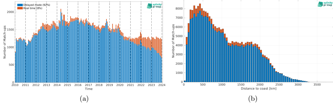
Figure 2: Number of match-ups between Argo and CCI SSS L4 Merged-OI v5.5 - 7-day running (ESA) SSS as a function of time (a) and as function of the distance to coast (b) over the Tropical Pacific Ocean Pi-MEP region and for the full satellite product period.
