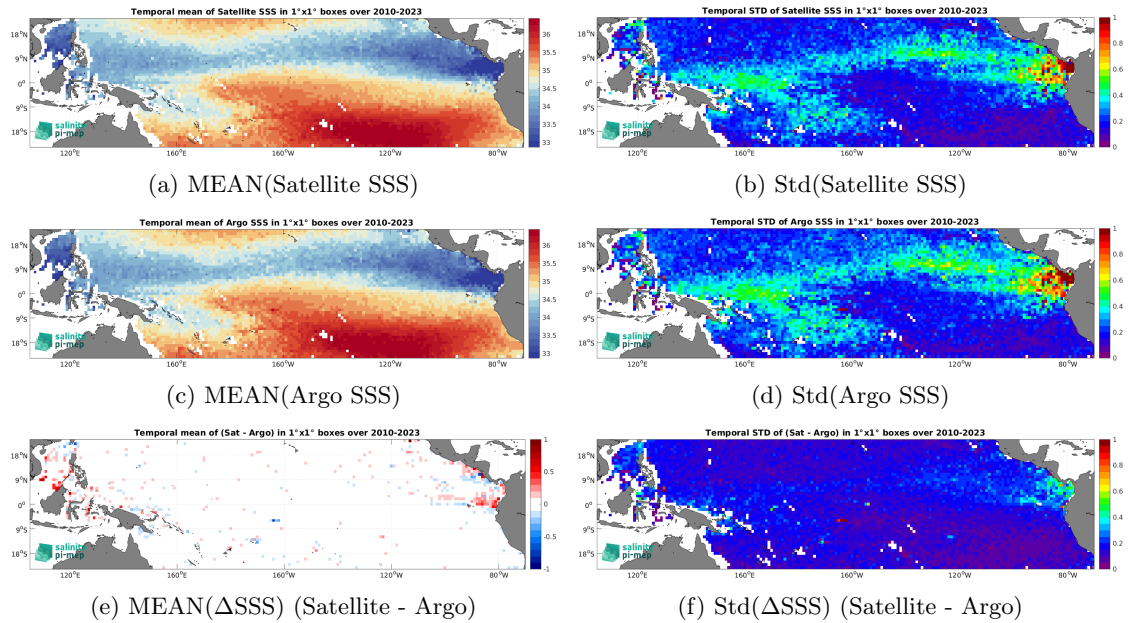
Figure 7: Temporal mean (left) and Std (right) of SSS from CCI SSS L4 Merged-OI v5.5 - 7-day running (ESA) (top), Argo (middle), and of \Delta SSS (Satellite - Argo). Only match-up pairs are used to generate these maps.
