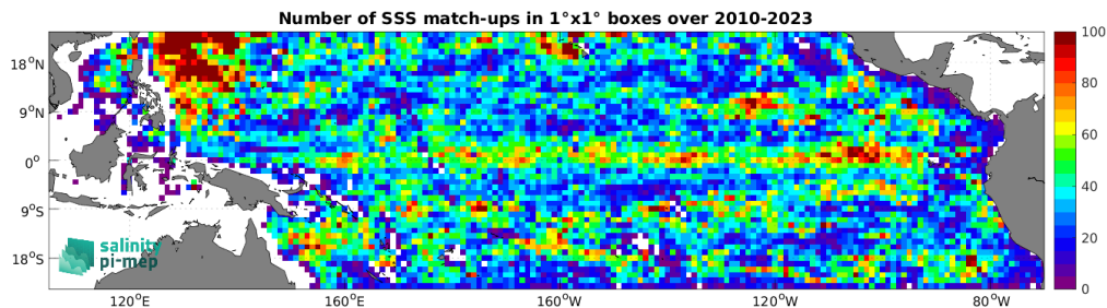
Figure 5: Number of SSS match-ups between Argo SSS and the CCI SSS L4 Merged-OI v5.5 - 7-day running (ESA) SSS product for the Tropical Pacific Ocean Pi-MEP region over 1^\circ \times 1^\circ boxes and for the full satellite product period.
