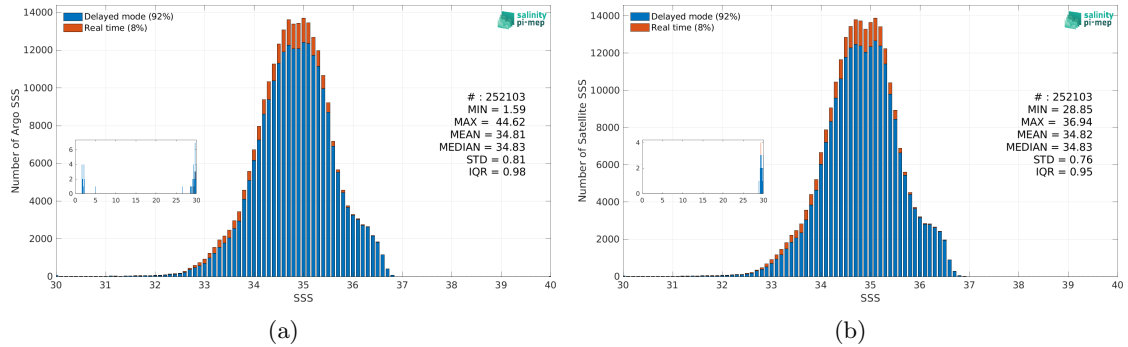
Figure 3: Histograms of SSS from Argo (a) and CCI SSS L4 Merged-OI v5.5 - 7-day running (ESA) (b) considering all match-up pairs per bins of 0.1 over the Tropical Pacific Ocean Pi-MEP region and for the full satellite product period.
