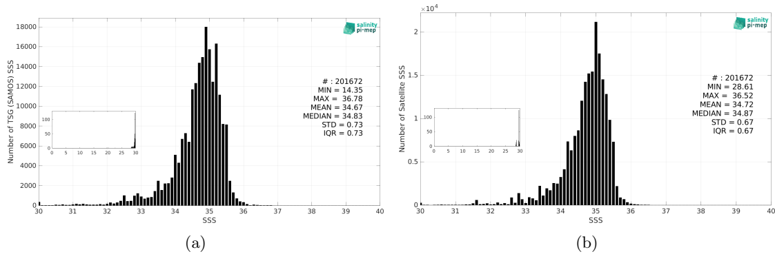
Figure 3: Histograms of SSS from TSG (SAMOS) (a) and CCI SSS L4 Merged-OI v5.5 - 30-day running (ESA) (b) considering all match-up pairs per bins of 0.1 over the Tropical Pacific Ocean Pi-MEP region and for the full satellite product period.
