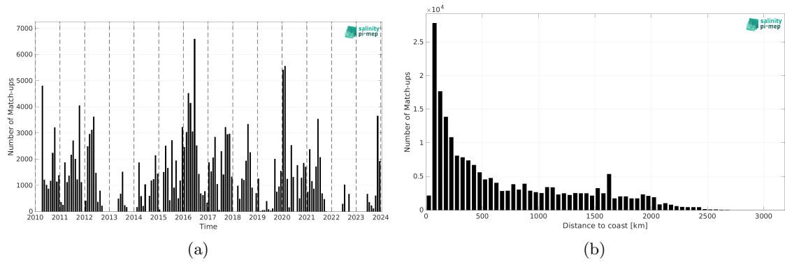
Figure 2: Number of match-ups between TSG (SAMOS) and CCI SSS L4 Merged-OI v5.5 - 30-day running (ESA) SSS as a function of time (a) and as function of the distance to coast (b) over the Tropical Pacific Ocean Pi-MEP region and for the full satellite product period.
