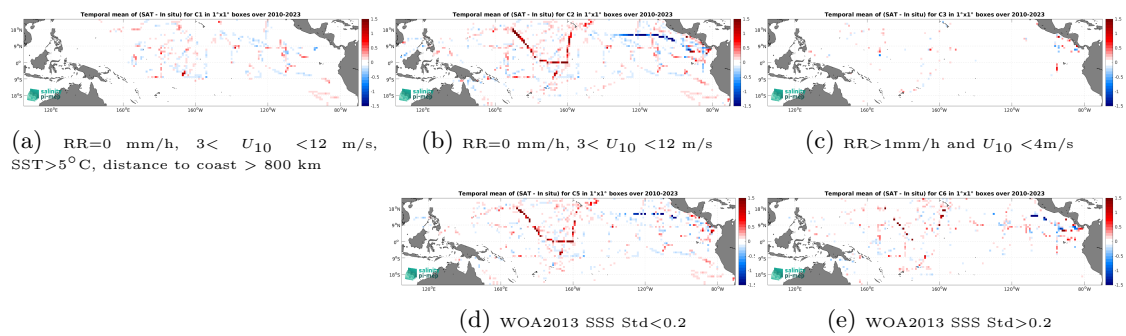
Figure 14: Temporal mean gridded over spatial boxes of size 1^\circ \times 1^\circ of \Delta SSS (CCI SSS L4 Merged-OI v5.5 - 30-day running (ESA) - TSG (SAMOS)) for 5 different subdatasets corresponding to:RR=0 mm/h, 3 < U_{10} < 12 m/s, SST >5^\circ C, distance to coast > 800 km (a), RR=0 mm/h, 3 < U_{10} < 12 m/s (b), RR >1 mm/h and U_{10} < 4 m/s (c), WOA2013 SSS Std <0.2 (d), WOA2013 SSS Std >0.2 (e).
