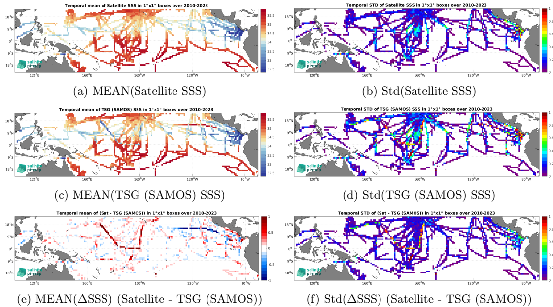
Figure 7: Temporal mean (left) and Std (right) of SSS from CCI SSS L4 Merged-OI v5.5 - 30-day running (ESA) (top), TSG (SAMOS) (middle), and of \Delta SSS (Satellite - TSG (SAMOS)). Only match-up pairs are used to generate these maps.
