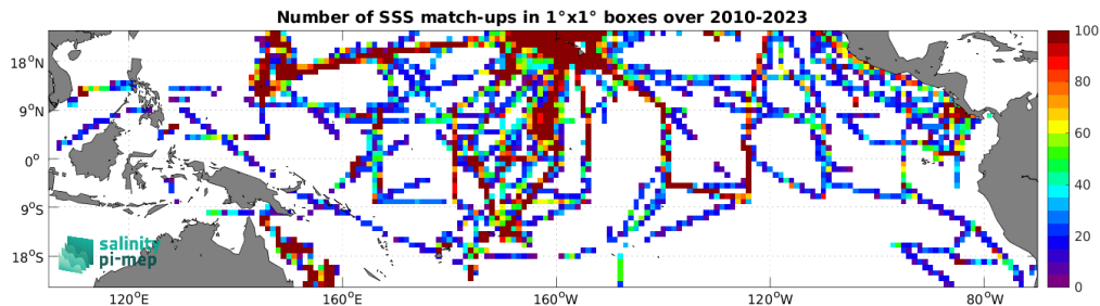
Figure 5: Number of SSS match-ups between TSG (SAMOS) SSS and the CCI SSS L4 Merged-OI v5.5 - 30-day running (ESA) SSS product for the Tropical Pacific Ocean Pi-MEP region over 1^\circ \times 1^\circ boxes and for the full satellite product period.
