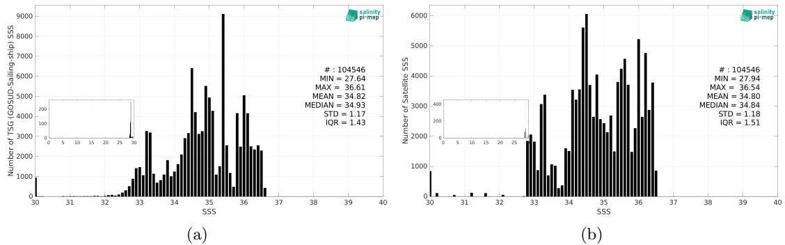
Figure 3: Histograms of SSS from TSG (GOSUD-Sailing-ship) (a) and CCI SSS L4 Merged-OI v5.5 - 30-day running (ESA) (b) considering all match-up pairs per bins of 0.1 over the Tropical Pacific Ocean Pi-MEP region and for the full satellite product period.
