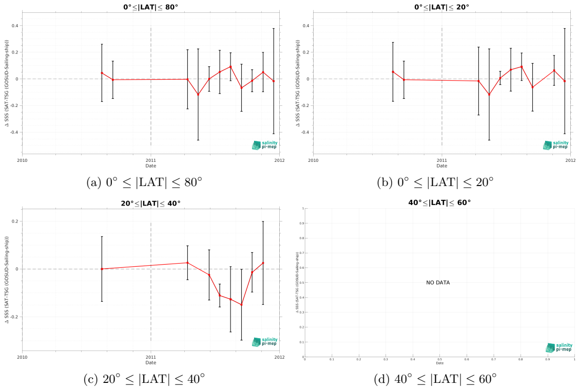
Figure 11: Monthly median (red curves) of \Delta SSS (Satellite - in situ ) between CCI SSS L4 Merged-OI v5.5 - 30-day running (ESA) and TSG (GOSUD-Sailing-ship) SSS as function of time for all the collected Pi-MEP match-up pairs estimated over the Tropical Pacific Ocean Pi-MEP region and for the full satellite product period are shown for different latitude bands: (a) 80^\circ\text{S}-80^\circ\text{N} , (b) 20^\circ\text{S}-20^\circ\text{N} , (c) 40^\circ\text{S}-20^\circ\text{S} and 20^\circ\text{N}-40^\circ\text{N} and (d) 60^\circ\text{S}-40^\circ\text{S} and 40^\circ\text{N}-60^\circ\text{N} .
