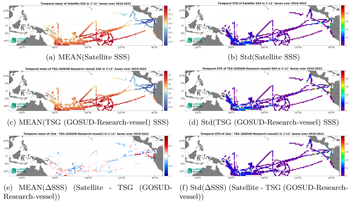
Figure 7: Temporal mean (left) and Std (right) of SSS from CCI SSS L4 Merged-OI v5.5 - 30-day running (ESA) (top), TSG (GOSUD-Research-vessel) (middle), and of \Delta SSS (Satellite - TSG (GOSUD-Research-vessel)). Only match-up pairs are used to generate these maps.
