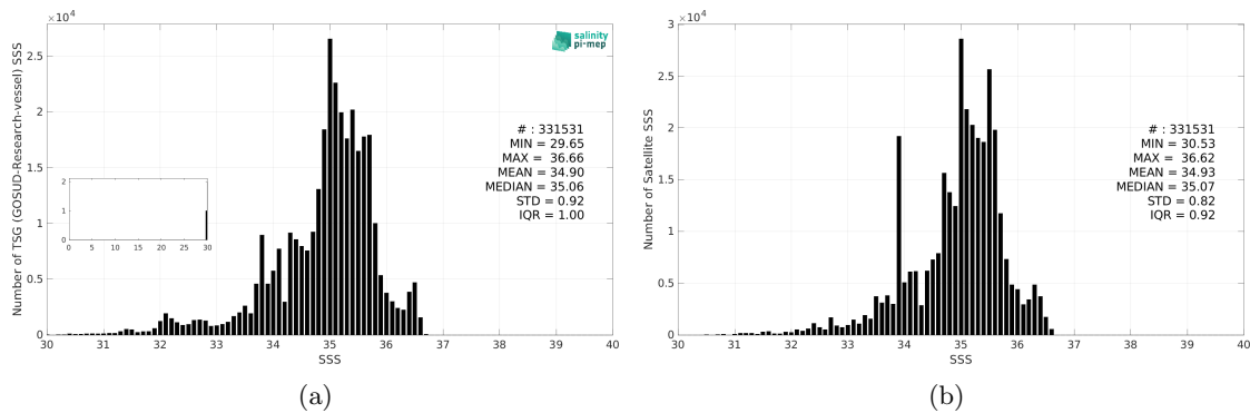
Figure 3: Histograms of SSS from TSG (GOSUD-Research-vessel) (a) and CCI SSS L4 Merged-OI v5.5 - 30-day running (ESA) (b) considering all match-up pairs per bins of 0.1 over the Tropical Pacific Ocean Pi-MEP region and for the full satellite product period.
