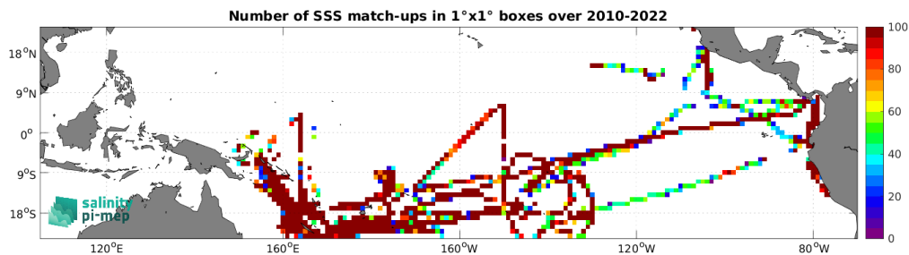
Figure 5: Number of SSS match-ups between TSG (GOSUD-Research-vessel) SSS and the CCI SSS L4 Merged-OI v5.5 - 30-day running (ESA) SSS product for the Tropical Pacific Ocean Pi-MEP region over 1°x1° boxes and for the full satellite product period.
