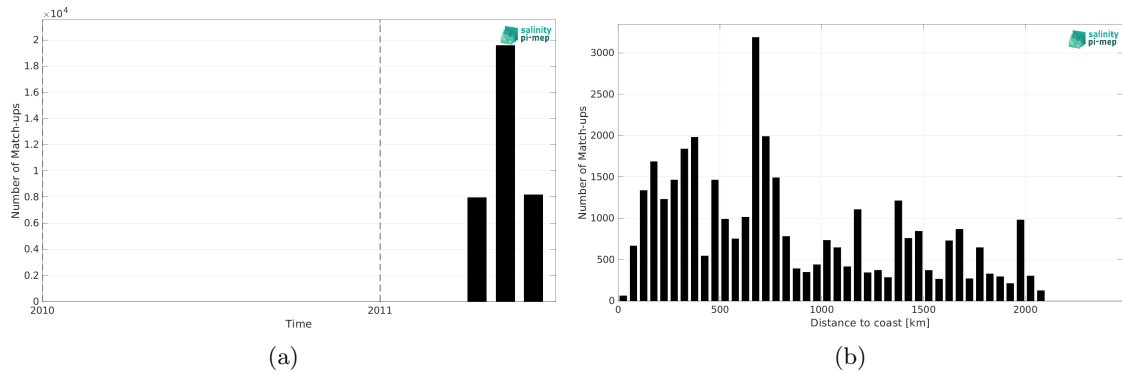
Figure 2: Number of match-ups between TSG (CSIC-UTM) and CCI SSS L4 Merged-OI v5.5 - 30-day running (ESA) SSS as a function of time (a) and as function of the distance to coast (b) over the Tropical Pacific Ocean Pi-MEP region and for the full satellite product period.
