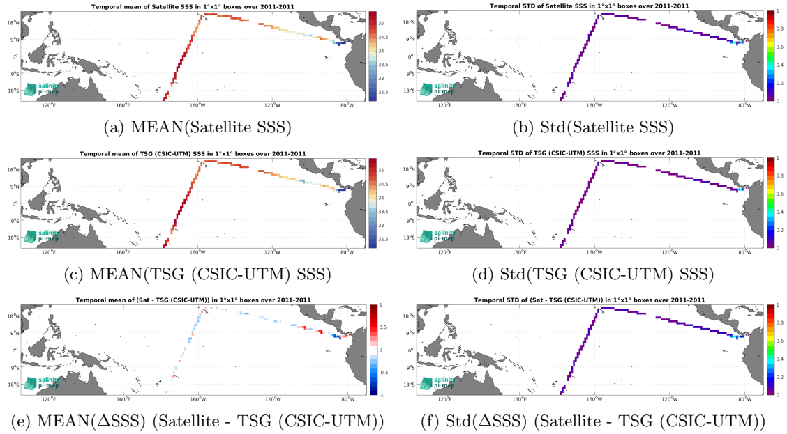
Figure 7: Temporal mean (left) and Std (right) of SSS from CCI SSS L4 Merged-OI v5.5 - 30-day running (ESA) (top), TSG (CSIC-UTM) (middle), and of \Delta SSS (Satellite - TSG (CSIC-UTM)). Only match-up pairs are used to generate these maps.
