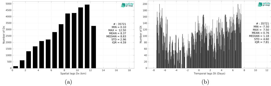
Figure 6: Histograms of the spatial (a) and temporal (b) lags between the location/time of the TSG (CSIC-UTM) measurement and the date of the corresponding CCI SSS L4 Merged-OI v5.5 - 30-day running (ESA) SSS pixel.
