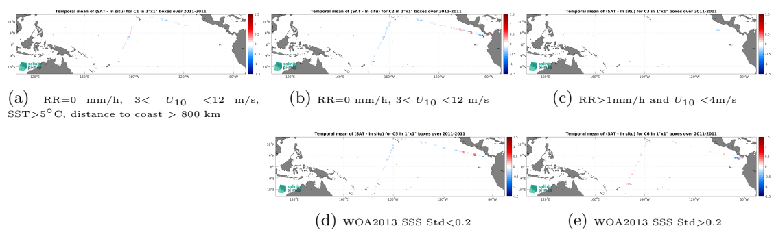
Figure 14: Temporal mean gridded over spatial boxes of size 1^\circ \times 1^\circ of \Delta SSS (CCI SSS L4 Merged-OI v5.5 - 30-day running (ESA) - TSG (CSIC-UTM)) for 5 different subdatasets corresponding to:RR=0 mm/h, 3 < U_{10} < 12 m/s, SST > 5^\circ\text{C} , distance to coast > 800 km (a), RR=0 mm/h, 3 < U_{10} < 12 m/s (b), RR > 1 mm/h and U_{10} < 4 m/s (c), WOA2013 SSS Std < 0.2 (d), WOA2013 SSS Std > 0.2 (e).
