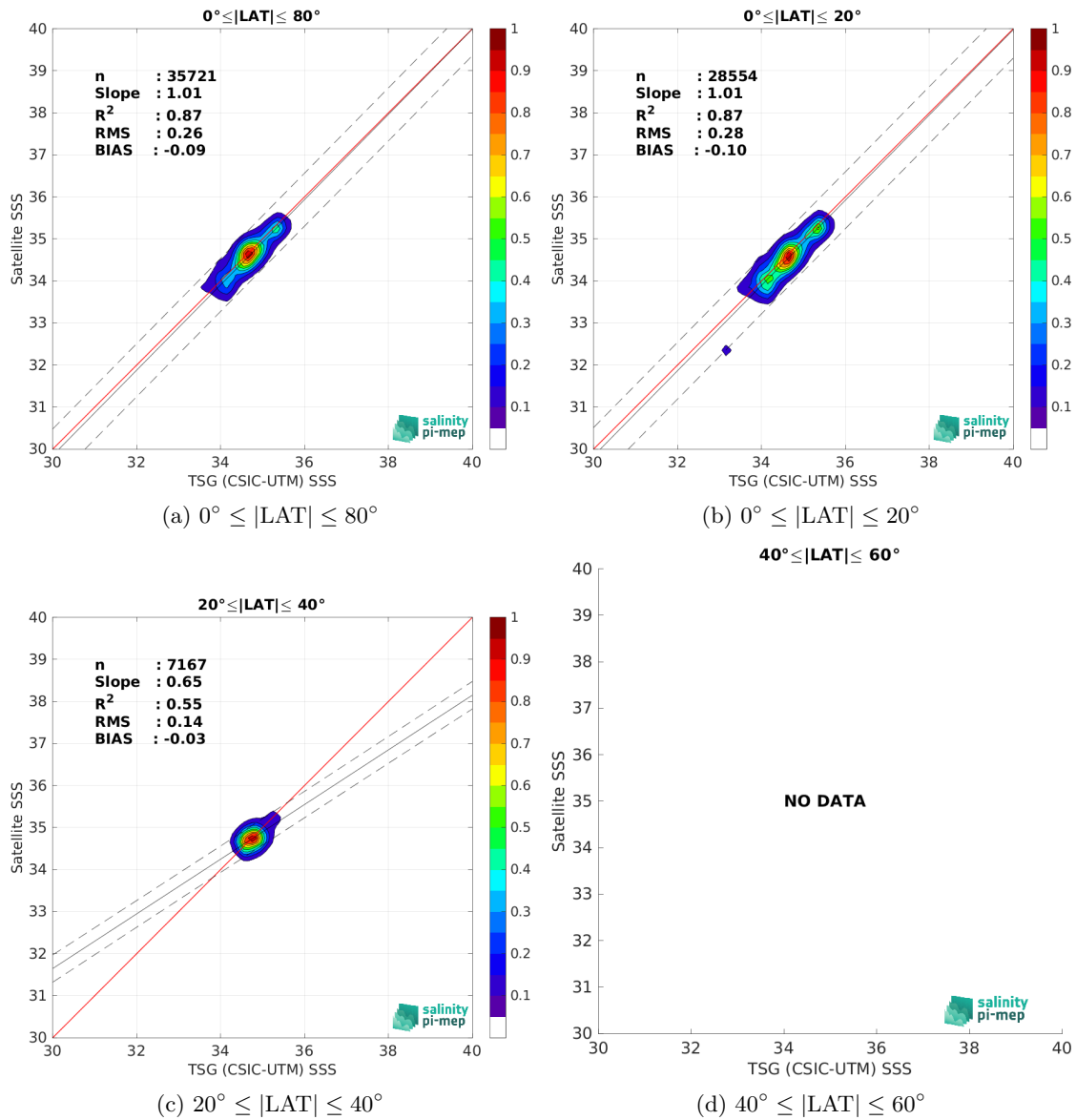
Figure 10: Contour maps of the concentration of CCI SSS L4 Merged-OI v5.5 - 30-day running (ESA) SSS (y-axis) versus TSG (CSIC-UTM) SSS (x-axis) at match-up pairs for different latitude bands. For each plot, the red line shows x=y . The black thin and dashed lines indicate a linear fit through the data cloud and the \pm 95\% confidence levels, respectively. The number match-up pairs n , the slope and R^2 coefficient of the linear fit, the root mean square (RMS) and the mean bias between satellite and in situ data are indicated for each latitude band in each plots.
