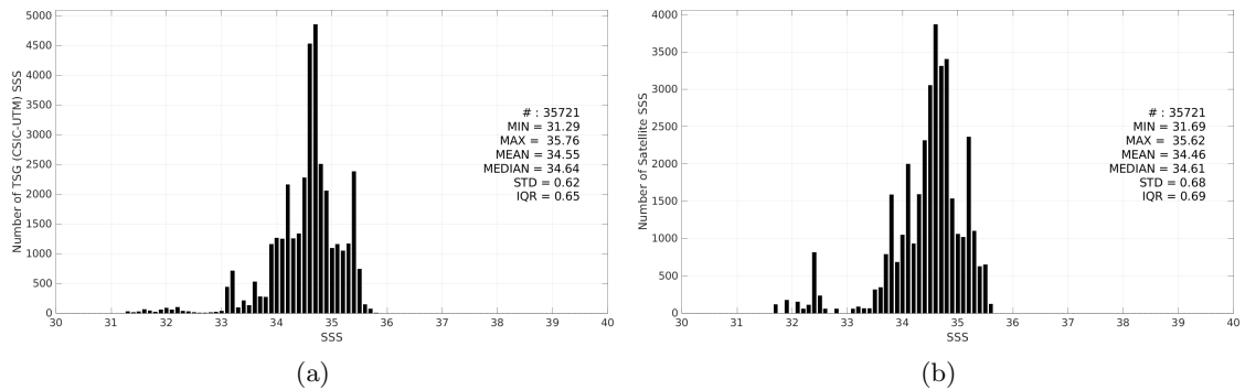
Figure 3: Histograms of SSS from TSG (CSIC-UTM) (a) and CCI SSS L4 Merged-OI v5.5 - 30-day running (ESA) (b) considering all match-up pairs per bins of 0.1 over the Tropical Pacific Ocean Pi-MEP region and for the full satellite product period.
