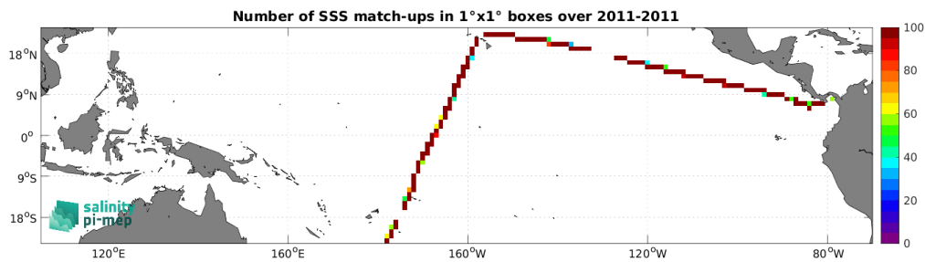
Figure 5: Number of SSS match-ups between TSG (CSIC-UTM) SSS and the CCI SSS L4 Merged-OI v5.5 - 30-day running (ESA) SSS product for the Tropical Pacific Ocean Pi-MEP region over 1^\circ \times 1^\circ boxes and for the full satellite product period.
