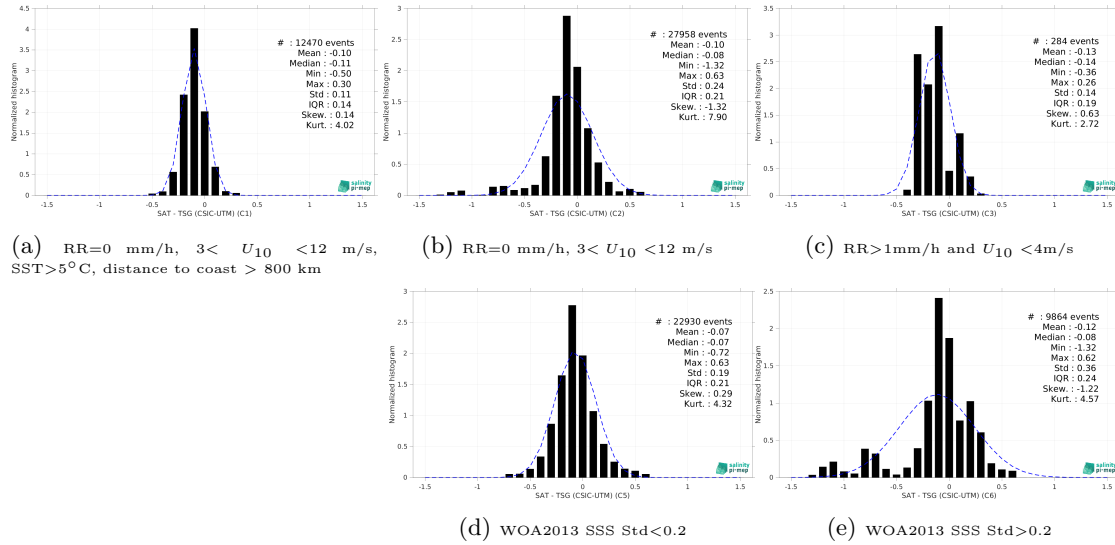
Figure 15: Normalized histogram of \Delta SSS (CCI SSS L4 Merged-OI v5.5 - 30-day running (ESA) - TSG (CSIC-UTM)) for 5 different subdatasets corresponding to: RR=0 mm/h, 3 < U_{10} < 12 m/s, SST>5°C, distance to coast > 800 km (a), RR=0 mm/h, 3 < U_{10} < 12 m/s (b), RR>1mm/h and U_{10} < 4 m/s (c), WOA2013 SSS Std<0.2 (d), WOA2013 SSS Std>0.2 (e).
