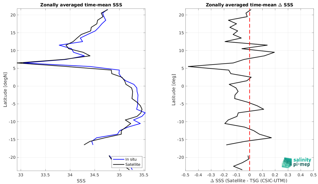
Figure 9: Left panel: Zonal mean SSS from CCI SSS L4 Merged-OI v5.5 - 30-day running (ESA) satellite product (black) and from TSG (CSIC-UTM) (blue). Right panel: Zonal mean of \Delta SSS (Satellite - TSG (CSIC-UTM)) for all the collected Pi-MEP match-up pairs estimated over the full satellite product period.
