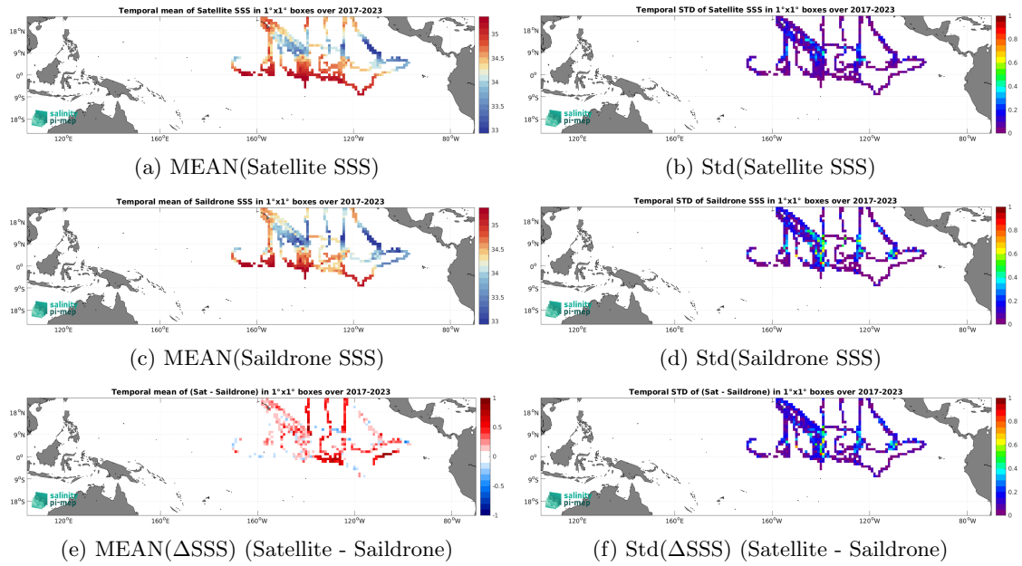
Figure 7: Temporal mean (left) and Std (right) of SSS from CCI SSS L4 Merged-OI v5.5 - 30-day running (ESA) (top), Saildrone (middle), and of \Delta SSS (Satellite - Saildrone). Only match-up pairs are used to generate these maps.
