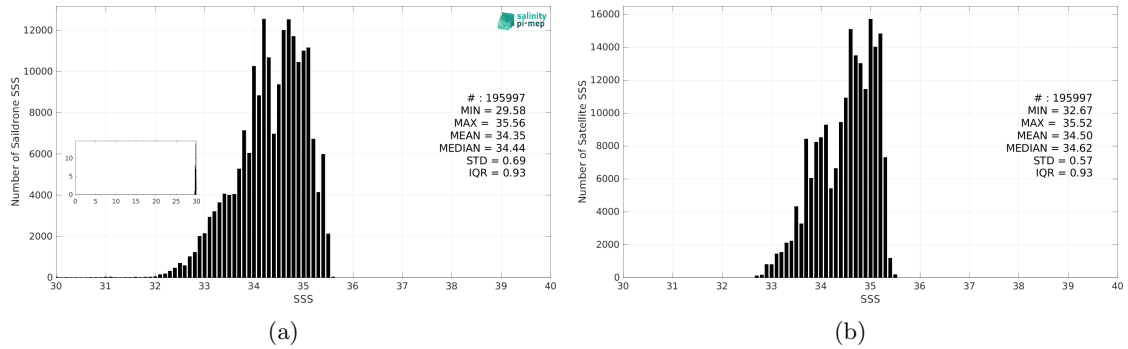
Figure 3: Histograms of SSS from Saildrone (a) and CCI SSS L4 Merged-OI v5.5 - 30-day running (ESA) (b) considering all match-up pairs per bins of 0.1 over the Tropical Pacific Ocean Pi-MEP region and for the full satellite product period.
