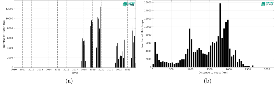
Figure 2: Number of match-ups between Saildrone and CCI SSS L4 Merged-OI v5.5 - 30-day running (ESA) SSS as a function of time (a) and as function of the distance to coast (b) over the Tropical Pacific Ocean Pi-MEP region and for the full satellite product period.
