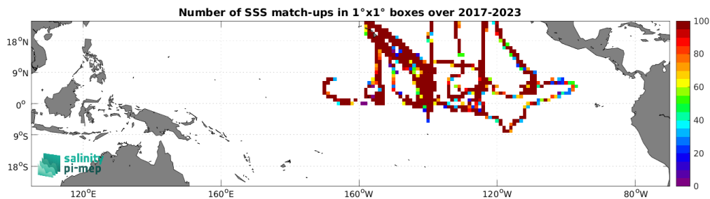
Figure 5: Number of SSS match-ups between Saildrone SSS and the CCI SSS L4 Merged-OI v5.5 - 30-day running (ESA) SSS product for the Tropical Pacific Ocean Pi-MEP region over 1^\circ \times 1^\circ boxes and for the full satellite product period.
