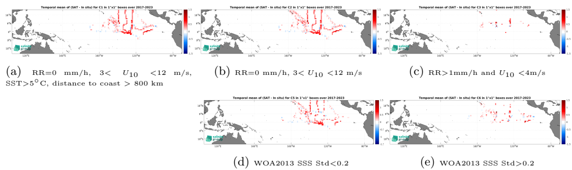
Figure 14: Temporal mean gridded over spatial boxes of size 1^\circ \times 1^\circ of \Delta SSS (CCI SSS L4 Merged-OI v5.5 - 30-day running (ESA) - Saildrone) for 5 different subdatasets corresponding to: RR=0 mm/h, 3 < U_{10} < 12 m/s, SST > 5^\circ\text{C} , distance to coast > 800 km (a), RR=0 mm/h, 3 < U_{10} < 12 m/s (b), RR > 1 mm/h and U_{10} < 4 m/s (c), WOA2013 SSS Std < 0.2 (d), WOA2013 SSS Std > 0.2 (e).
