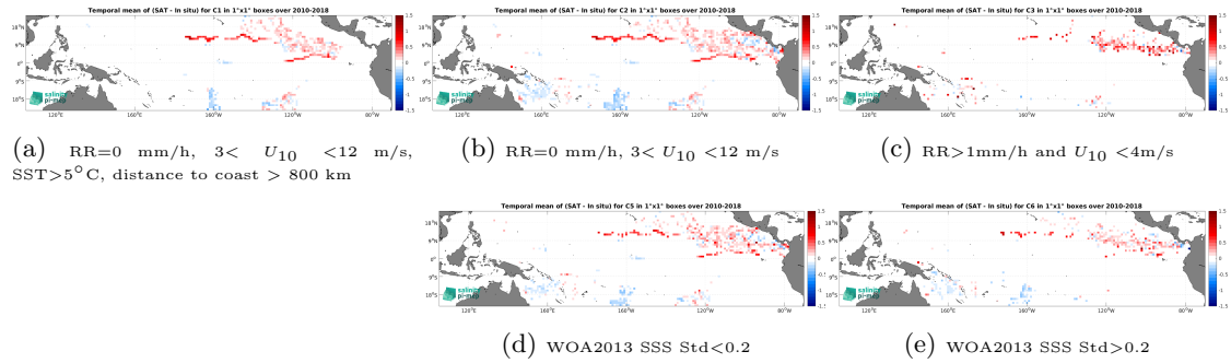
Figure 13: Temporal mean gridded over spatial boxes of size 1^\circ \times 1^\circ of \Delta SSS (CCI SSS L4 Merged-OI v5.5 - 30-day running (ESA) - Surface drifters) for 5 different subdatasets corresponding to:RR=0 mm/h, 3 < U_{10} < 12 m/s, SST > 5^\circ\text{C} , distance to coast > 800 km (a), RR=0 mm/h, 3 < U_{10} < 12 m/s (b), RR > 1 mm/h and U_{10} < 4 m/s (c), WOA2013 SSS Std < 0.2 (d), WOA2013 SSS Std > 0.2 (e).
