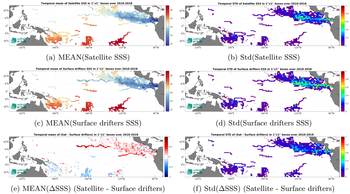
Figure 6: Temporal mean (left) and Std (right) of SSS from CCI SSS L4 Merged-OI v5.5 - 30-day running (ESA) (top), Surface drifters (middle), and of \Delta SSS (Satellite - Surface drifters). Only match-up pairs are used to generate these maps.
