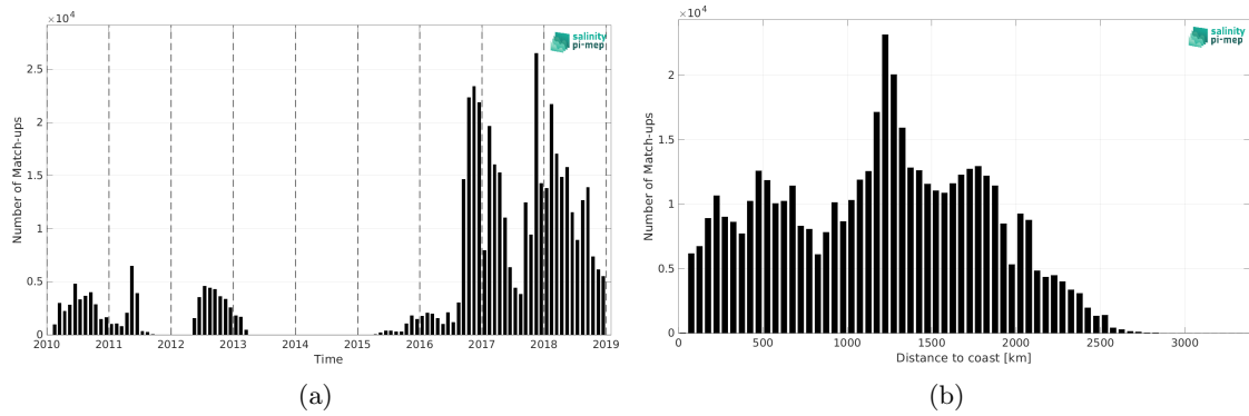
Figure 2: Number of match-ups between Surface drifters and CCI SSS L4 Merged-OI v5.5 - 30-day running (ESA) SSS as a function of time (a) and as function of the distance to coast (b) over the Tropical Pacific Ocean Pi-MEP region and for the full satellite product period.
