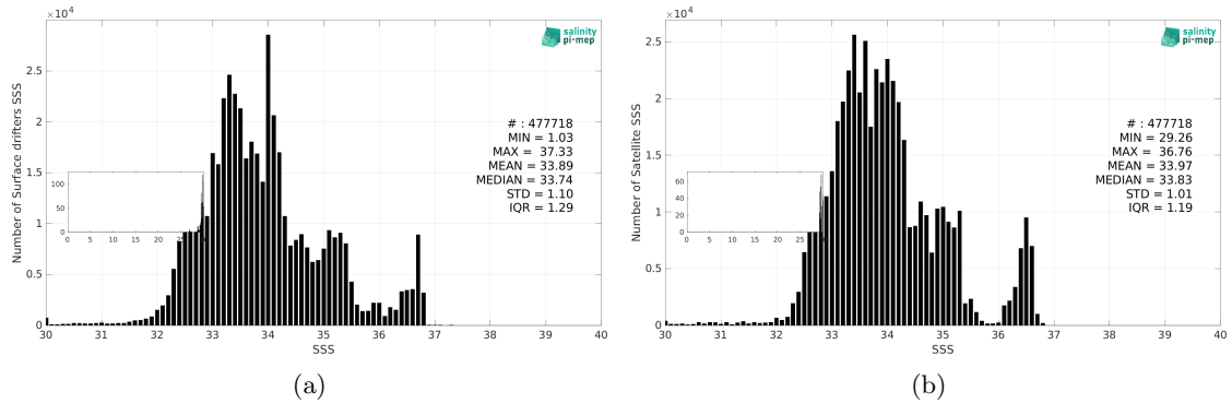
Figure 3: Histograms of SSS from Surface drifters (a) and CCI SSS L4 Merged-OI v5.5 - 30-day running (ESA) (b) considering all match-up pairs per bins of 0.1 over the Tropical Pacific Ocean Pi-MEP region and for the full satellite product period.
