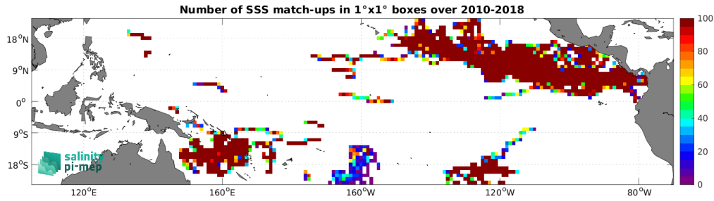
Figure 4: Number of SSS match-ups between Surface drifters SSS and the CCI SSS L4 Merged-OI v5.5 - 30-day running (ESA) SSS product for the Tropical Pacific Ocean Pi-MEP region over 1^\circ \times 1^\circ boxes and for the full satellite product period.
