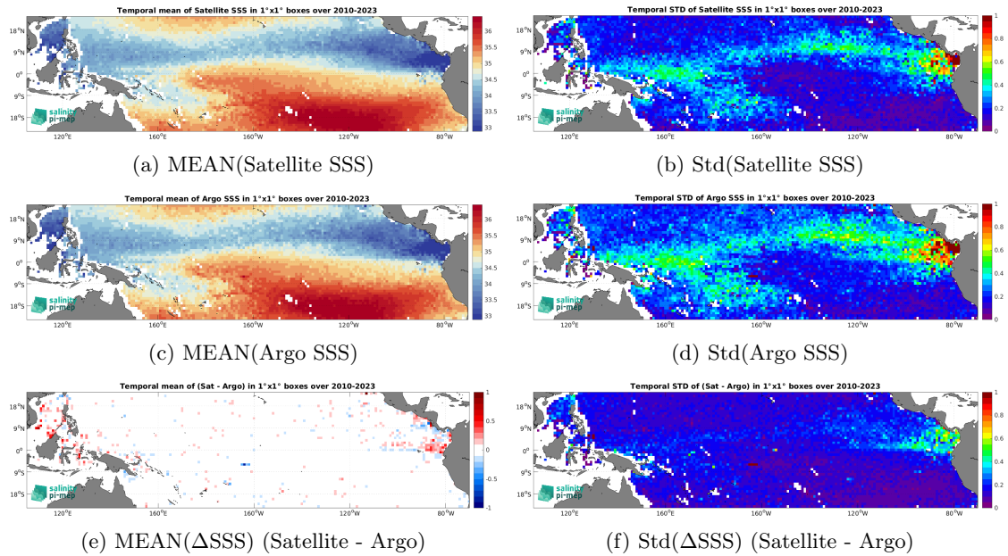
Figure 7: Temporal mean (left) and Std (right) of SSS from CCI SSS L4 Merged-OI v5.5 - 30-day running (ESA) (top), Argo (middle), and of \Delta SSS (Satellite - Argo). Only match-up pairs are used to generate these maps.
