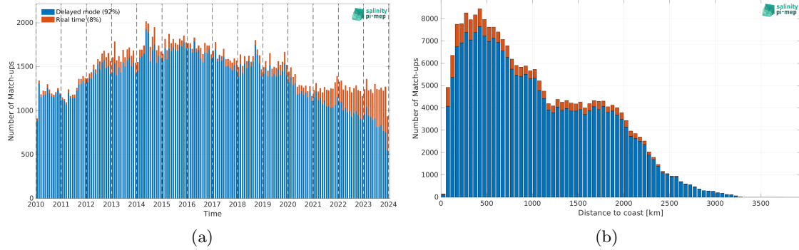
Figure 2: Number of match-ups between Argo and CCI SSS L4 Merged-OI v5.5 - 30-day running (ESA) SSS as a function of time (a) and as function of the distance to coast (b) over the Tropical Pacific Ocean Pi-MEP region and for the full satellite product period.
