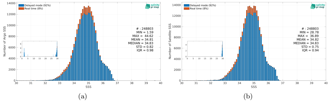
Figure 3: Histograms of SSS from Argo (a) and CCI SSS L4 Merged-OI v5.5 - 30-day running (ESA) (b) considering all match-up pairs per bins of 0.1 over the Tropical Pacific Ocean Pi-MEP region and for the full satellite product period.
