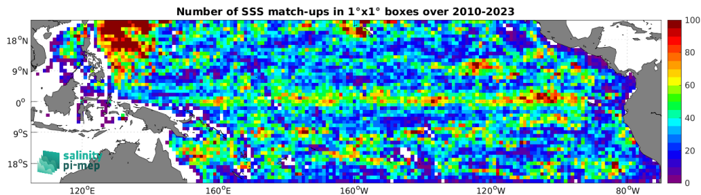
Figure 5: Number of SSS match-ups between Argo SSS and the CCI SSS L4 Merged-OI v5.5 - 30-day running (ESA) SSS product for the Tropical Pacific Ocean Pi-MEP region over 1^\circ \times 1^\circ boxes and for the full satellite product period.
