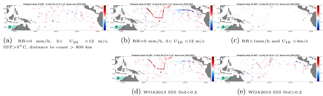
Figure 14: Temporal mean gridded over spatial boxes of size 1^\circ \times 1^\circ of \Delta SSS (CCI SSS L4 Merged-OI v4.41 - 7-day running (ESA) - TSG (SAMOS)) for 5 different subdatasets corresponding to:RR=0 mm/h, 3 < U_{10} < 12 m/s, SST >5^\circ C, distance to coast > 800 km (a), RR=0 mm/h, 3 < U_{10} < 12 m/s (b), RR >1 mm/h and U_{10} < 4 m/s (c), WOA2013 SSS Std <0.2 (d), WOA2013 SSS Std >0.2 (e).
