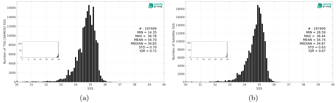
Figure 3: Histograms of SSS from TSG (SAMOS) (a) and CCI SSS L4 Merged-OI v4.41 - 7-day running (ESA) (b) considering all match-up pairs per bins of 0.1 over the Tropical Pacific Ocean Pi-MEP region and for the full satellite product period.
