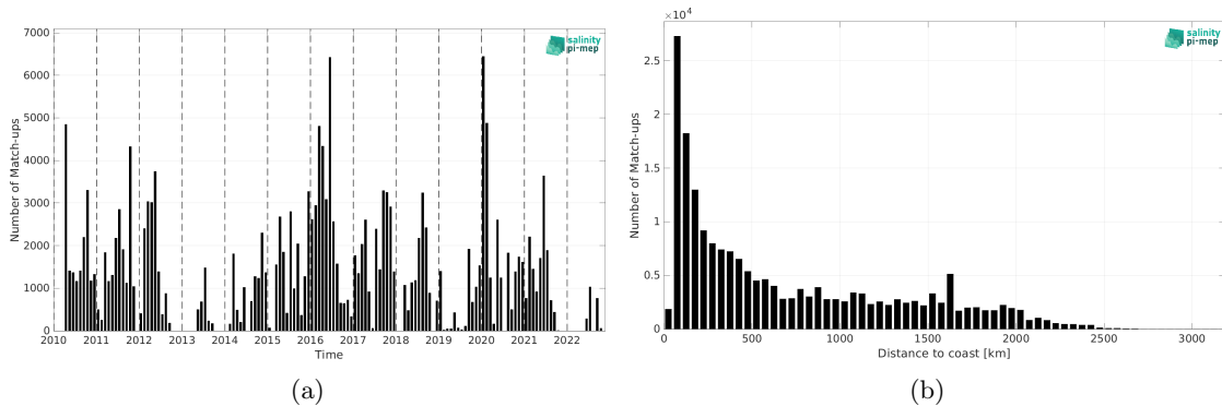
Figure 2: Number of match-ups between TSG (SAMOS) and CCI SSS L4 Merged-OI v4.41 - 7-day running (ESA) SSS as a function of time (a) and as function of the distance to coast (b) over the Tropical Pacific Ocean Pi-MEP region and for the full satellite product period.
