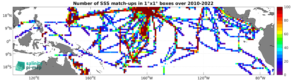
Figure 5: Number of SSS match-ups between TSG (SAMOS) SSS and the CCI SSS L4 Merged-OI v4.41 - 7-day running (ESA) SSS product for the Tropical Pacific Ocean Pi-MEP region over 1^\circ \times 1^\circ boxes and for the full satellite product period.
