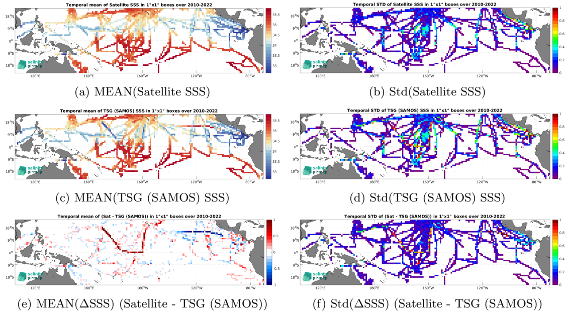
Figure 7: Temporal mean (left) and Std (right) of SSS from CCI SSS L4 Merged-OI v4.41 - 7-day running (ESA) (top), TSG (SAMOS) (middle), and of \Delta SSS (Satellite - TSG (SAMOS)). Only match-up pairs are used to generate these maps.
