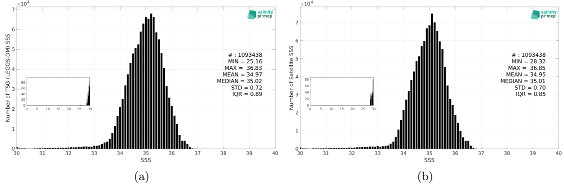
Figure 3: Histograms of SSS from TSG (LEGOS-DM) (a) and CCI SSS L4 Merged-OI v4.41 - 7-day running (ESA) (b) considering all match-up pairs per bins of 0.1 over the Tropical Pacific Ocean Pi-MEP region and for the full satellite product period.
