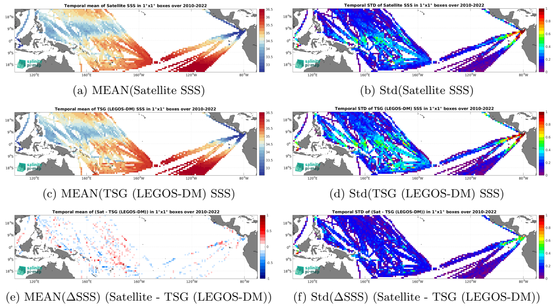
Figure 7: Temporal mean (left) and Std (right) of SSS from CCI SSS L4 Merged-OI v4.41 - 7-day running (ESA) (top), TSG (LEGOS-DM) (middle), and of \Delta SSS (Satellite - TSG (LEGOS-DM)). Only match-up pairs are used to generate these maps.
