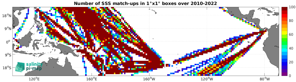
Figure 5: Number of SSS match-ups between TSG (LEGOS-DM) SSS and the CCI SSS L4 Merged-OI v4.41 - 7-day running (ESA) SSS product for the Tropical Pacific Ocean Pi-MEP region over 1^\circ \times 1^\circ boxes and for the full satellite product period.
