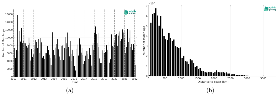
Figure 2: Number of match-ups between TSG (LEGOS-DM) and CCI SSS L4 Merged-OI v4.41 - 7-day running (ESA) SSS as a function of time (a) and as function of the distance to coast (b) over the Tropical Pacific Ocean Pi-MEP region and for the full satellite product period.
