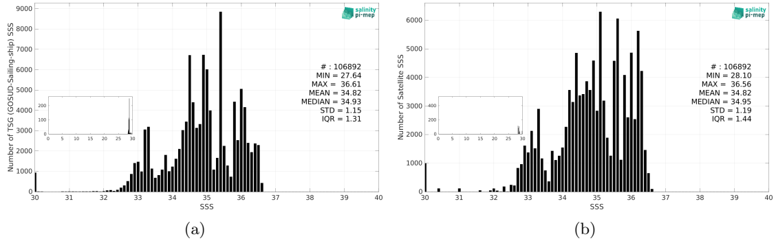
Figure 3: Histograms of SSS from TSG (GOSUD-Sailing-ship) (a) and CCI SSS L4 Merged-OI v4.41 - 7-day running (ESA) (b) considering all match-up pairs per bins of 0.1 over the Tropical Pacific Ocean Pi-MEP region and for the full satellite product period.
