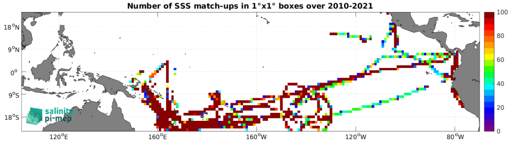
Figure 5: Number of SSS match-ups between TSG (GOSUD-Research-vessel) SSS and the CCI SSS L4 Merged-OI v4.41 - 7-day running (ESA) SSS product for the Tropical Pacific Ocean Pi-MEP region over 1^\circ \times 1^\circ boxes and for the full satellite product period.
