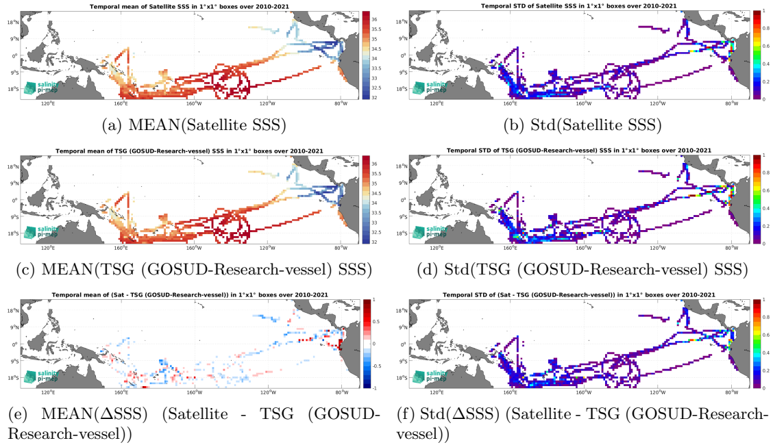
Figure 7: Temporal mean (left) and Std (right) of SSS from CCI SSS L4 Merged-OI v4.41 - 7-day running (ESA) (top), TSG (GOSUD-Research-vessel) (middle), and of \Delta SSS (Satellite - TSG (GOSUD-Research-vessel)). Only match-up pairs are used to generate these maps.
