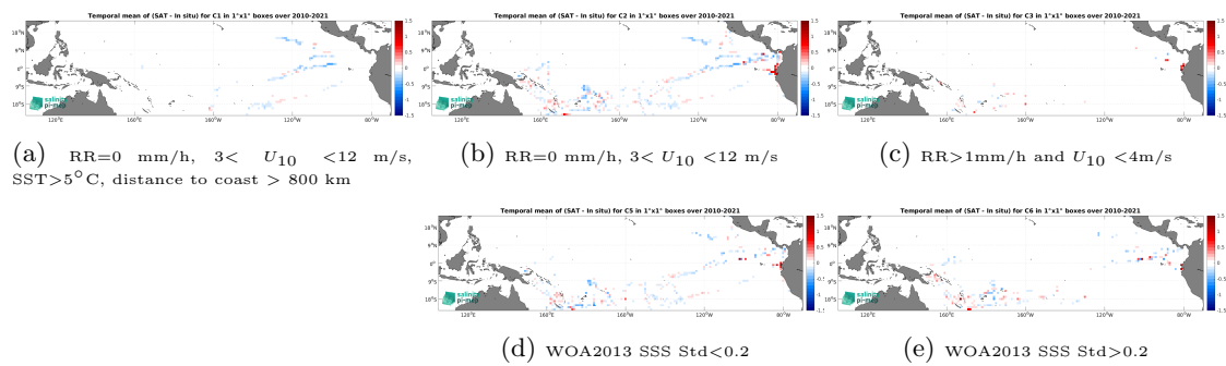
Figure 14: Temporal mean gridded over spatial boxes of size 1^\circ \times 1^\circ of \Delta SSS (CCI SSS L4 Merged-OI v4.41 - 7-day running (ESA) - TSG (GOSUD-Research-vessel)) for 5 different subdatasets corresponding to: RR=0 mm/h, 3 < U_{10} < 12 m/s, SST > 5^\circ\text{C} , distance to coast > 800 km (a), RR=0 mm/h, 3 < U_{10} < 12 m/s (b), RR > 1 mm/h and U_{10} < 4 m/s (c), WOA2013 SSS Std < 0.2 (d), WOA2013 SSS Std > 0.2 (e).
