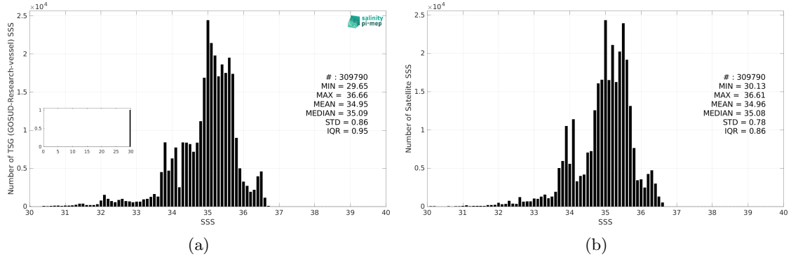
Figure 3: Histograms of SSS from TSG (GOSUD-Research-vessel) (a) and CCI SSS L4 Merged-OI v4.41 - 7-day running (ESA) (b) considering all match-up pairs per bins of 0.1 over the Tropical Pacific Ocean Pi-MEP region and for the full satellite product period.
