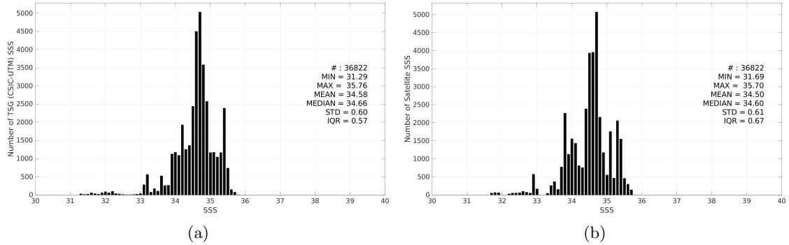
Figure 3: Histograms of SSS from TSG (CSIC-UTM) (a) and CCI SSS L4 Merged-OI v4.41 - 7-day running (ESA) (b) considering all match-up pairs per bins of 0.1 over the Tropical Pacific Ocean Pi-MEP region and for the full satellite product period.
