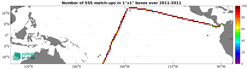
Figure 5: Number of SSS match-ups between TSG (CSIC-UTM) SSS and the CCI SSS L4 Merged-OI v4.41 - 7-day running (ESA) SSS product for the Tropical Pacific Ocean Pi-MEP region over 1^\circ \times 1^\circ boxes and for the full satellite product period.
