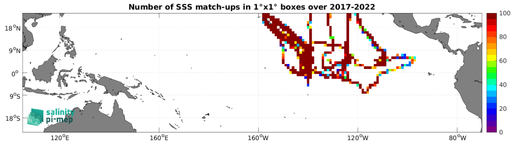
Figure 5: Number of SSS match-ups between Sailldrone SSS and the CCI SSS L4 Merged-OI v4.41 - 7-day running (ESA) SSS product for the Tropical Pacific Ocean Pi-MEP region over 1^\circ \times 1^\circ boxes and for the full satellite product period.
