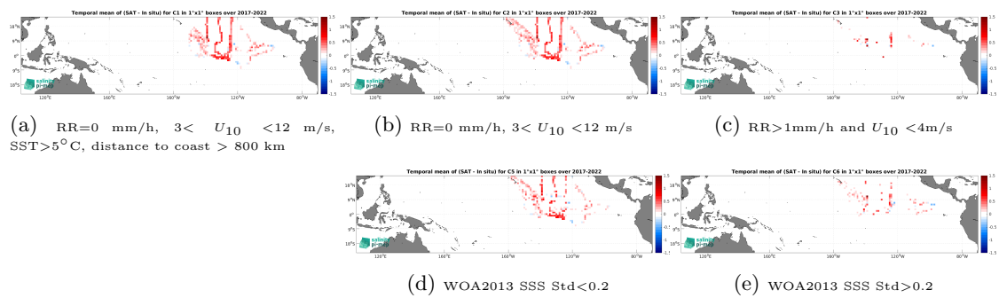
Figure 14: Temporal mean gridded over spatial boxes of size 1^\circ \times 1^\circ of \Delta SSS (CCI SSS L4 Merged-OI v4.41 - 7-day running (ESA) - Saildrone) for 5 different subdatasets corresponding to:RR=0 mm/h, 3 < U_{10} < 12 m/s, SST >5^\circ C, distance to coast > 800 km (a), RR=0 mm/h, 3 < U_{10} < 12 m/s (b), RR >1 mm/h and U_{10} < 4 m/s (c), WOA2013 SSS Std <0.2 (d), WOA2013 SSS Std >0.2 (e).
