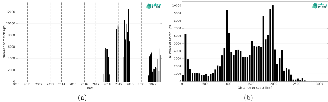
Figure 2: Number of match-ups between Saildrone and CCI SSS L4 Merged-OI v4.41 - 7-day running (ESA) SSS as a function of time (a) and as function of the distance to coast (b) over the Tropical Pacific Ocean Pi-MEP region and for the full satellite product period.
