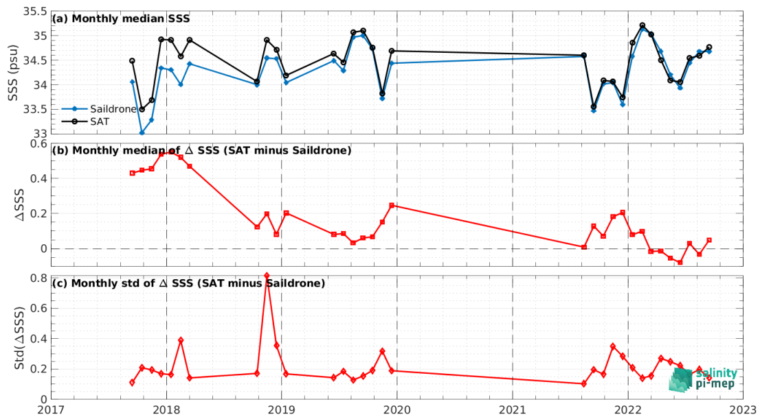
Figure 8: Time series of the monthly median SSS (top), median of \Delta SSS (Satellite - Sairdroner) and Std of \Delta SSS (Satellite - Sairdroner) over the Tropical Pacific Ocean Pi-MEP region considering all match-ups collected by the Pi-MEP.
