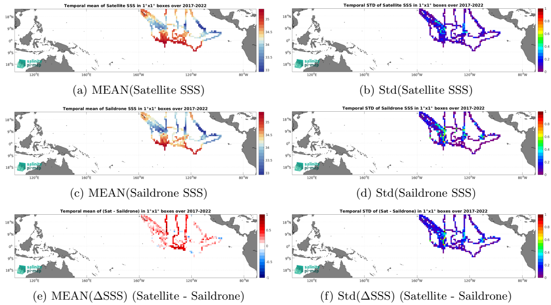
Figure 7: Temporal mean (left) and Std (right) of SSS from CCI SSS L4 Merged-OI v4.41 - 7-day running (ESA) (top), Saildrone (middle), and of \Delta SSS (Satellite - Saildrone). Only match-up pairs are used to generate these maps.
