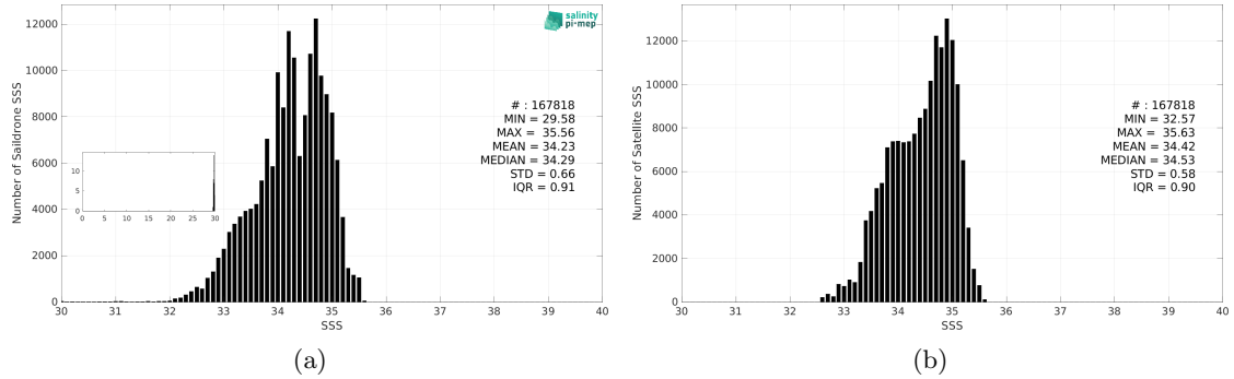
Figure 3: Histograms of SSS from Saildrone (a) and CCI SSS L4 Merged-OI v4.41 - 7-day running (ESA) (b) considering all match-up pairs per bins of 0.1 over the Tropical Pacific Ocean Pi-MEP region and for the full satellite product period.
