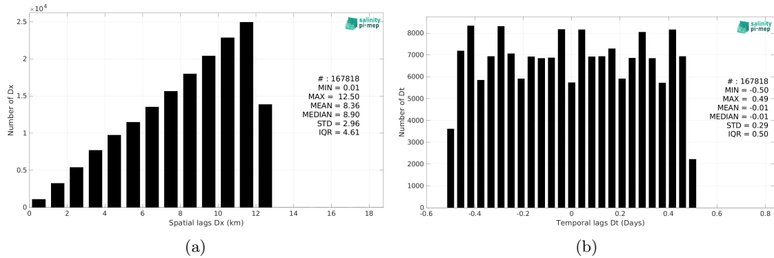
Figure 6: Histograms of the spatial (a) and temporal (b) lags between the location/time of the Sailldrone measurement and the date of the corresponding CCI SSS L4 Merged-OI v4.41 - 7-day running (ESA) SSS pixel.
