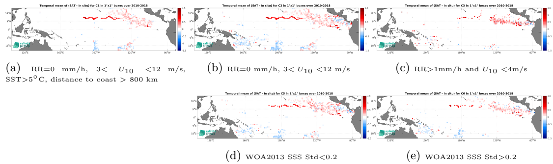
Figure 13: Temporal mean gridded over spatial boxes of size 1^\circ \times 1^\circ of \Delta SSS (CCI SSS L4 Merged-OI v4.41 - 7-day running (ESA) - Surface drifters) for 5 different subdatasets corresponding to: RR=0 mm/h, 3 < U_{10} < 12 m/s, SST > 5^\circ\text{C} , distance to coast > 800 km (a), RR=0 mm/h, 3 < U_{10} < 12 m/s (b), RR > 1 mm/h and U_{10} < 4 m/s (c), WOA2013 SSS Std < 0.2 (d), WOA2013 SSS Std > 0.2 (e).
