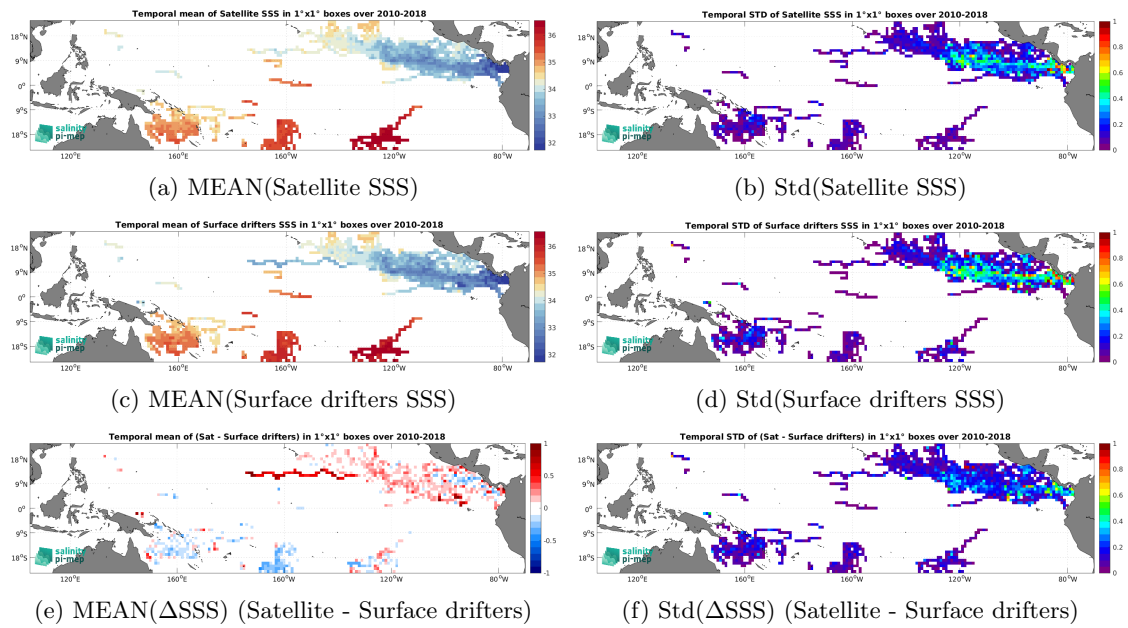
Figure 6: Temporal mean (left) and Std (right) of SSS from CCI SSS L4 Merged-OI v4.41 - 7-day running (ESA) (top), Surface drifters (middle), and of \Delta SSS (Satellite - Surface drifters). Only match-up pairs are used to generate these maps.
