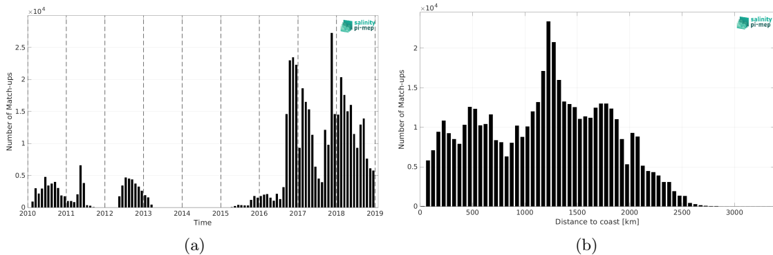
Figure 2: Number of match-ups between Surface drifters and CCI SSS L4 Merged-OI v4.41 - 7-day running (ESA) SSS as a function of time (a) and as function of the distance to coast (b) over the Tropical Pacific Ocean Pi-MEP region and for the full satellite product period.
