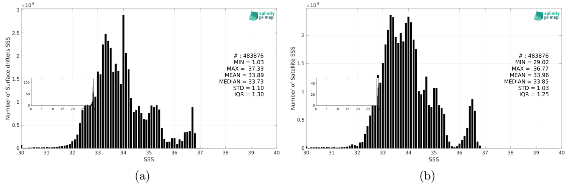
Figure 3: Histograms of SSS from Surface drifters (a) and CCI SSS L4 Merged-OI v4.41 - 7-day running (ESA) (b) considering all match-up pairs per bins of 0.1 over the Tropical Pacific Ocean Pi-MEP region and for the full satellite product period.
