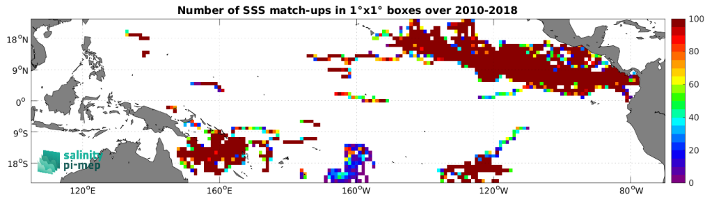
Figure 4: Number of SSS match-ups between Surface drifters SSS and the CCI SSS L4 Merged-OI v4.41 - 7-day running (ESA) SSS product for the Tropical Pacific Ocean Pi-MEP region over 1^\circ \times 1^\circ boxes and for the full satellite product period.
