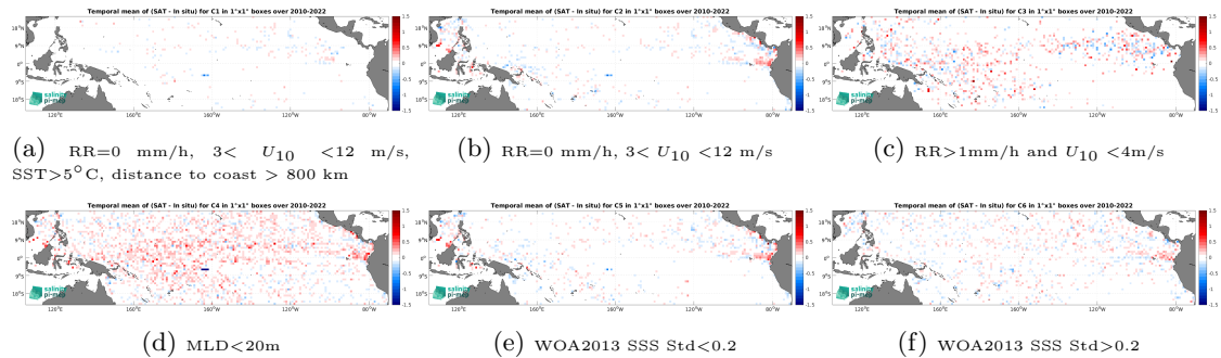
Figure 14: Temporal mean gridded over spatial boxes of size 1^\circ \times 1^\circ of \Delta SSS (CCI SSS L4 Merged-OI v4.41 - 7-day running (ESA) - Argo) for 6 different subdatasets corresponding to:RR=0 mm/h, 3 < U_{10} < 12 m/s, SST >5^\circ C, distance to coast > 800 km (a), RR=0 mm/h, 3 < U_{10} < 12 m/s (b), RR >1 mm/h and U_{10} < 4 m/s (c),MLD <20 m (d),WOA2013 SSS Std <0.2 (e),WOA2013 SSS Std >0.2 (f).
