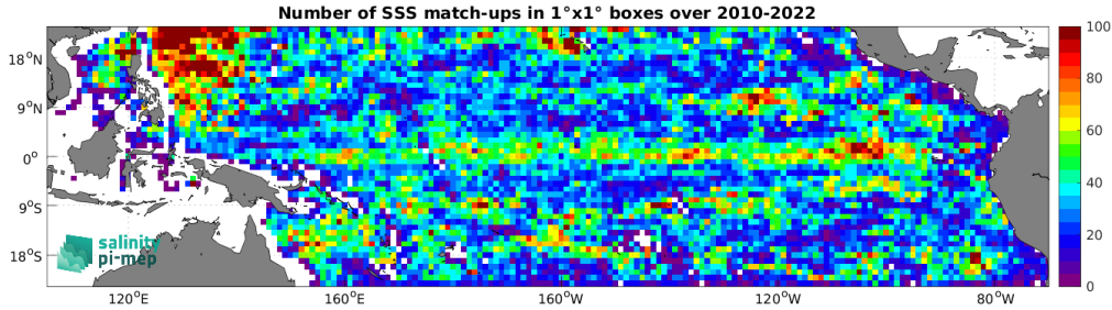
Figure 5: Number of SSS match-ups between Argo SSS and the CCI SSS L4 Merged-OI v4.41 - 7-day running (ESA) SSS product for the Tropical Pacific Ocean Pi-MEP region over 1^\circ \times 1^\circ boxes and for the full satellite product period.
