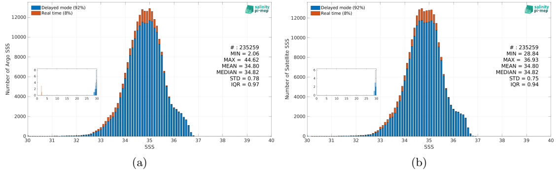
Figure 3: Histograms of SSS from Argo (a) and CCI SSS L4 Merged-OI v4.41 - 7-day running (ESA) (b) considering all match-up pairs per bins of 0.1 over the Tropical Pacific Ocean Pi-MEP region and for the full satellite product period.
