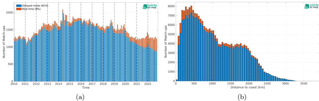
Figure 2: Number of match-ups between Argo and CCI SSS L4 Merged-OI v4.41 - 7-day running (ESA) SSS as a function of time (a) and as function of the distance to coast (b) over the Tropical Pacific Ocean Pi-MEP region and for the full satellite product period.
