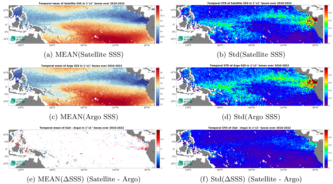
Figure 7: Temporal mean (left) and Std (right) of SSS from CCI SSS L4 Merged-OI v4.41 - 7-day running (ESA) (top), Argo (middle), and of \Delta SSS (Satellite - Argo). Only match-up pairs are used to generate these maps.
